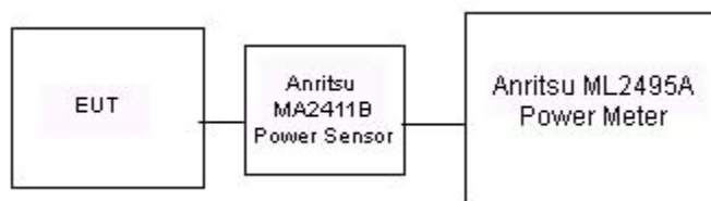
Figure 9-5 Power Measurement Setup for Bandwidths < 50 MHz
