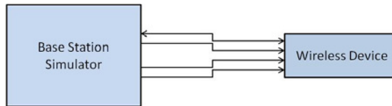
Figure I-4 Power Measurement Setup
