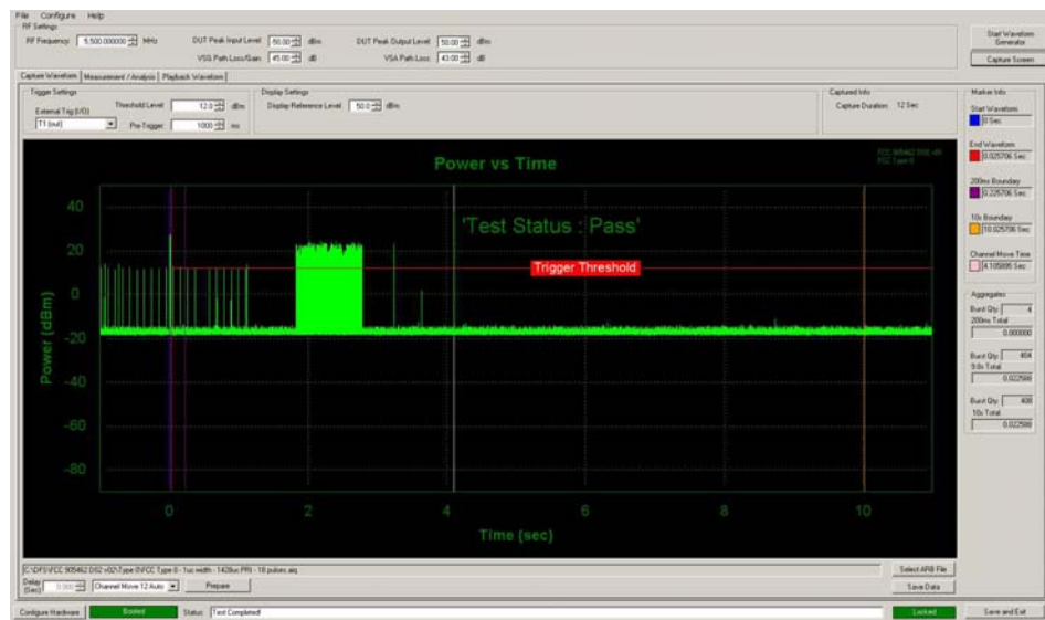
Figure 5-4. Band 2C Move Time and Aggregate Time
