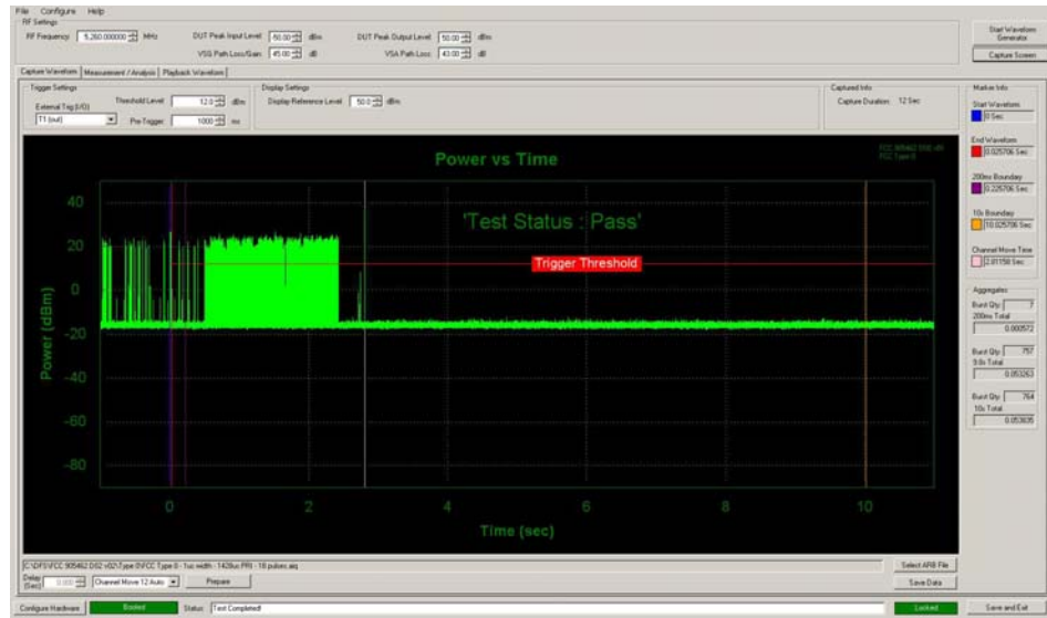
Figure 5-3. Band 2A Move Time and Aggregate Time
