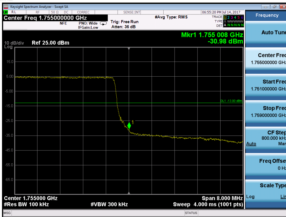
Plot 7-211. Upper Band Edge Plot (Band 4 - 10.0MHz QPSK - RB Size 50)
