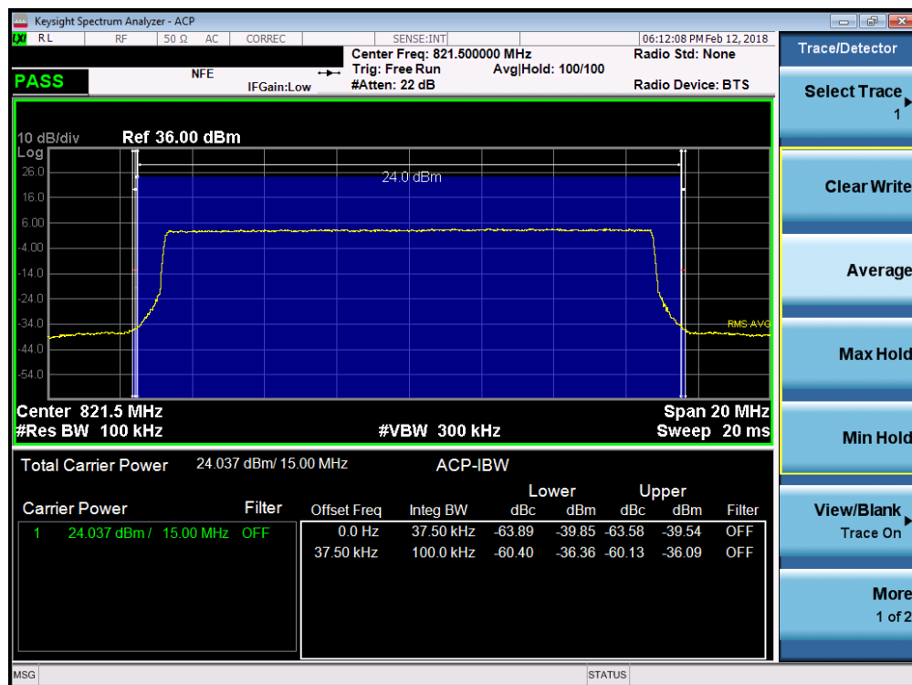
Plot 7-32. Channel Edge Plot (15MHz QPSK – RB Size 75)
