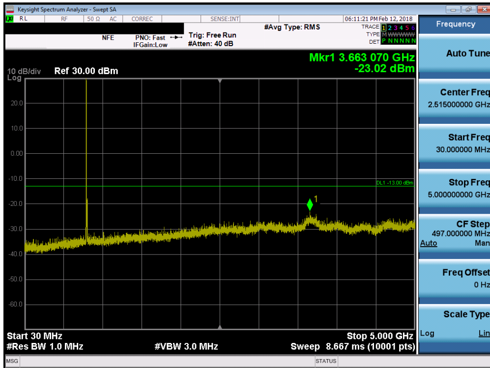
Plot 7-21. Conducted Spurious Plot (15MHz QPSK – RB Size 1, RB Offset 0 – Low Channel)
