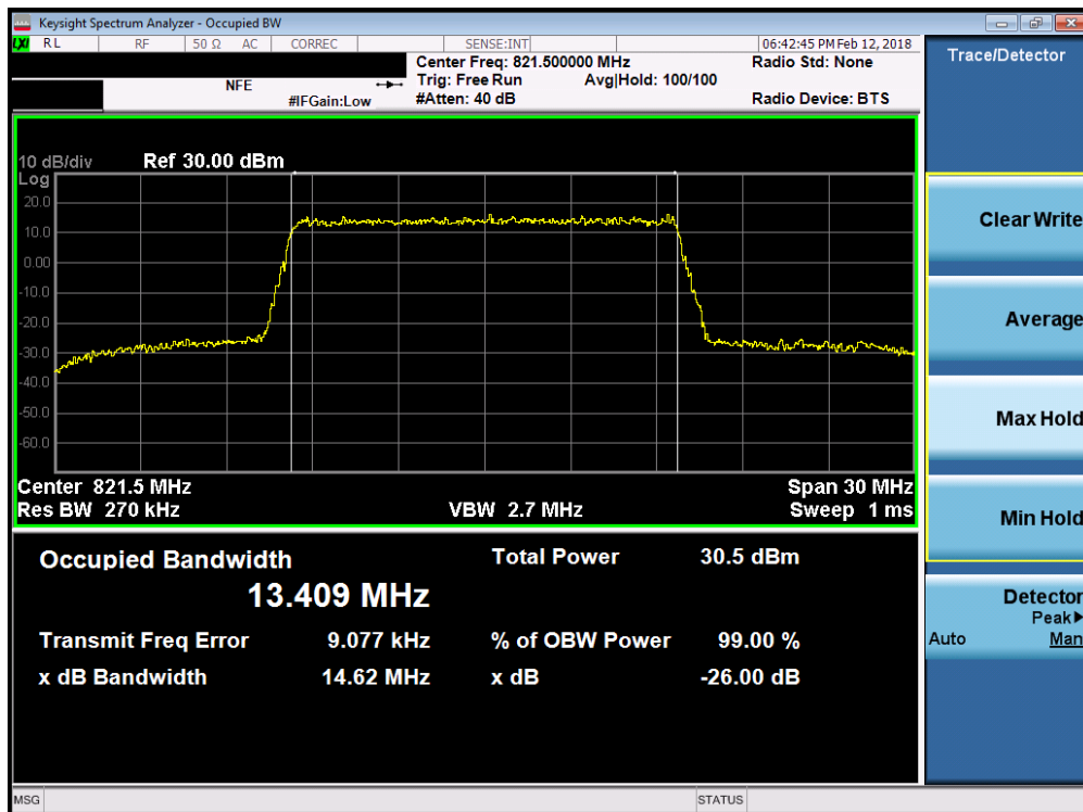
Plot 7-16. Occupied Bandwidth Plot (15MHz 64-QAM – RB Size 75)
