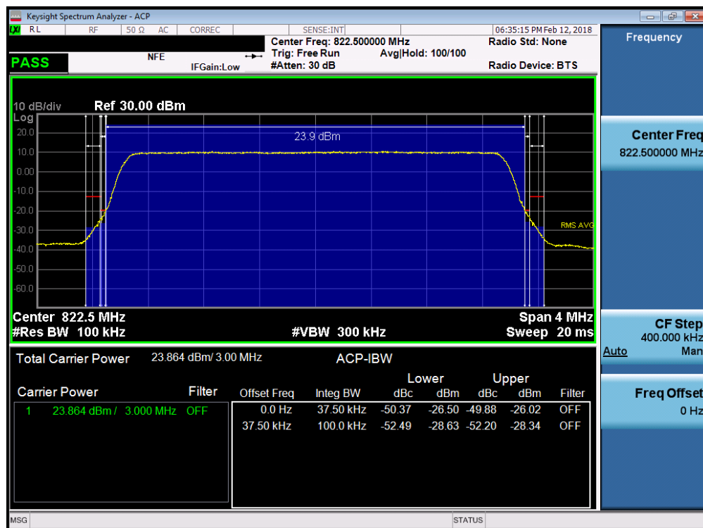
Plot 7-28. Channel Edge Plot (3MHz QPSK – RB Size 15 – High Channel)
