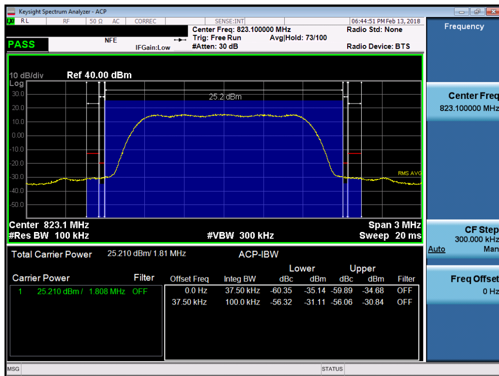
Plot 7-24. Channel Edge Plot (Ch. 684)
