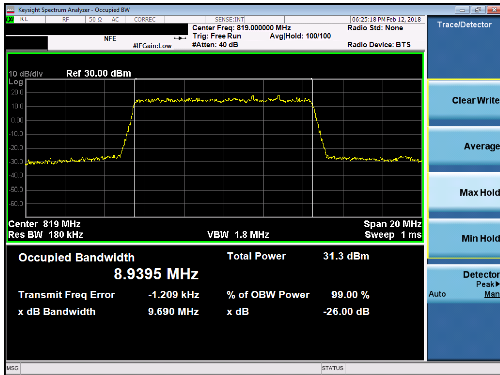
Plot 7-12. Occupied Bandwidth Plot (10MHz 16-QAM – RB Size 50)
