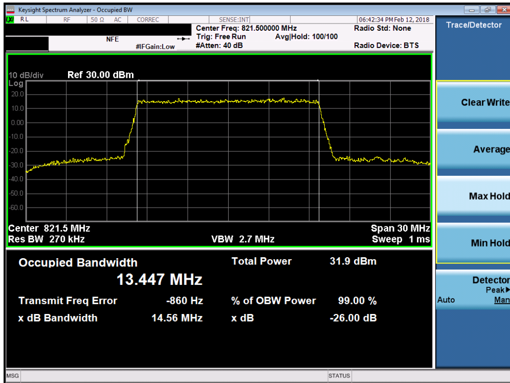
Plot 7-15. Occupied Bandwidth Plot (15MHz 16-QAM – RB Size 75)
