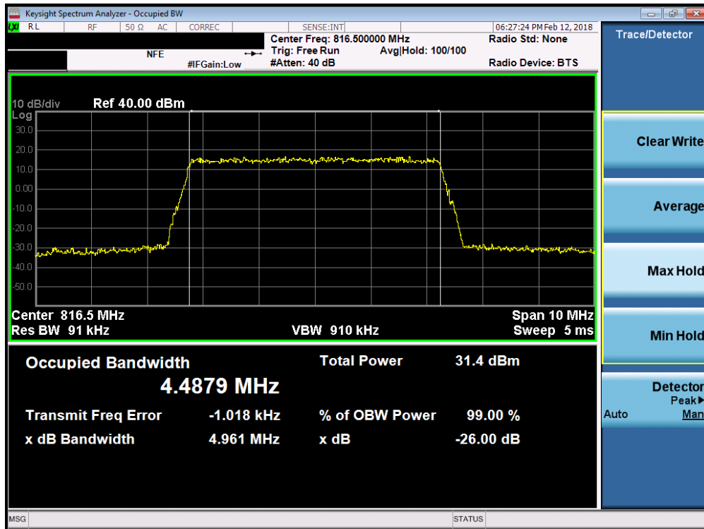
Plot 7-9. Occupied Bandwidth Plot (5MHz 16-QAM – RB Size 25– Low Channel)
