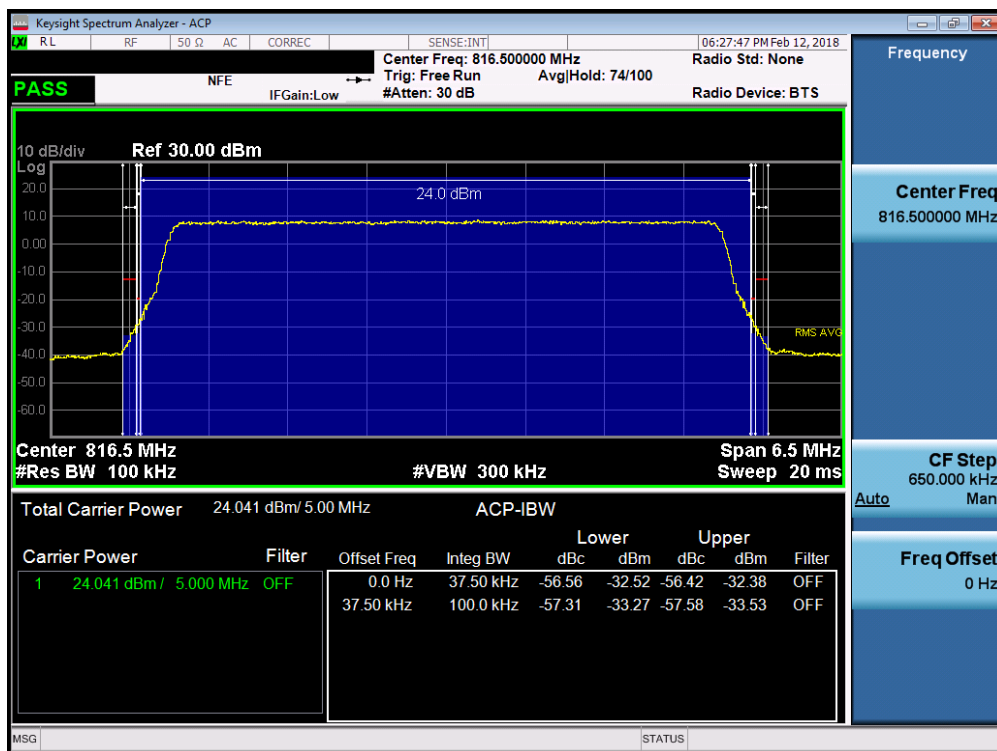
Plot 7-29. Channel Edge Plot (5MHz QPSK – RB Size 25– Low Channel)
