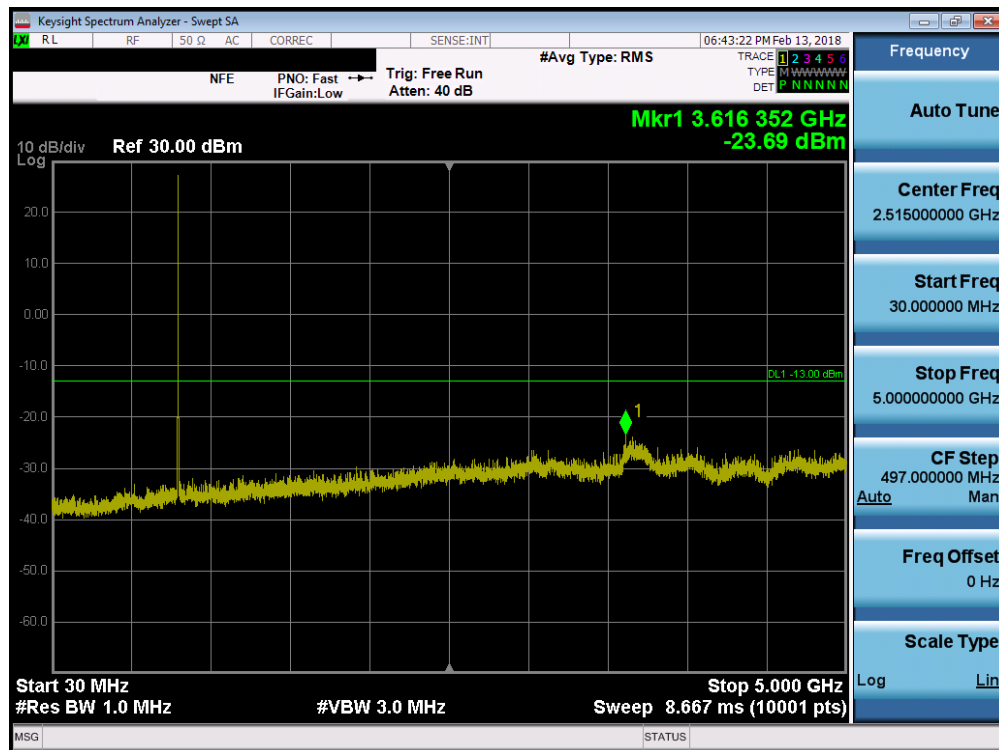
Plot 7-17. Conducted Spurious Plot (Ch. 476)
