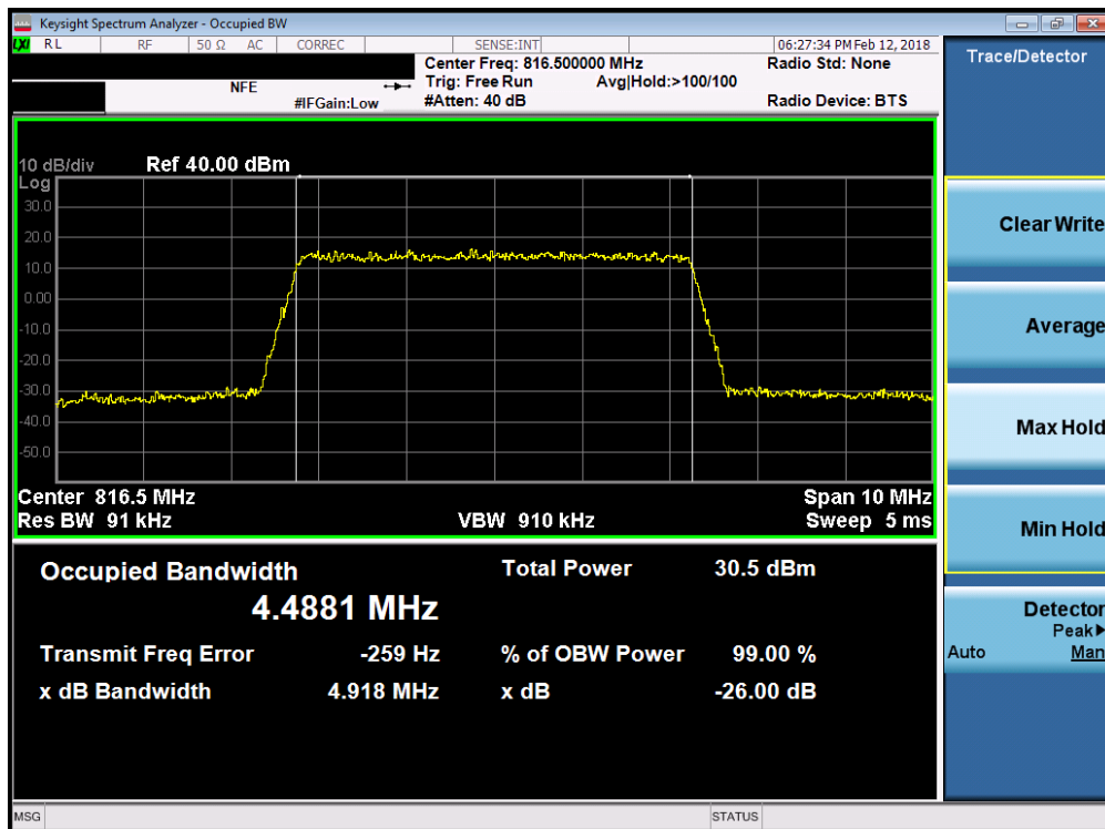
Plot 7-10. Occupied Bandwidth Plot (5MHz 64-QAM – RB Size 25– Low Channel)
