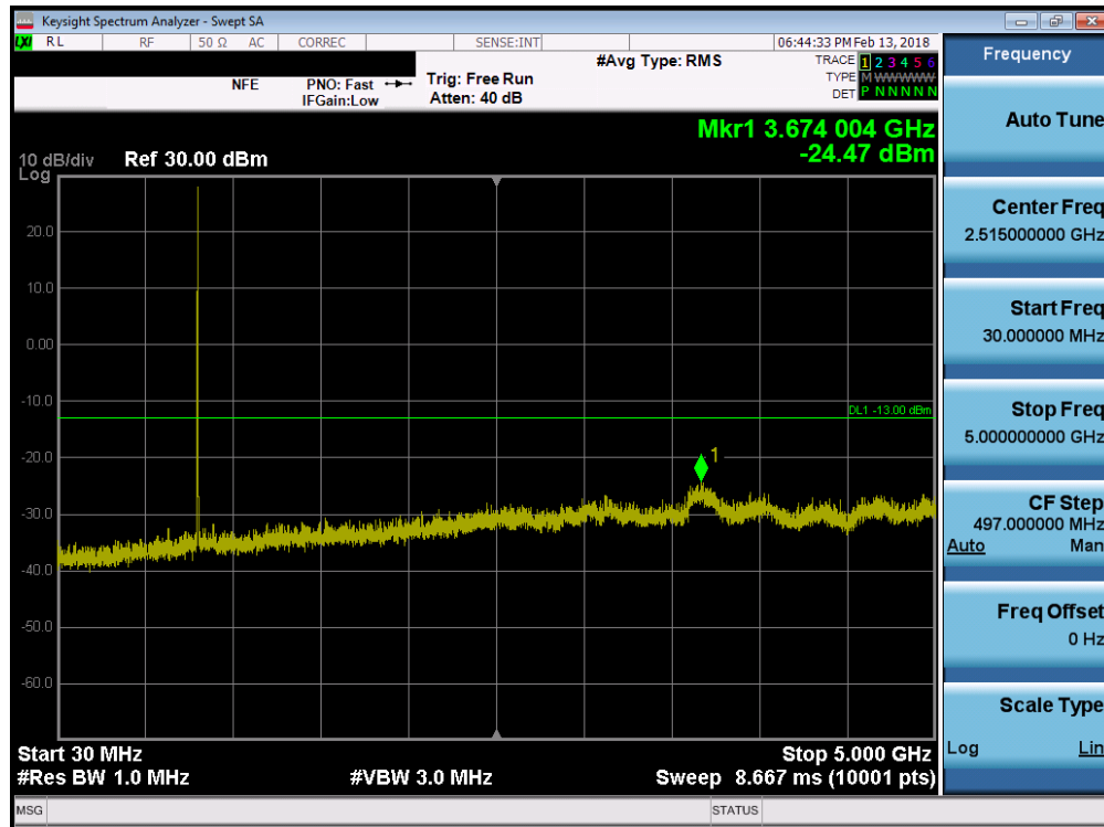
Plot 7-19. Conducted Spurious Plot (Ch. 684)
