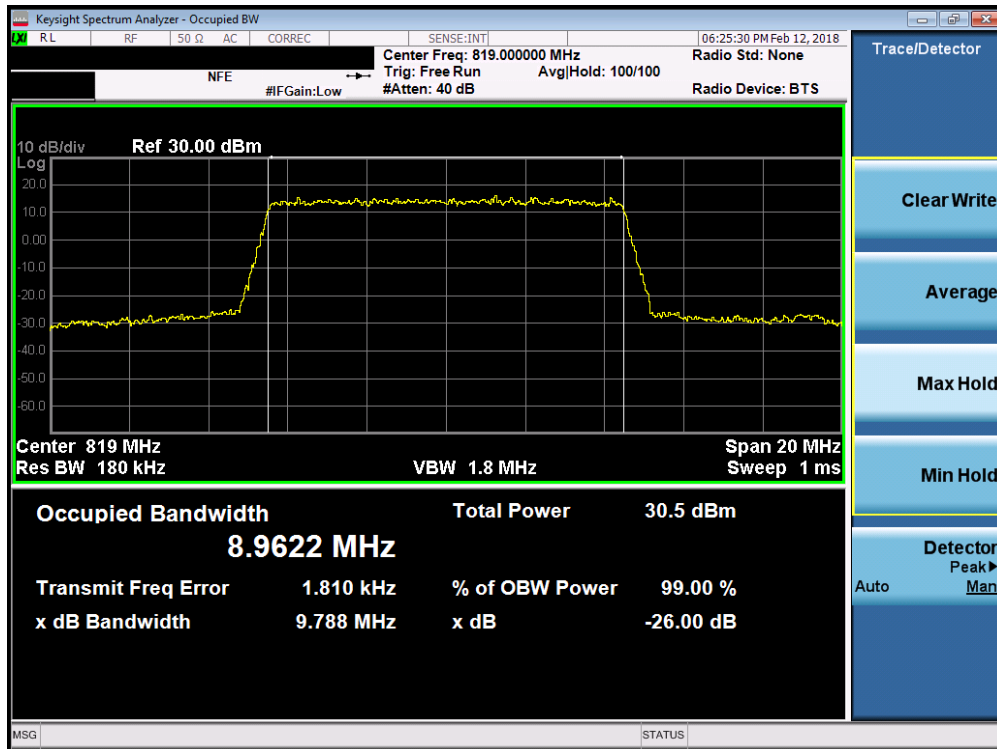
Plot 7-13. Occupied Bandwidth Plot (10MHz 64-QAM – RB Size 50)
