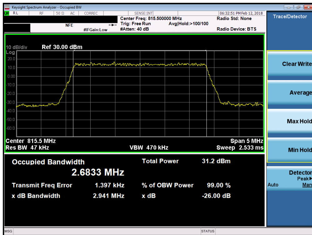
Plot 7-7. Occupied Bandwidth Plot (3MHz 64-QAM – RB Size 15– Low Channel)
