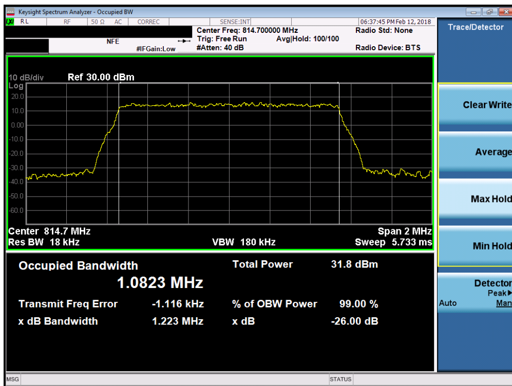
Plot 7-2. Occupied Bandwidth Plot (1.4MHz QPSK – RB Size 6– Low Channel)
