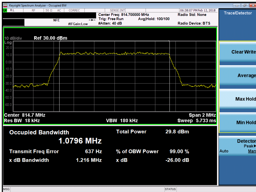
Plot 7-4. Occupied Bandwidth Plot (1.4MHz 64-QAM – RB Size 6– Low Channel)
