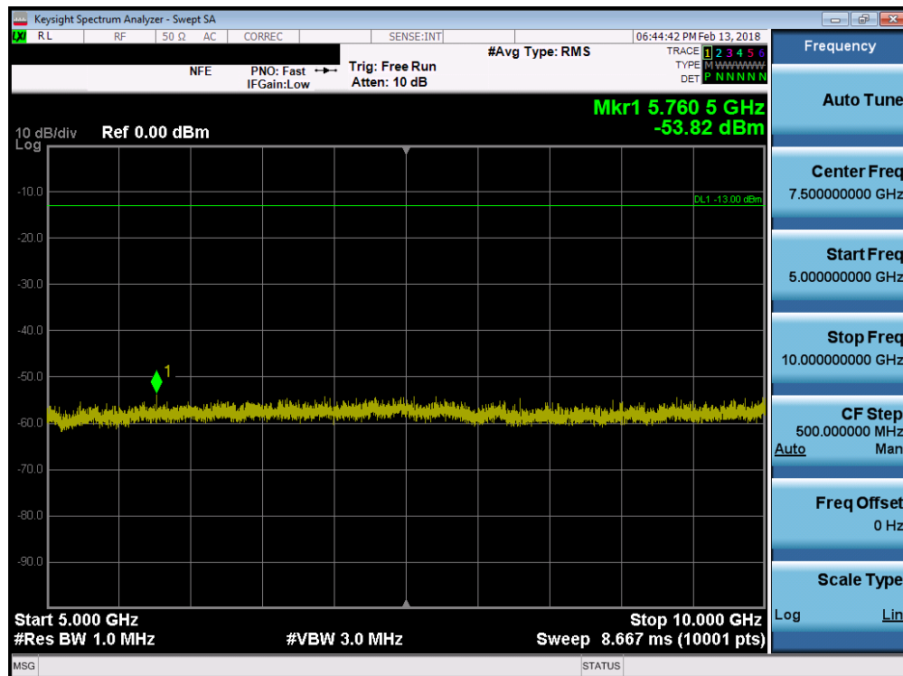
Plot 7-20. Conducted Spurious Plot (Ch. 684)
