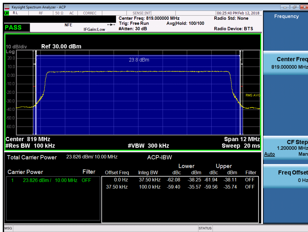
Plot 7-31. Channel Edge Plot (10MHz QPSK – RB Size 50)
