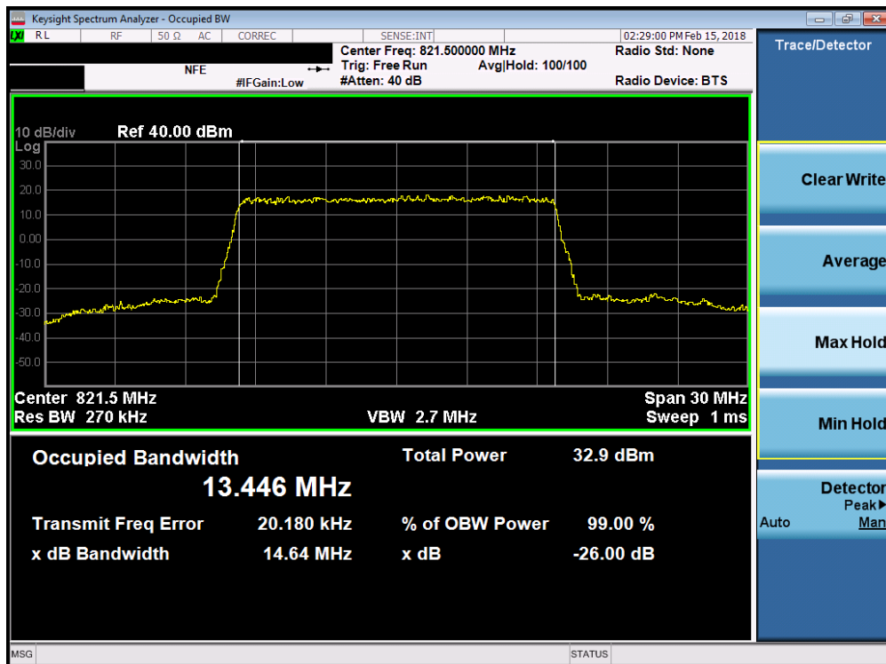
Plot 7-14. Occupied Bandwidth Plot (15MHz QPSK – RB Size 75)
