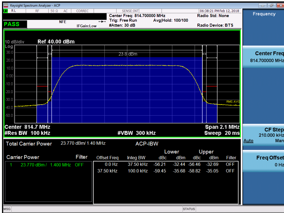
Plot 7-25. Channel Edge Plot (1.4MHz QPSK – RB Size 6– Low Channel)
