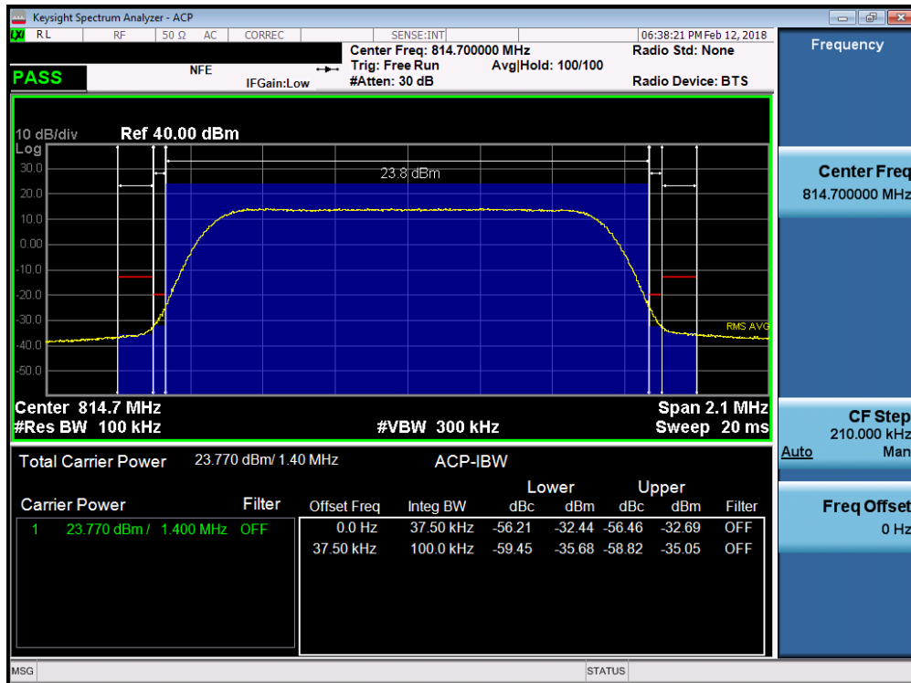
Plot 7-26. Channel Edge Plot (1.4MHz QPSK – RB Size 6 – High Channel)
