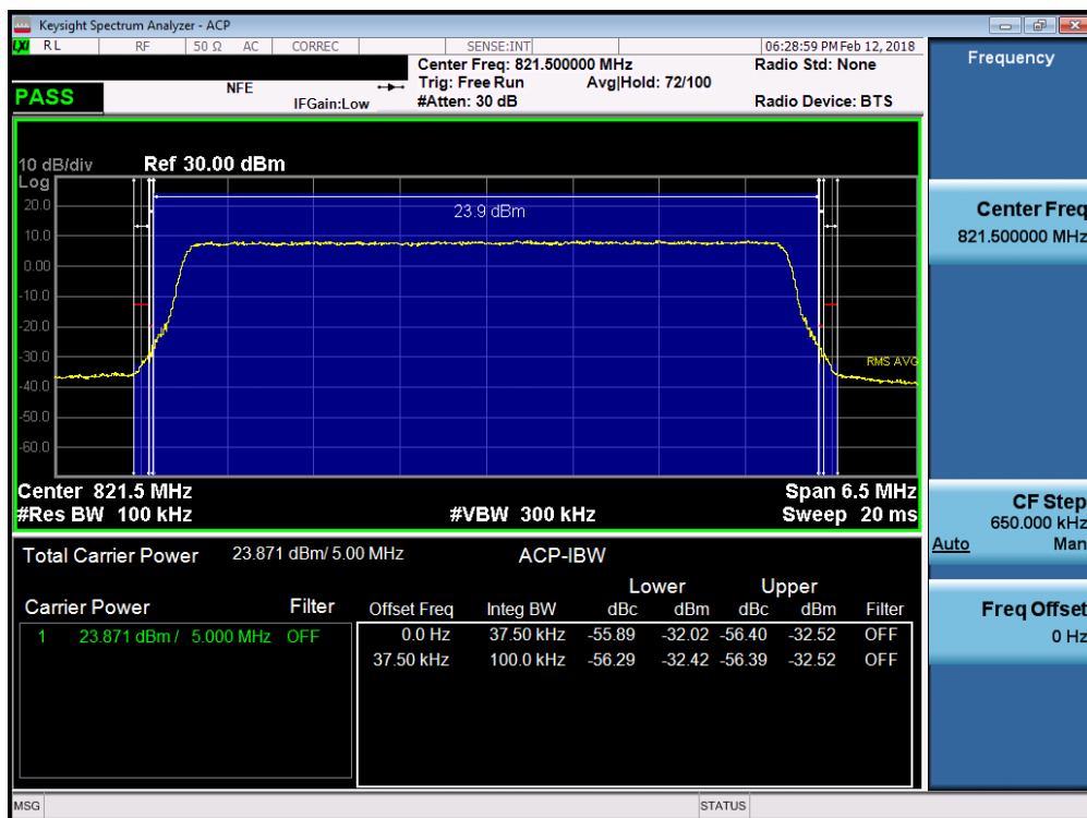
Plot 7-30. Channel Edge Plot (5MHz QPSK – RB Size 25 – High Channel)
