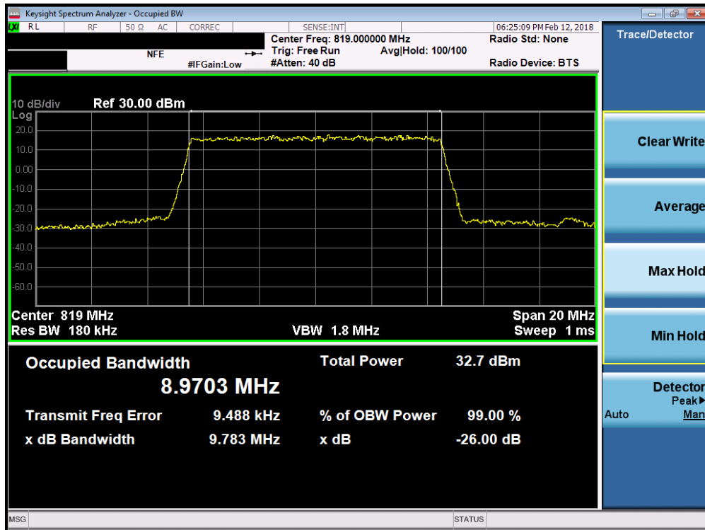
Plot 7-11. Occupied Bandwidth Plot (10MHz QPSK – RB Size 50)
