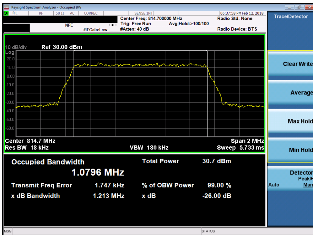
Plot 7-3. Occupied Bandwidth Plot (1.4MHz 16-QAM – RB Size 6– Low Channel)
