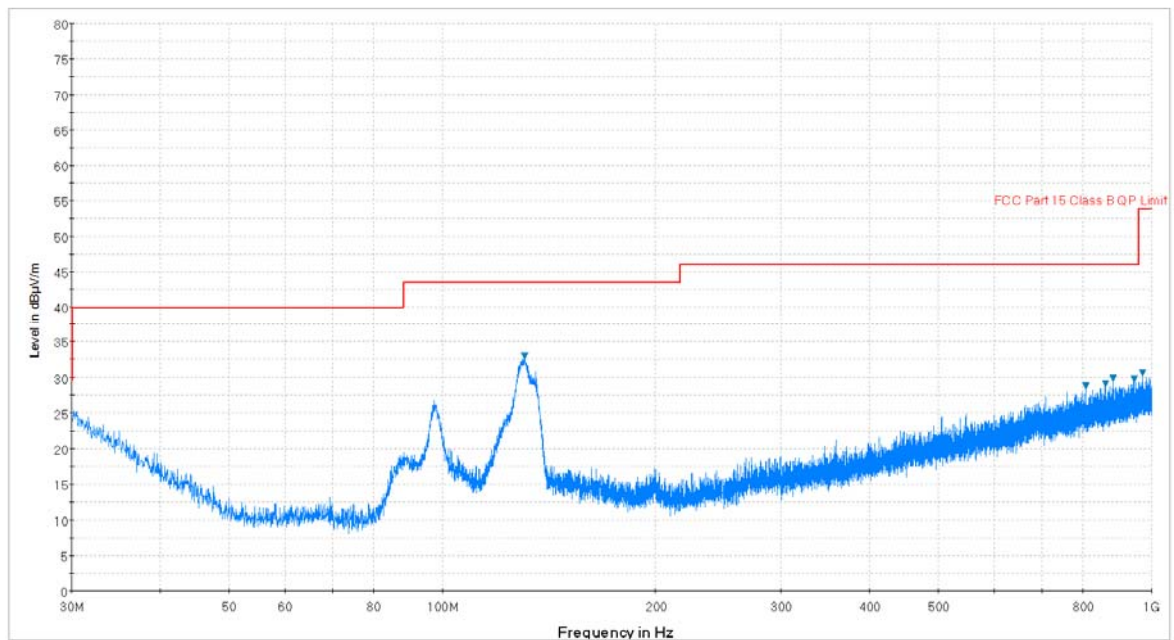
Plot 7-55. Radiated Spurious Plot below 1GHz (Pol. V)
