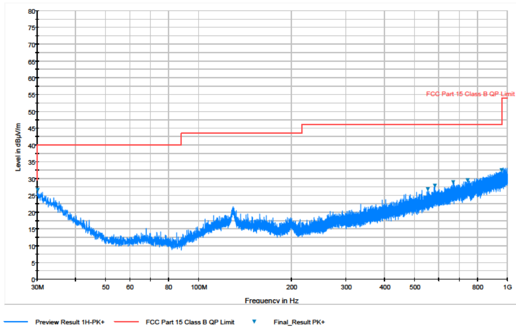
Plot 7-1. Radiated Spurious Plot 30MHz – 1GHz (Pol. H)
