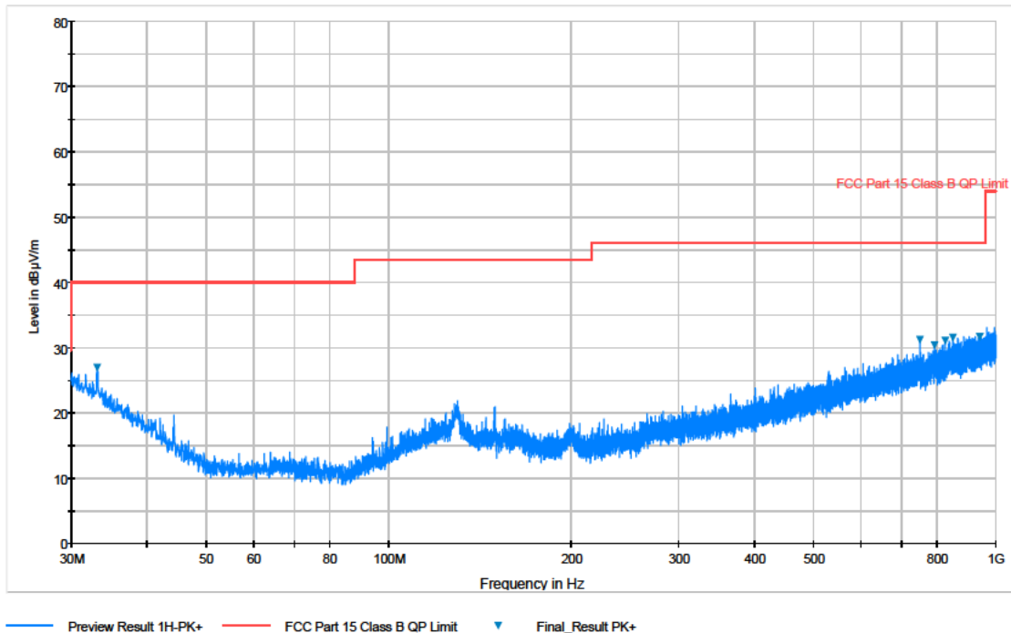
Plot 7-2. Radiated Spurious Plot 30MHz – 1GHz (Pol. V)
