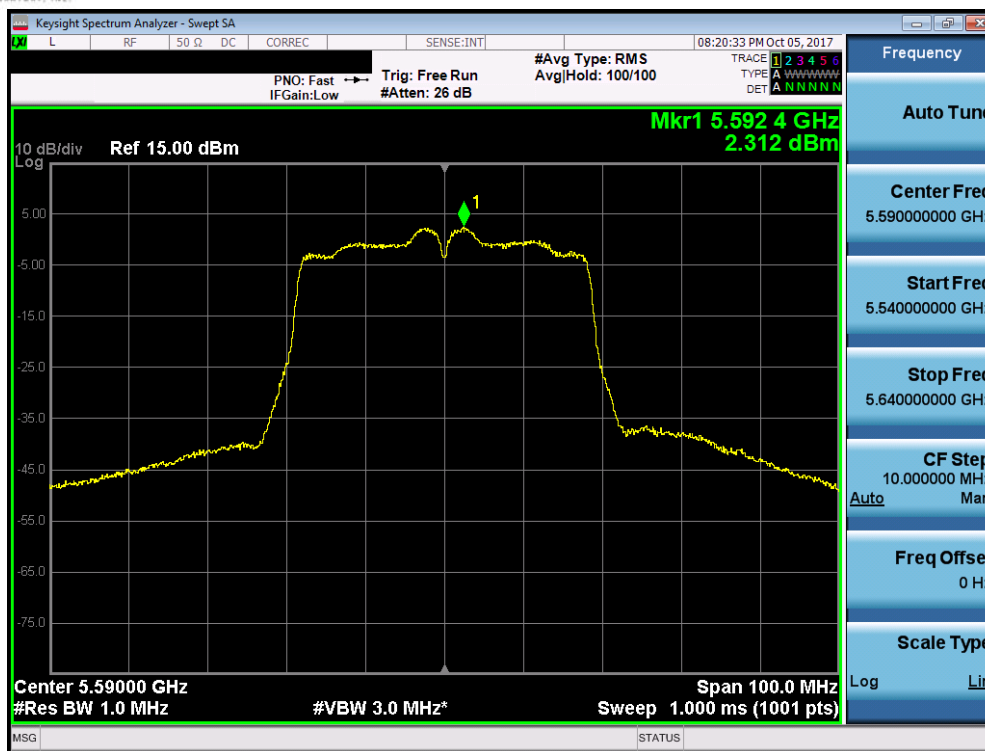
Plot 7-15. Power Spectral Density Plot (40MHz BW 802.11n (UNII Band 2C) – Ch. 118)
