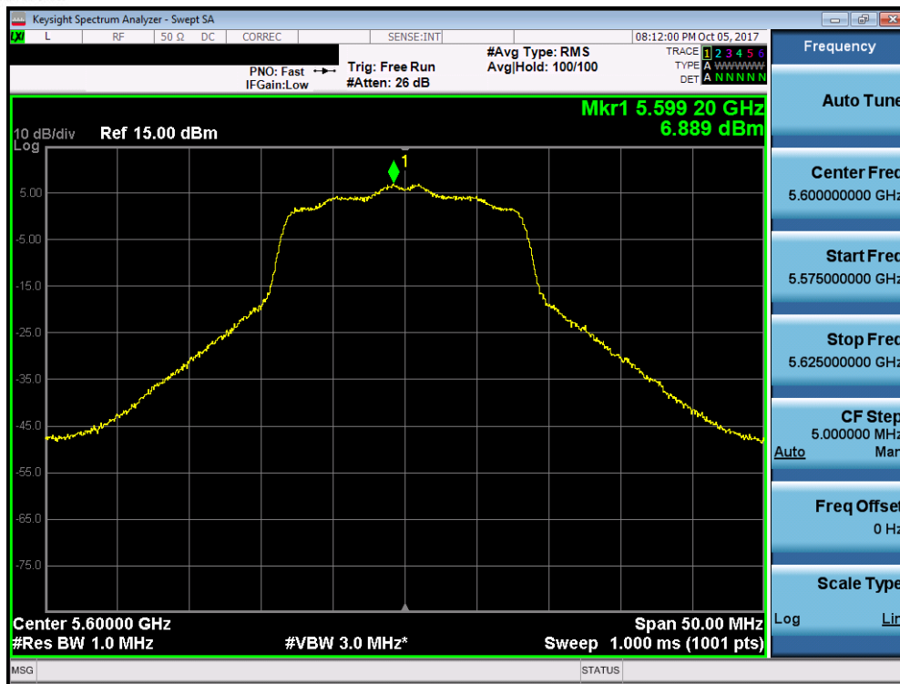
Plot 7-9. Power Spectral Density Plot (802.11a (UNII Band 2C) – Ch. 120)
