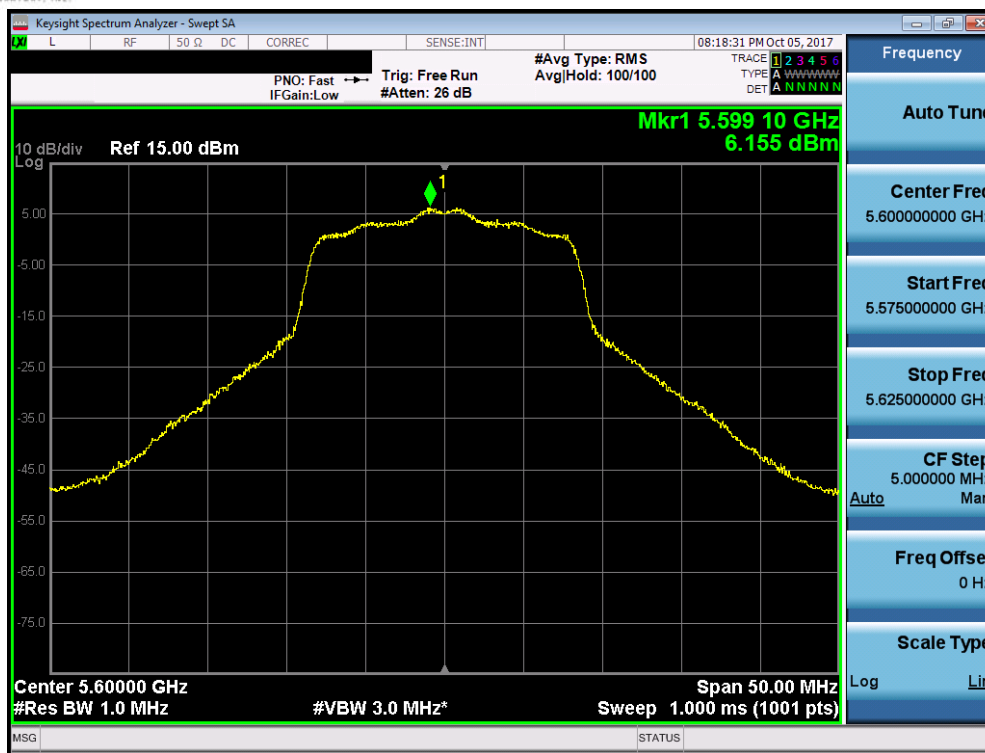
Plot 7-13. Power Spectral Density Plot (802.11a (UNII Band 2C) – Ch. 120)
