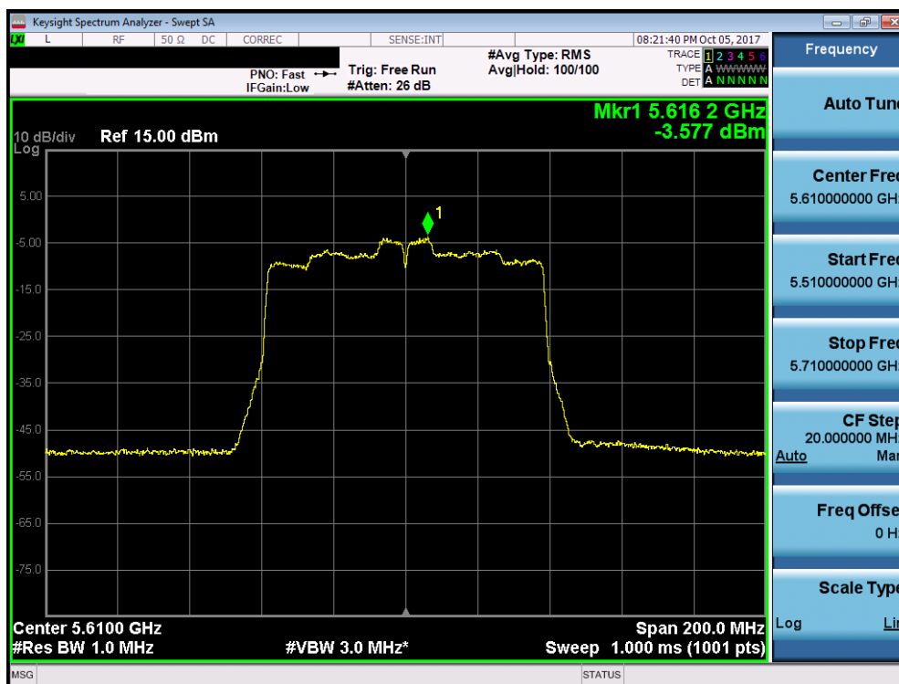
Plot 7-16. Power Spectral Density Plot (80MHz BW 802.11ac (UNII Band 2C) – Ch. 122)
