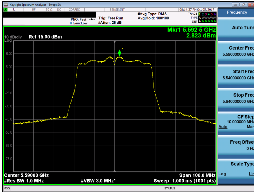
Plot 7-11. Power Spectral Density Plot (40MHz BW 802.11n (UNII Band 2C) – Ch. 118)
