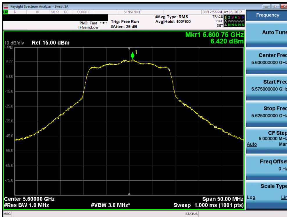
Plot 7-10. Power Spectral Density Plot (20MHz BW 802.11n (UNII Band 2C) – Ch. 120)
