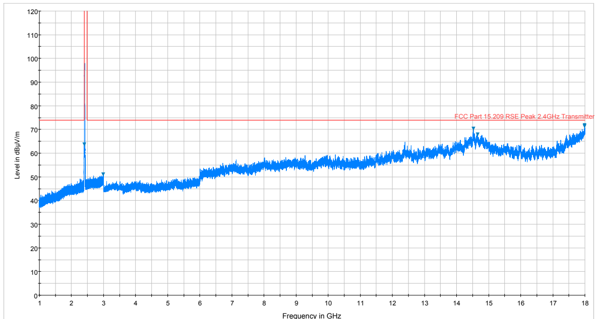
Plot 7-62. Radiated Spurious Plot above 1GHz (802.11b – Ch. 1, Ant. Pol. V)
