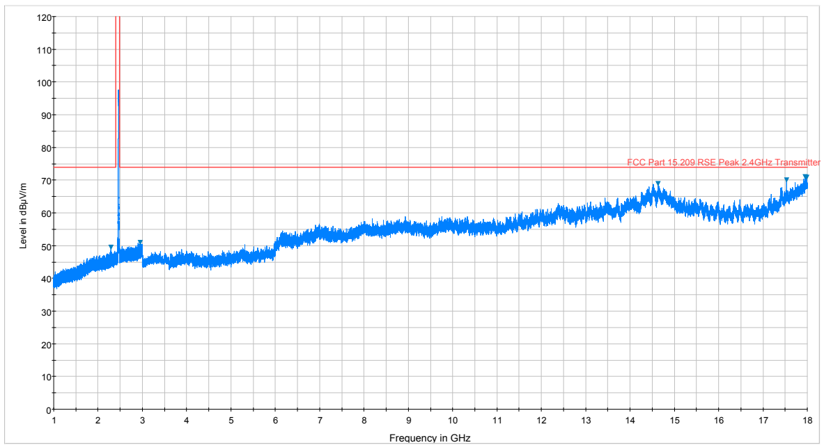
Plot 7-66. Radiated Spurious Plot above 1GHz (802.11b – Ch. 11, Ant. Pol. V)
