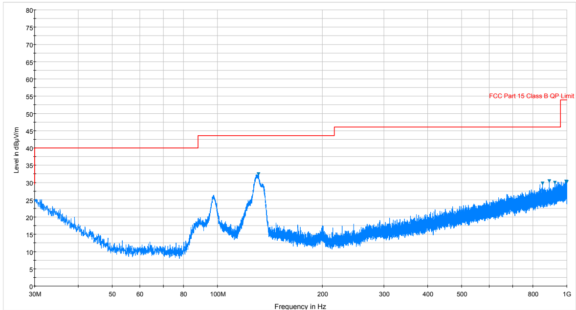
Plot 7-91. Radiated Spurious Plot below 1GHz (Pol. H)
