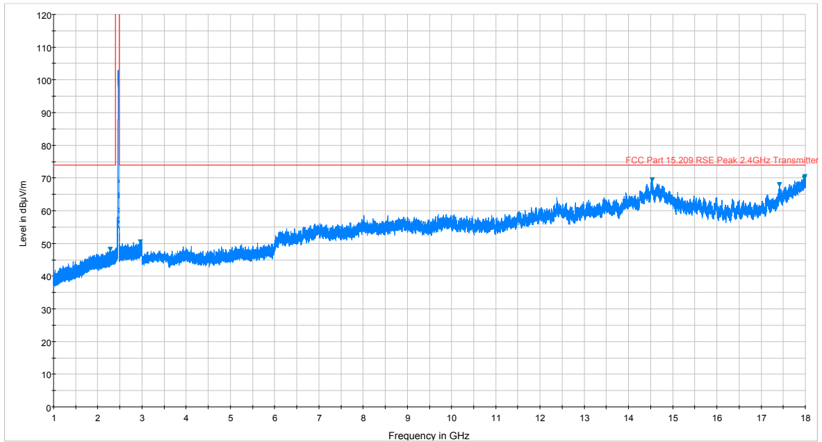
Plot 7-65. Radiated Spurious Plot above 1GHz (802.11b – Ch. 11, Ant. Pol. H)
