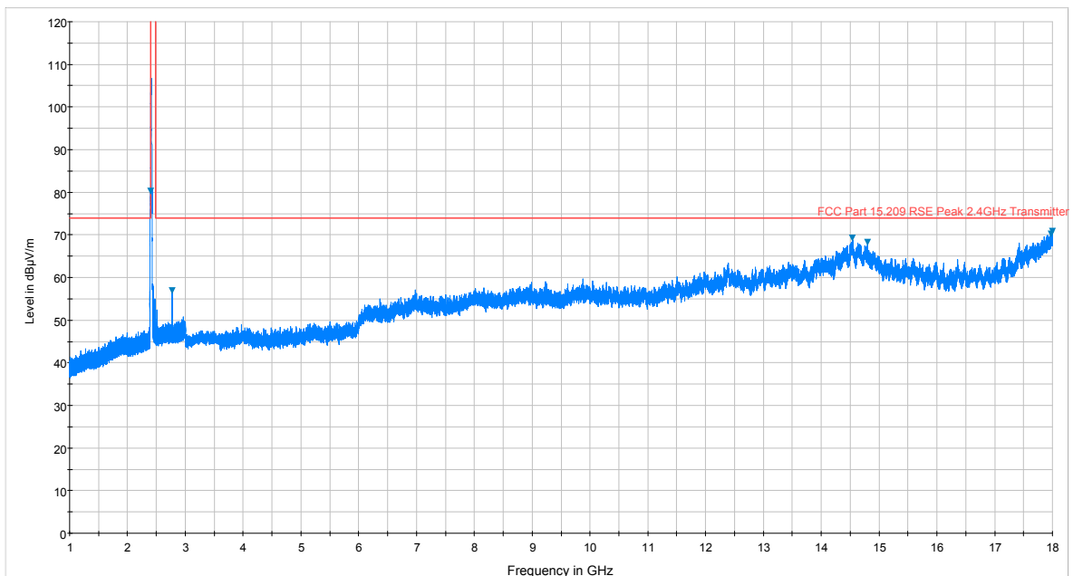
Plot 7-70. Radiated Spurious Plot above 1GHz (802.11b – Ch. 1, Ant. Pol. V)
