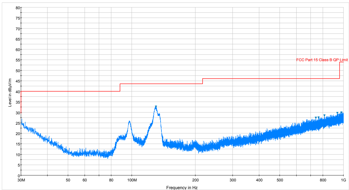
Plot 7-90. Radiated Spurious Plot below 1GHz (Pol. V)
