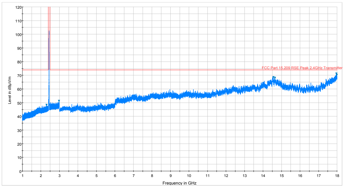
Plot 7-64. Radiated Spurious Plot above 1GHz (802.11b – Ch. 6, Ant. Pol. V)
