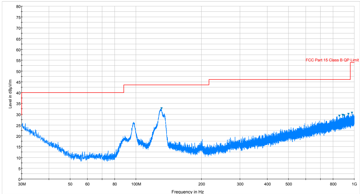
Plot 7-89. Radiated Spurious Plot below 1GHz (Pol. H)
