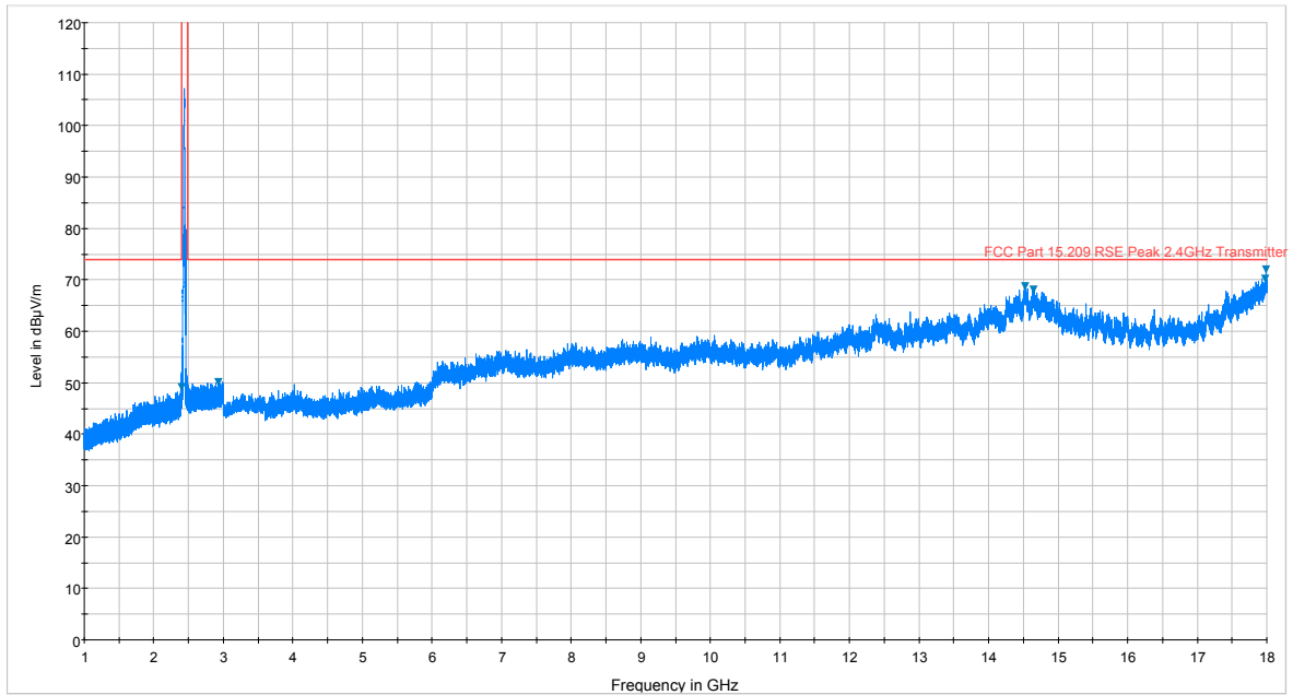
Plot 7-71. Radiated Spurious Plot above 1GHz (802.11b – Ch. 6, Ant. Pol. H)
