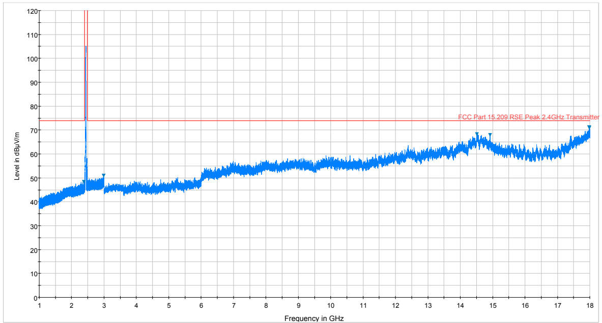
Plot 7-63. Radiated Spurious Plot above 1GHz (802.11b – Ch. 6, Ant. Pol. H)
