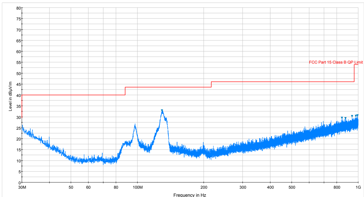
Plot 7-92. Radiated Spurious Plot below 1GHz (Pol. V)
