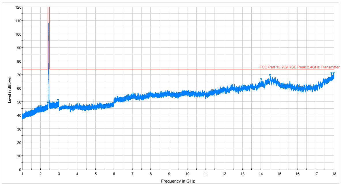
Plot 7-72. Radiated Spurious Plot above 1GHz (802.11b – Ch. 6, Ant. Pol. V)
