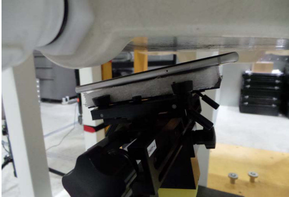
SAR Test Setup Photo 5: Mouth-Jaw Replacing Left Tilt
