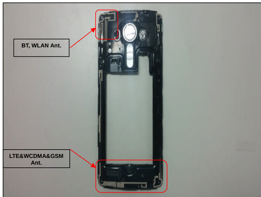
View of WLAN, BT, NFC, GSM&WCDMA&LTE Antenna
