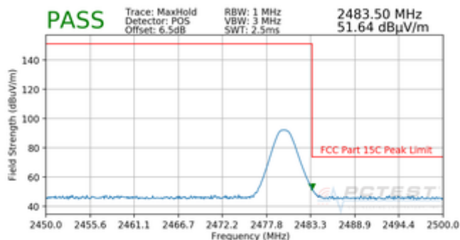
Plot 7-36. Radiated Restricted Upper Band Edge Measurement (Peak) with WCP
