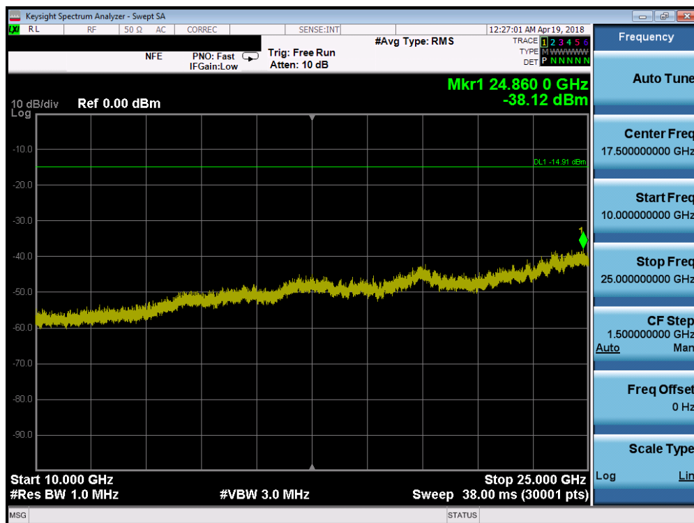
Plot 7-30. Conducted Spurious Plot (Bluetooth (LE), 2Mbps – Ch. 19)
