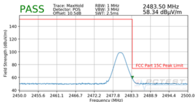
Plot 7-34. Radiated Restricted Upper Band Edge Measurement (Peak)
