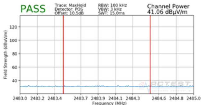
Plot 7-35. Radiated Restricted Upper Band Edge Measurement (Average) with WCP
