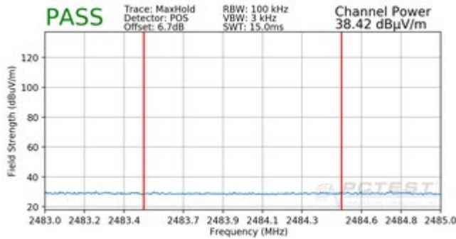
Plot 7-1. Radiated Restricted Upper Band Edge Measurement (Average & Peak)
