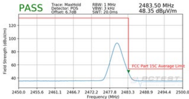
Plot 7-2. Radiated Restricted Upper Band Edge Measurement with WCP (Average & Peak)
