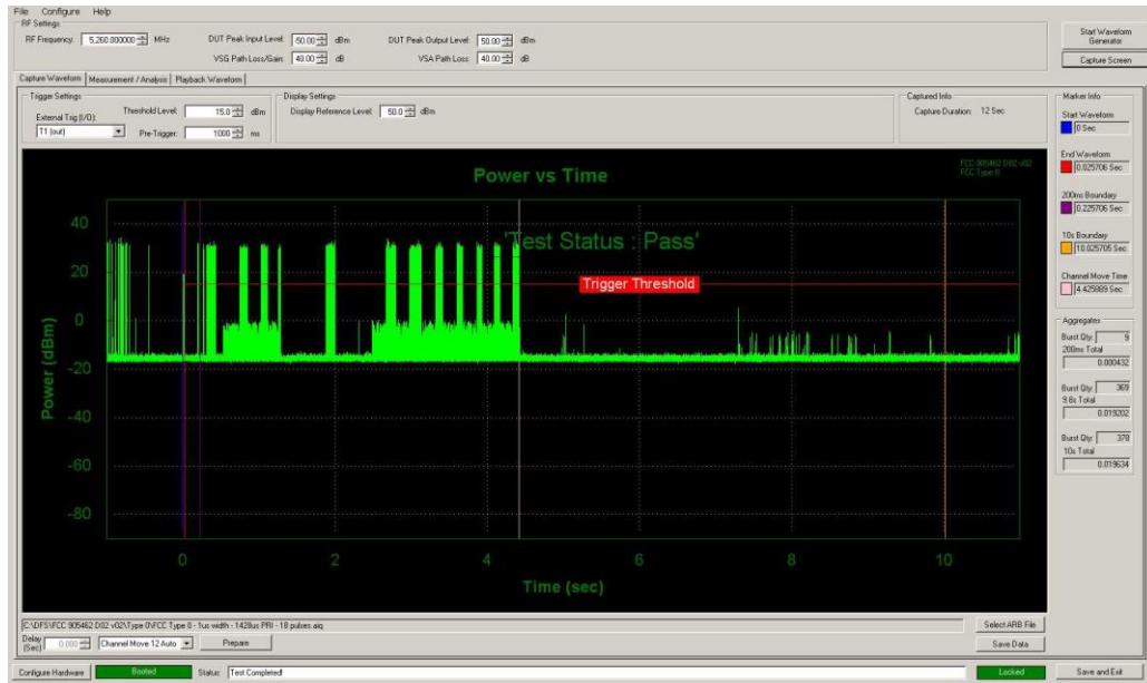
Figure 5-3. Band 2A Move Time and Aggregate Time
