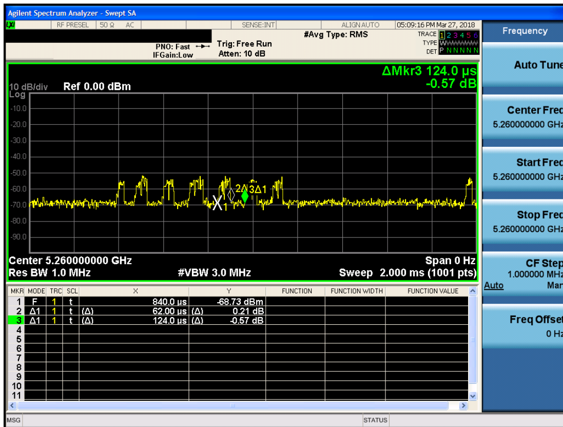
Figure 5-1. Band 2A Pulse Width and Period
