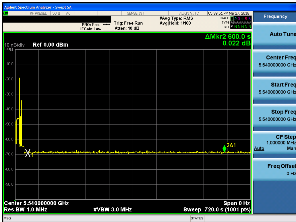
Figure 5-5. Band 2C Client Beacon Test – Monitoring live spectrum – Elapse time 10 minutes
