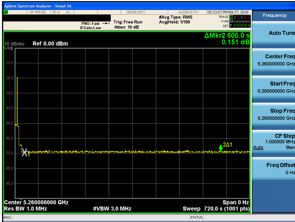
Figure 5-4. Band 2A Client Beacon Test – Monitoring live spectrum – Elapse time 10 minutes
