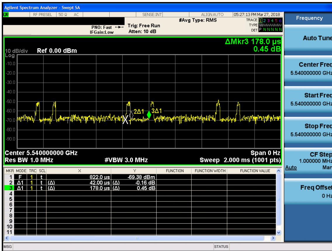
Figure 5-2. Band 2C Pulse Width
