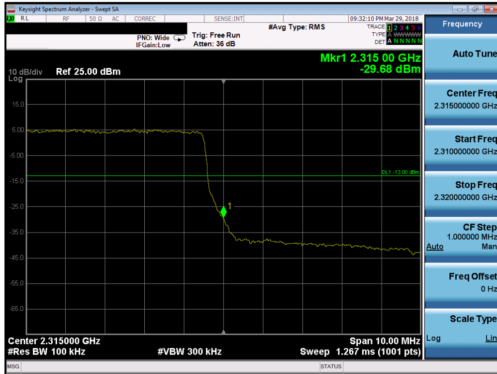
Plot 7-272. Upper Band Edge Plot (Band 30 - 10.0MHz QPSK - Full RB Configuration)
