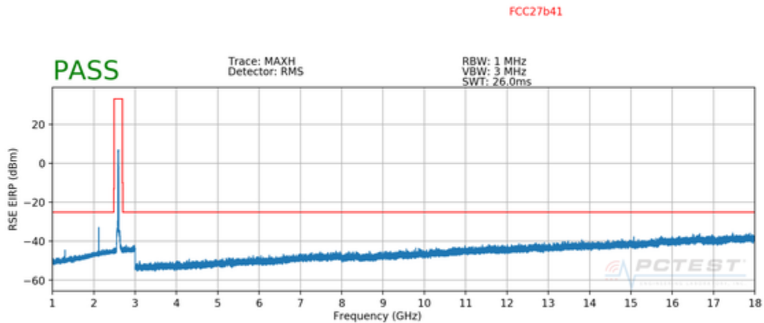
Plot 7-70. Radiated Spurious Plot (ULCA B41 PCC: RB 100 Offset 0, SCC: RB 100 Offset 0, Ant. Pol. H) – Mid Channel
