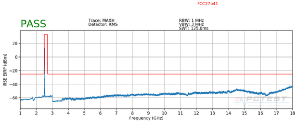
Plot 7-69. Radiated Spurious Data (ULCA B41 PCC: RB 1 Offset 99, SCC: RB 1 Offset 0, Ant. Pol. V) – Low Channel
