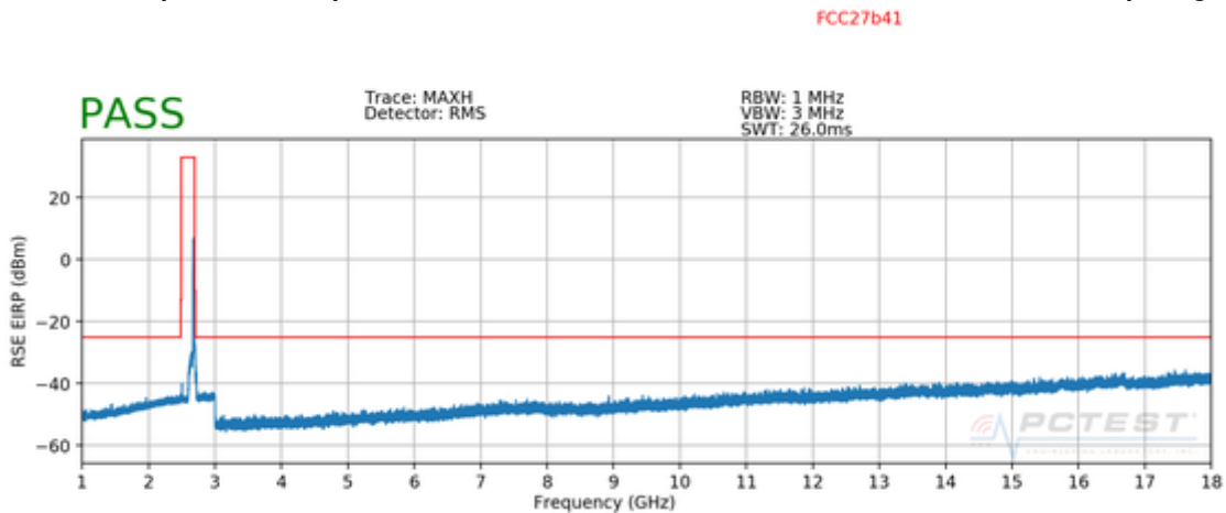
Plot 7-77. Radiated Spurious Data (ULCA B41 PCC: RB 1 Offset 99, SCC: RB 1 Offset 0, Ant. Pol. V) – High Channel
