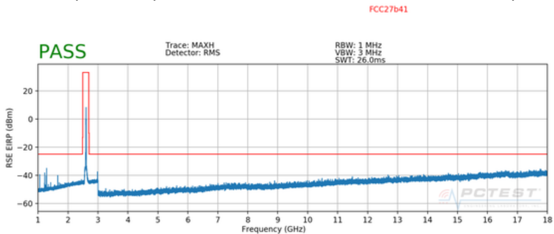
Plot 7-73. Radiated Spurious Data (ULCA B41 PCC: RB 1 Offset 99, SCC: RB 1 Offset 0, Ant. Pol. V) – Mid Channel
