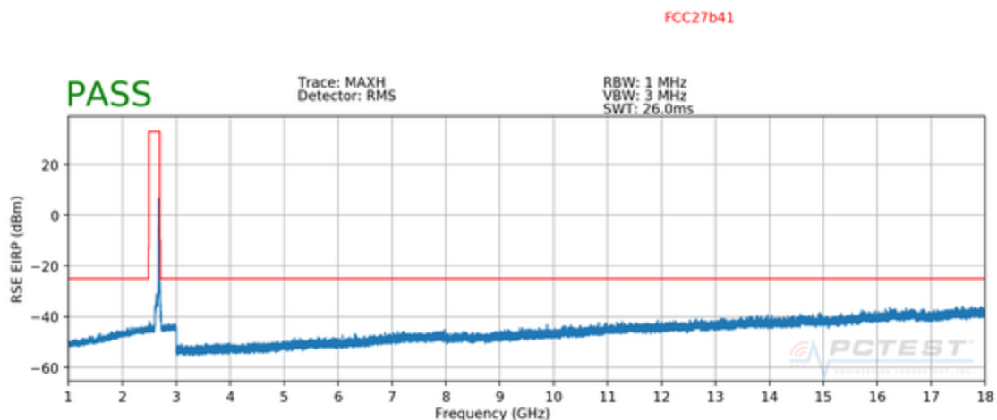
Plot 7-74. Radiated Spurious Plot (ULCA B41 PCC: RB 100 Offset 0, SCC: RB 100 Offset 0, Ant. Pol. H) – High Channel
