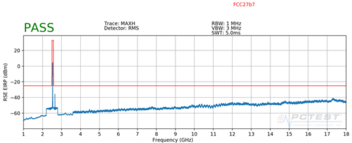
Plot 7-321. Radiated Spurious Plot 1GHz - 18GHz (Band 7)
