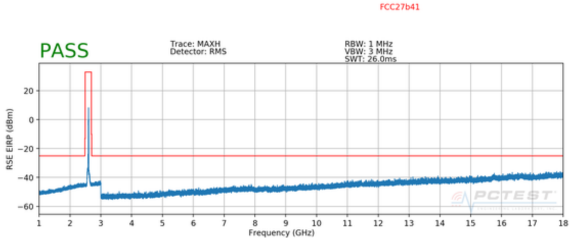
Plot 7-72. Radiated Spurious Data (ULCA B41 PCC: RB 1 Offset 99, SCC: RB 1 Offset 0, Ant. Pol. H) – Mid Channel
