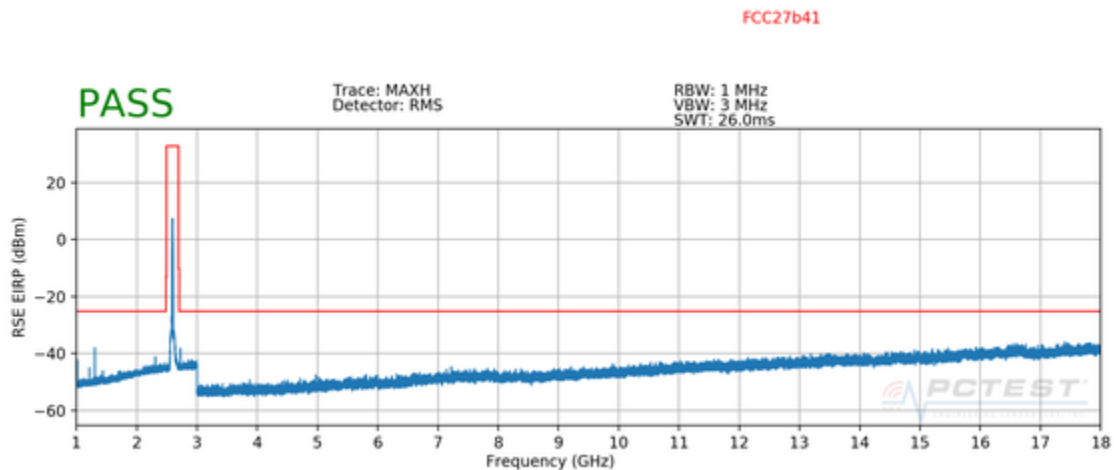
Plot 7-71. Radiated Spurious Plot (ULCA B41 PCC: RB 100 Offset 0, SCC: RB 100 Offset 0, Ant. Pol. V) – Mid Channel
