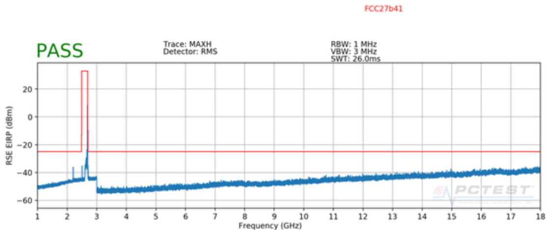
Plot 7-76. Radiated Spurious Data (ULCA B41 PCC: RB 1 Offset 99, SCC: RB 1 Offset 0, Ant. Pol. H) – High Channel
