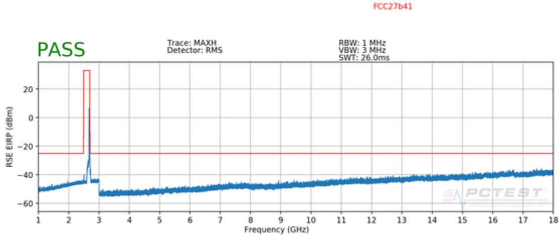
Plot 7-75. Radiated Spurious Plot (ULCA B41 PCC: RB 100 Offset 0, SCC: RB 100 Offset 0, Ant. Pol. V) – High Channel
