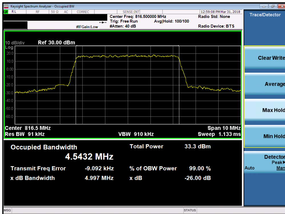
Plot 7-8. Occupied Bandwidth Plot (Band 26 5MHz QPSK – RB Size 25– Low Channel)
