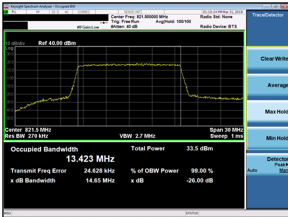
Plot 7-14. Occupied Bandwidth Plot (Band 26 15MHz QPSK – RB Size 75)
