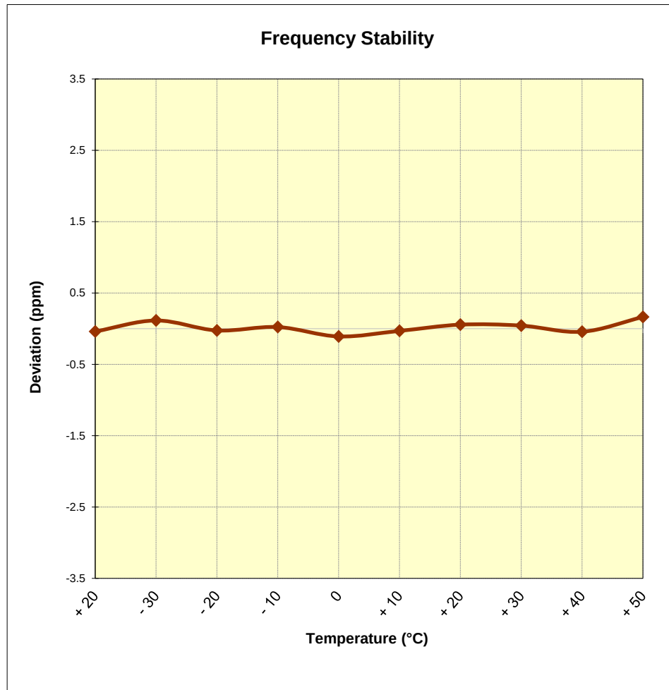
Figure 7-7. Frequency Stability Graph (Band 14)
