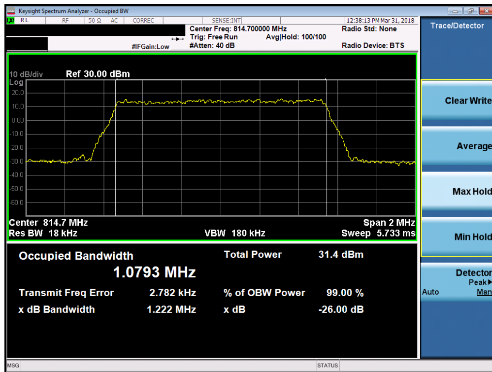
Plot 7-3. Occupied Bandwidth Plot (Band 26 1.4MHz 16-QAM – RB Size 6– Low Channel)
