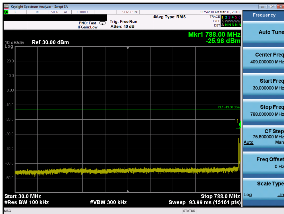
Plot 7-37. Conducted Spurious Plot (Band 14 - 10.0MHz QPSK - RB Size 1, RB Offset 0 High Channel)
