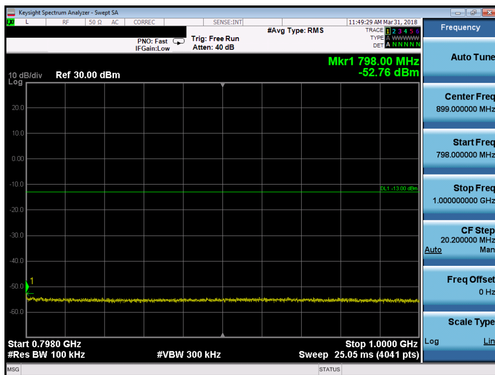
Plot 7-32. Conducted Spurious Plot (Band 14 - 10.0MHz QPSK - RB Size 1, RB Offset 0 Low Channel)
