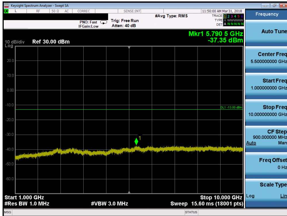
Plot 7-33. Conducted Spurious Plot (Band 14 - 10.0MHz QPSK - RB Size 1, RB Offset 0 Low Channel)
