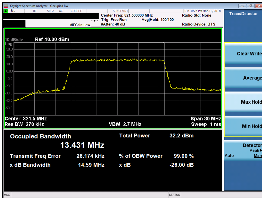
Plot 7-15. Occupied Bandwidth Plot (Band 26 15MHz 16-QAM – RB Size 75)
