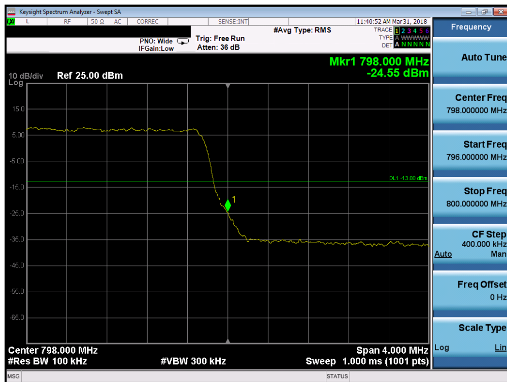
Plot 7-42. Upper Band Edge Plot (Band 14 - 5.0MHz QPSK - Full RB Configuration)
