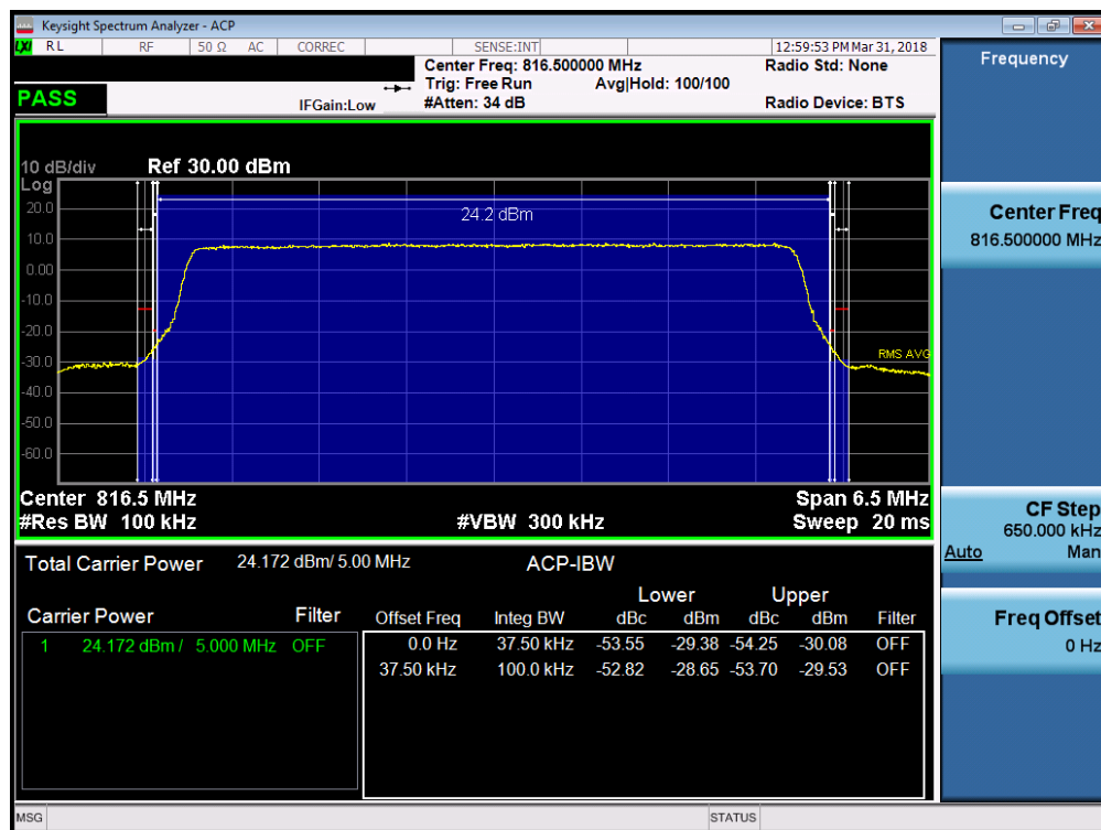
Plot 7-54. Channel Edge Plot (Band 26 - 5MHz QPSK – RB Size 25– Low Channel)
