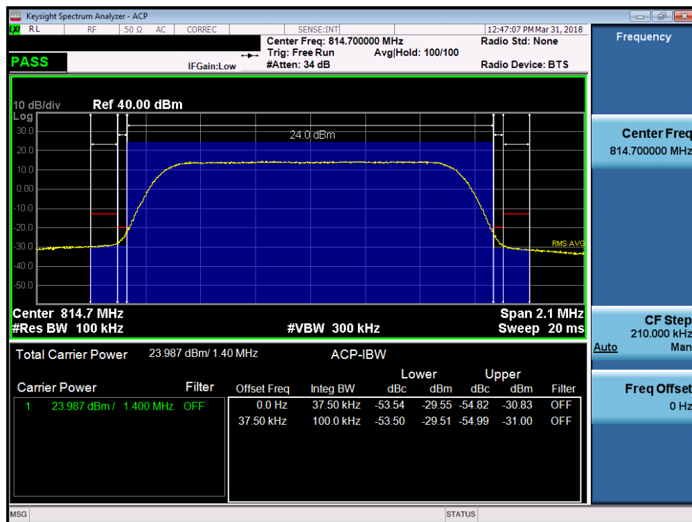
Plot 7-50. Channel Edge Plot (Band 26 - 1.4MHz QPSK – RB Size 6– Low Channel)
