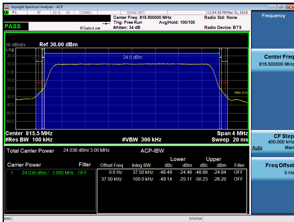
Plot 7-52. Channel Edge Plot (Band 26 - 3MHz QPSK – RB Size 15– Low Channel)
