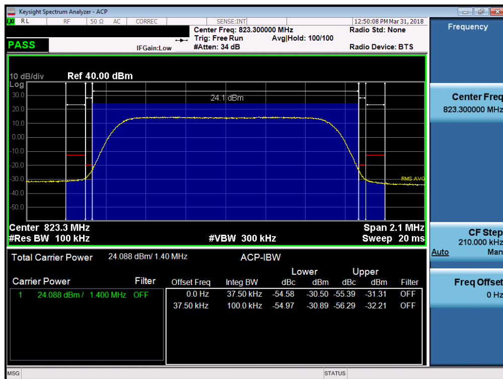
Plot 7-51. Channel Edge Plot (Band 26 - 1.4MHz QPSK – RB Size 6 – High Channel)
