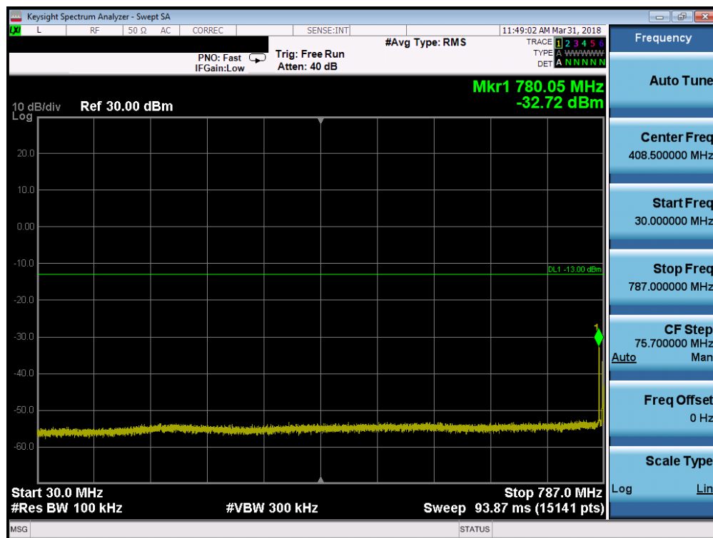
Plot 7-31. Conducted Spurious Plot (Band 14 - 10.0MHz QPSK - RB Size 1, RB Offset 0 Low Channel)
