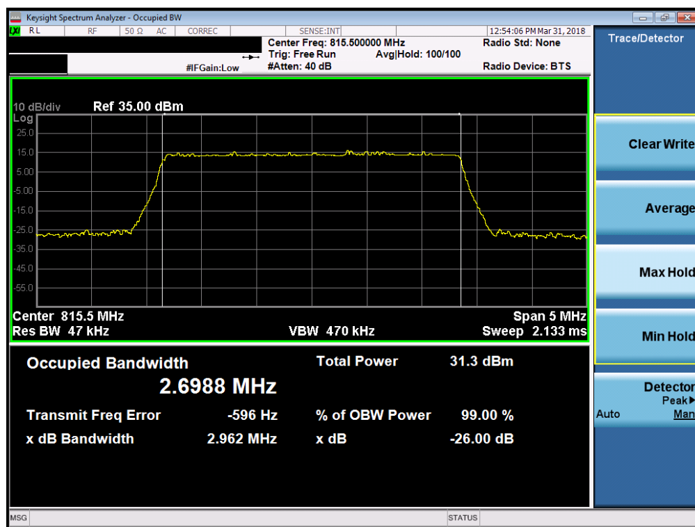
Plot 7-7. Occupied Bandwidth Plot (Band 26 3MHz 64-QAM – RB Size 15– Low Channel)
