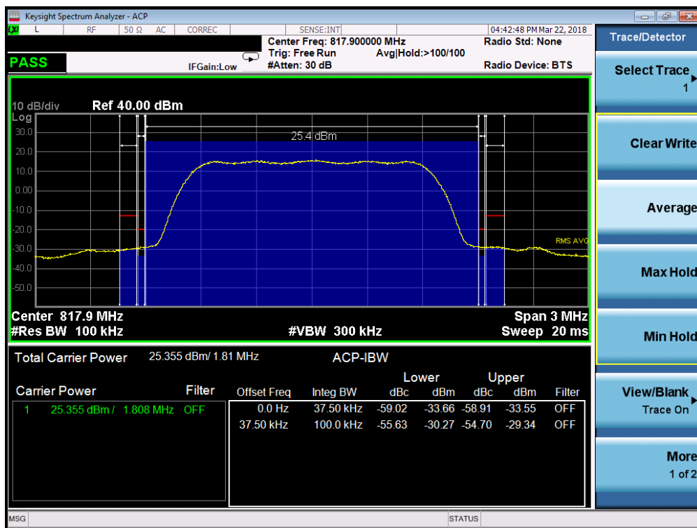
Plot 7-48. Channel Edge Plot (CDMA Ch. 476)
