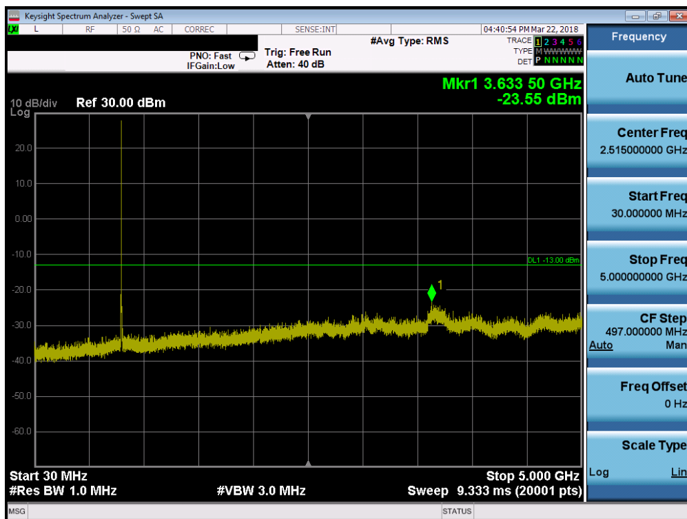
Plot 7-23. Conducted Spurious Plot (CDMA Ch. 476)
