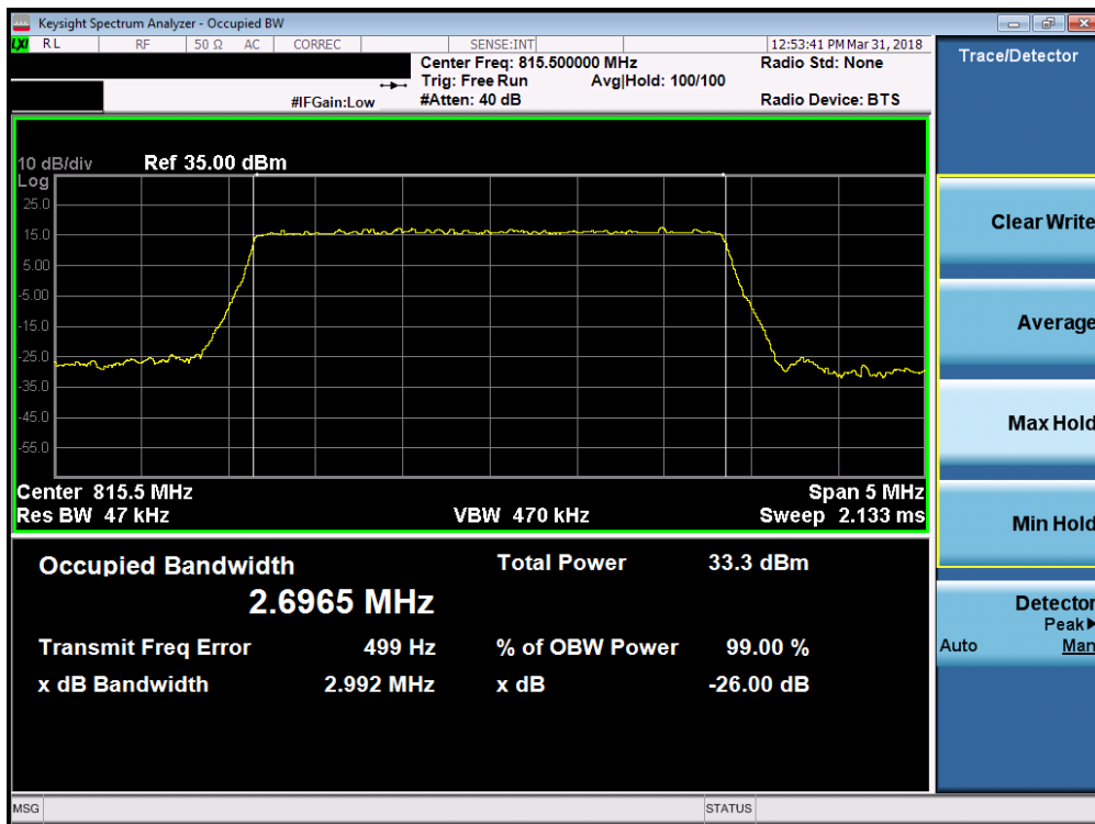
Plot 7-5. Occupied Bandwidth Plot (Band 26 3MHz QPSK – RB Size 15– Low Channel)
