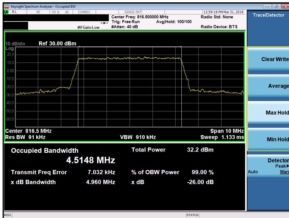
Plot 7-9. Occupied Bandwidth Plot (Band 26 5MHz 16-QAM – RB Size 25– Low Channel)
