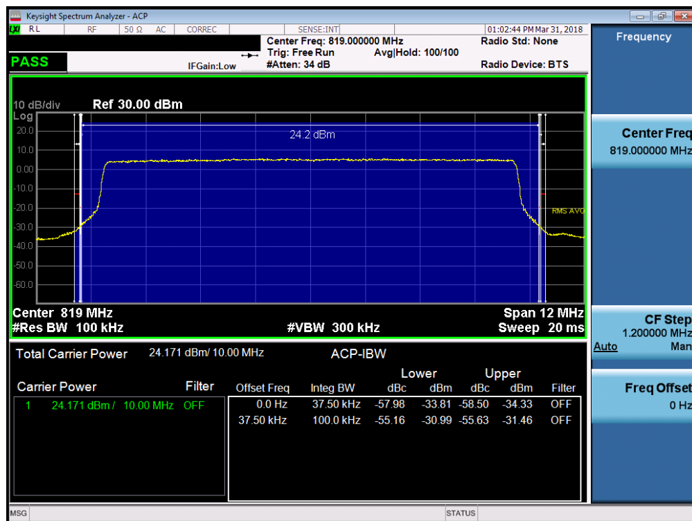
Plot 7-56. Channel Edge Plot (Band 26 - 10MHz QPSK – RB Size 50)
