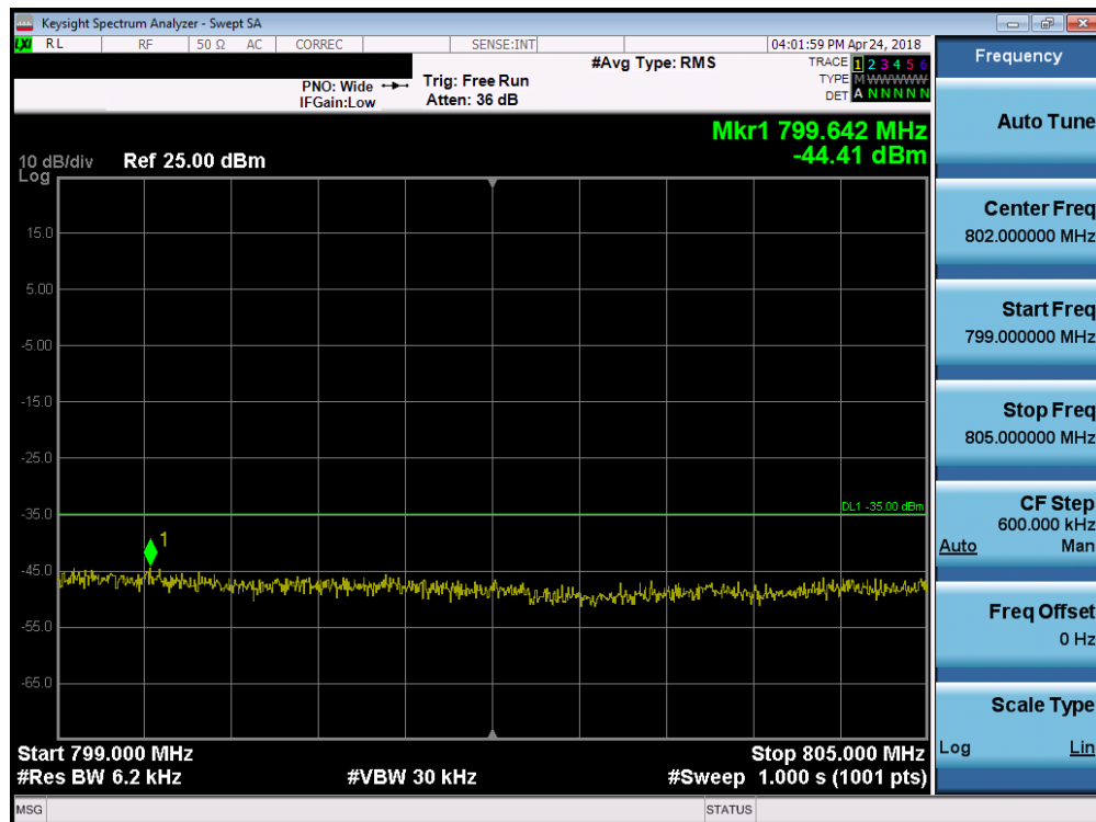
Plot 7-43. Upper Emission Mask Plot (Band 14 - 5.0MHz QPSK - Full RB Configuration)
