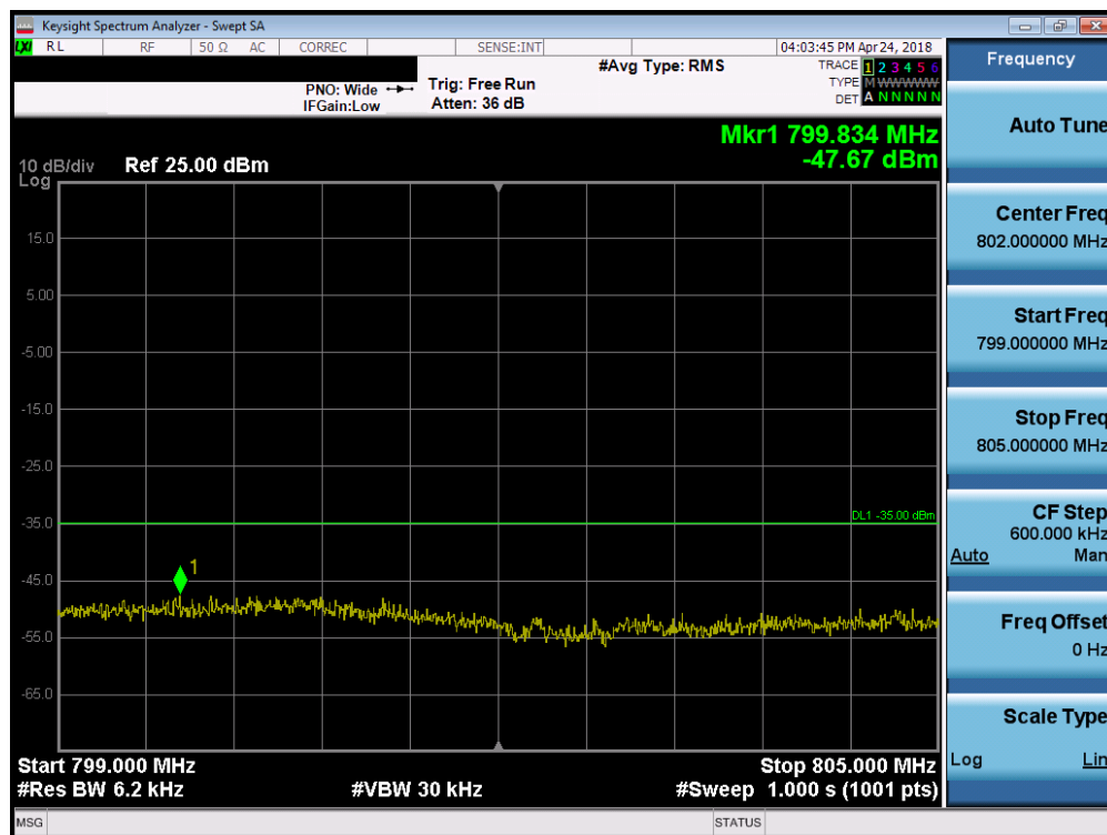
Plot 7-47. Upper Emission Mask Plot (Band 14 - 10.0MHz QPSK - Full RB Configuration)
