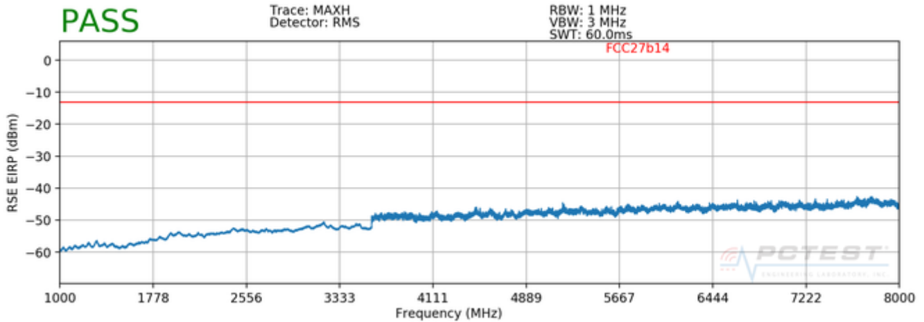
Plot 7-59. Radiated Spurious Plot above 1GHz (Band 14)
