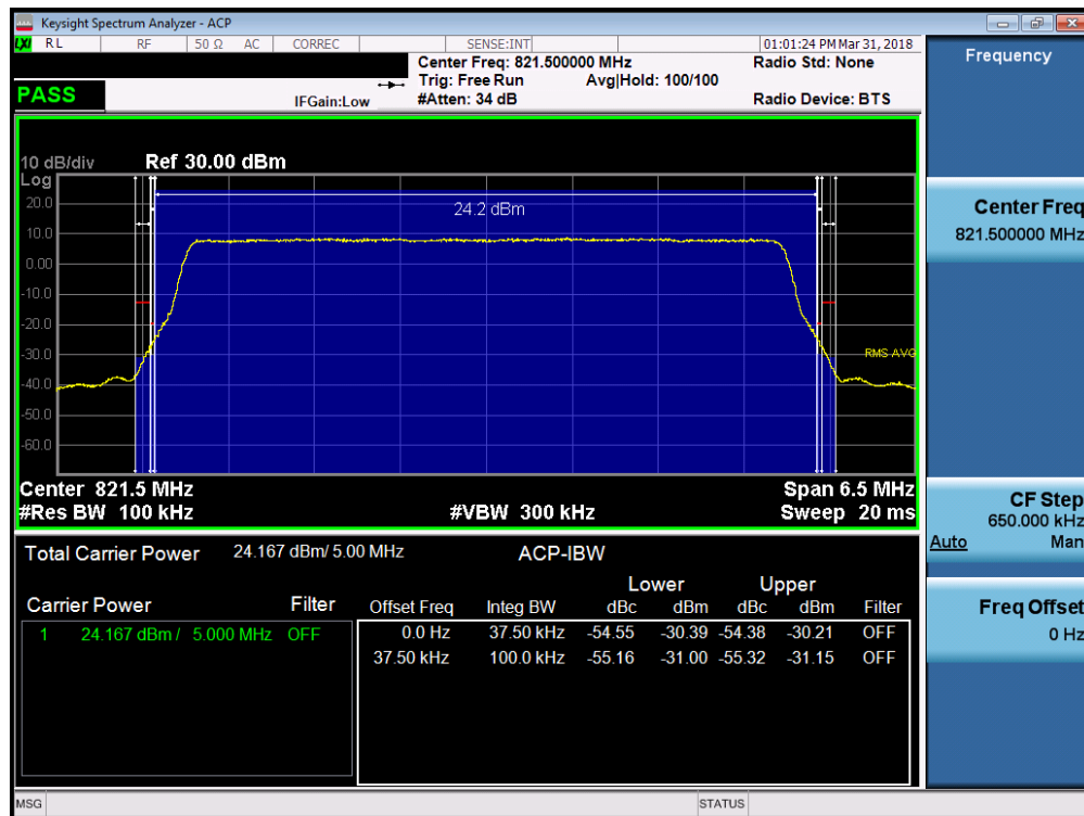
Plot 7-55. Channel Edge Plot (Band 26 - 5MHz QPSK – RB Size 25 – High Channel)
