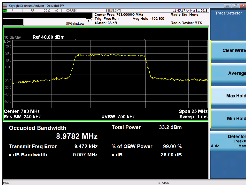
Plot 7-20. Occupied Bandwidth Plot (Band 14 - 10.0MHz QPSK - Full RB Configuration)
