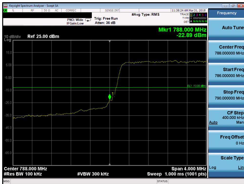
Plot 7-40. Lower Band Edge Plot (Band 14 - 5.0MHz QPSK - Full RB Configuration)
