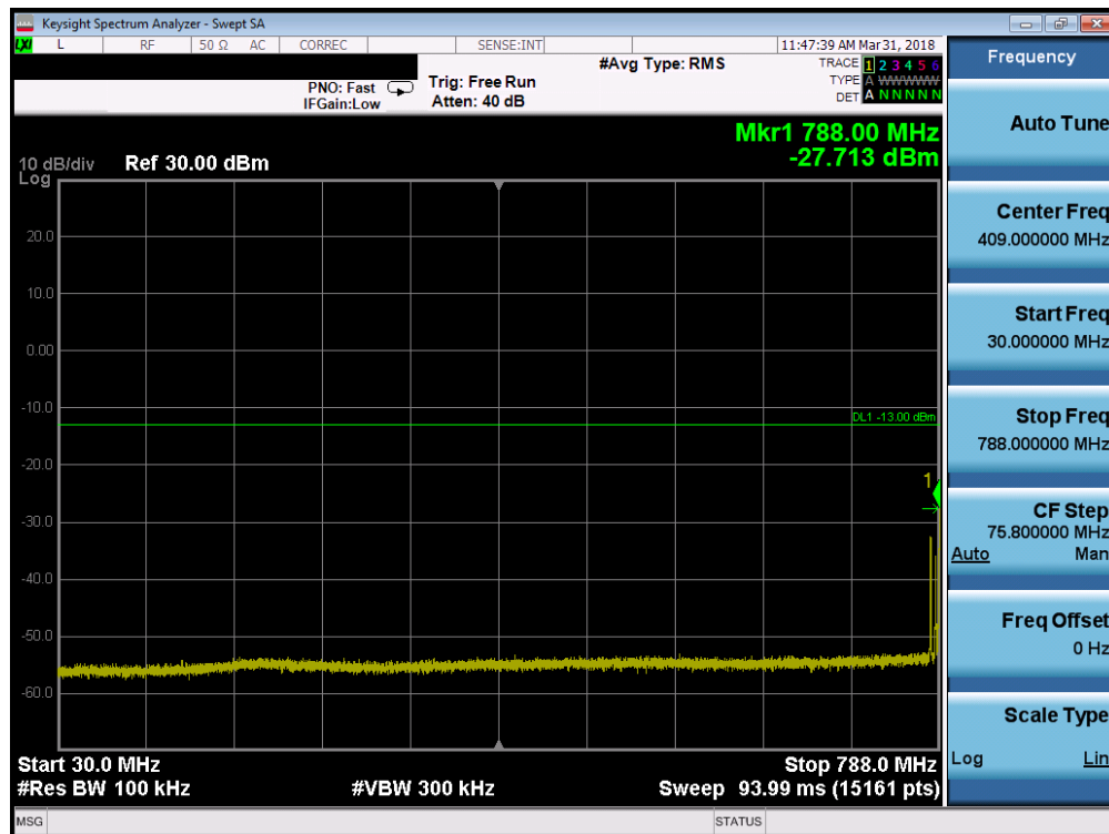
Plot 7-34. Conducted Spurious Plot (Band 14 - 10.0MHz QPSK - RB Size 1, RB Offset 0 Mid Channel)
