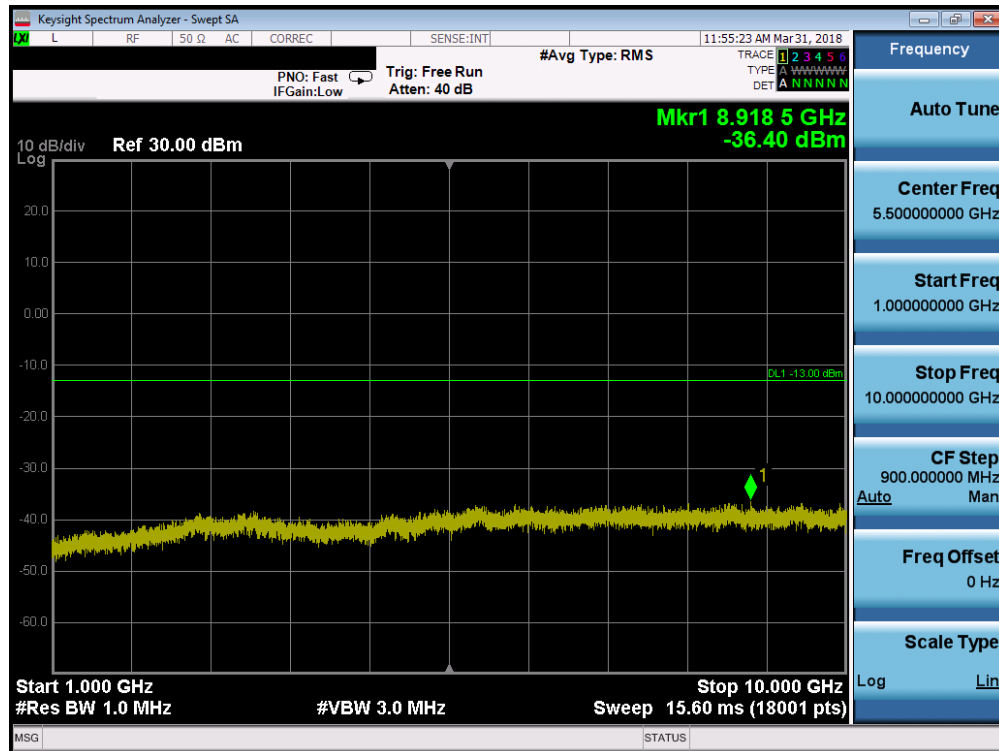
Plot 7-39. Conducted Spurious Plot (Band 14 - 10.0MHz QPSK - RB Size 1, RB Offset 0 High Channel)
