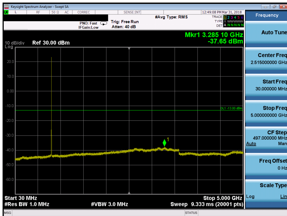
Plot 7-29. Conducted Spurious Plot (Band 26 - 1.4MHz QPSK – RB Size 1, RB Offset 0 – High Channel)
