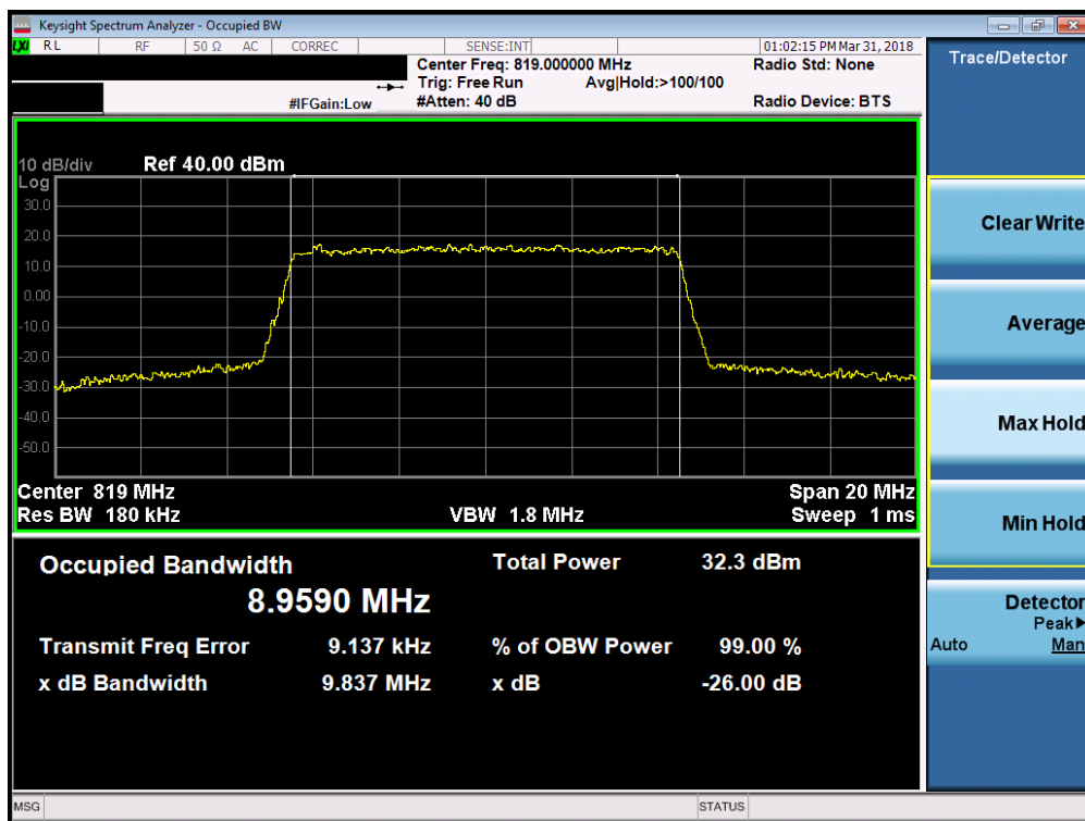
Plot 7-12. Occupied Bandwidth Plot (Band 26 10MHz 16-QAM – RB Size 50)
