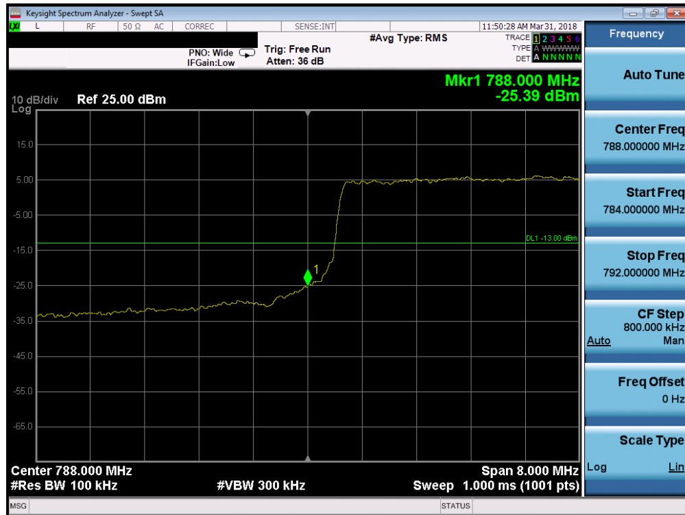
Plot 7-44. Lower Band Edge Plot (Band 14 - 10.0MHz QPSK - Full RB Configuration)
