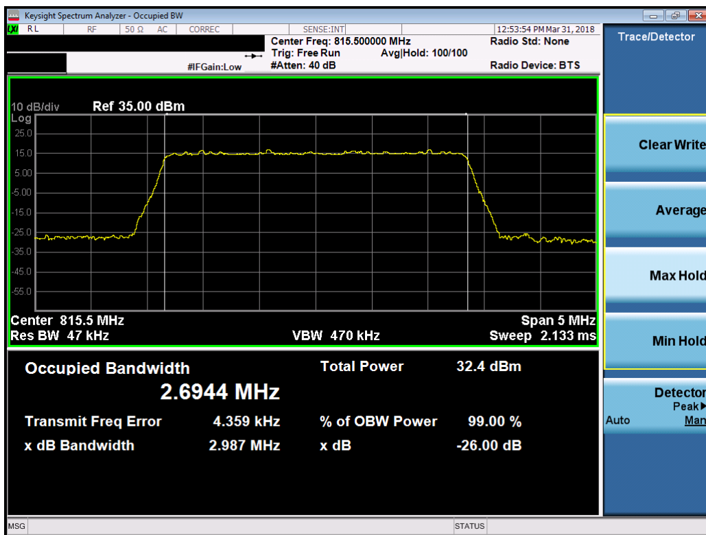
Plot 7-6. Occupied Bandwidth Plot (Band 26 3MHz 16-QAM – RB Size 15– Low Channel)
