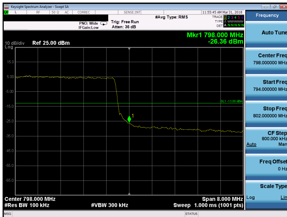
Plot 7-46. Upper Band Edge Plot (Band 14 - 10.0MHz QPSK - Full RB Configuration)
