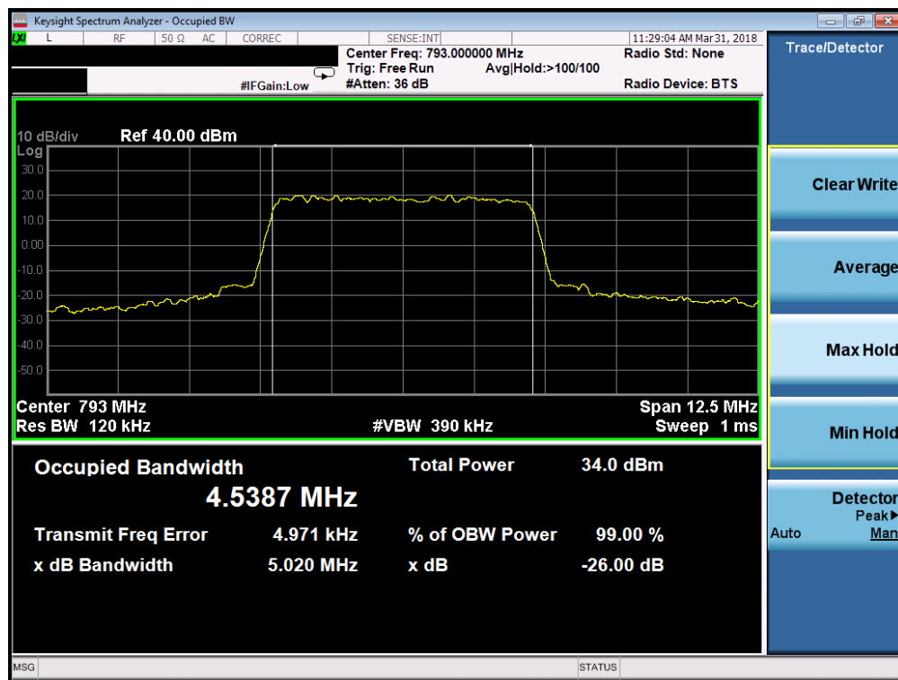
Plot 7-17. Occupied Bandwidth Plot (Band 14 - 5.0MHz QPSK - Full RB Configuration)
