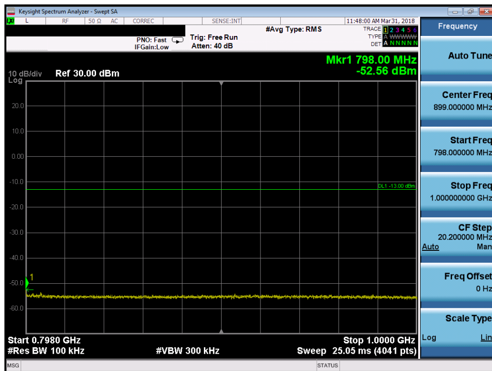
Plot 7-35. Conducted Spurious Plot (Band 14 - 10.0MHz QPSK - RB Size 1, RB Offset 0 Mid Channel)
