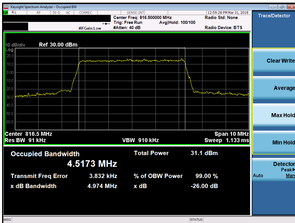
Plot 7-10. Occupied Bandwidth Plot (Band 26 5MHz 64-QAM – RB Size 25– Low Channel)
