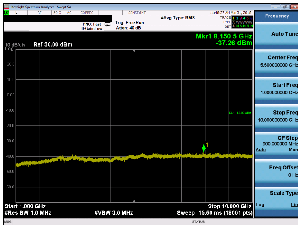
Plot 7-36. Conducted Spurious Plot (Band 14 - 10.0MHz QPSK - RB Size 1, RB Offset 0 Mid Channel)
