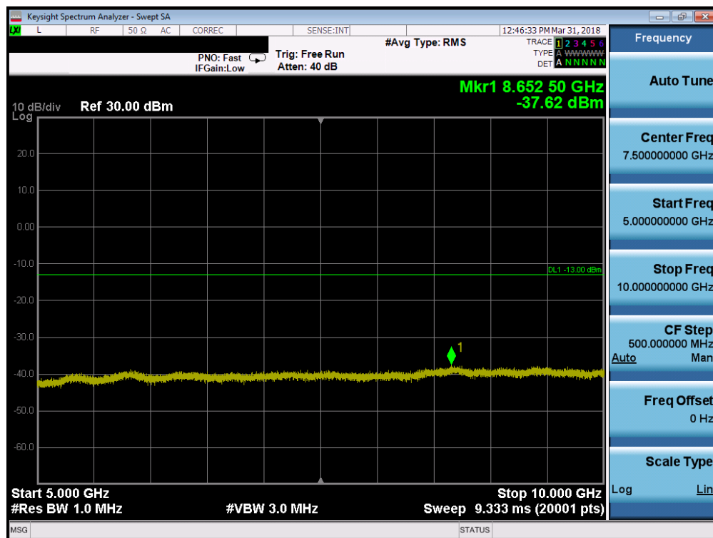
Plot 7-28. Conducted Spurious Plot (Band 26 - 1.4MHz QPSK – RB Size 1, RB Offset 0 – Low Channel)
