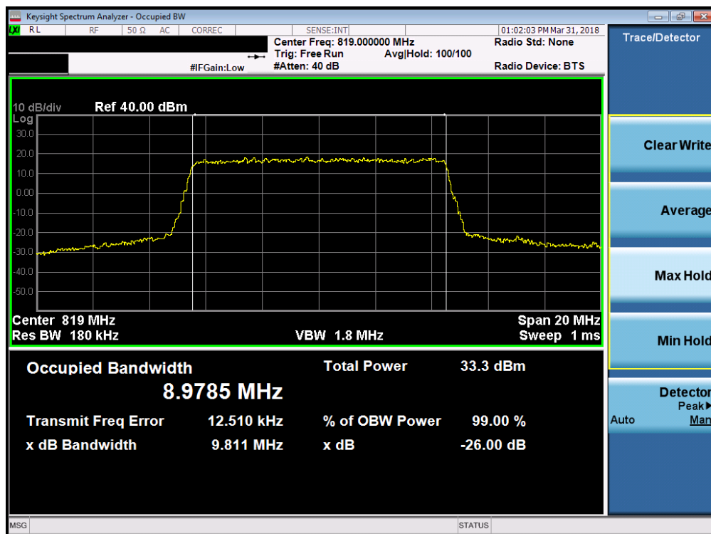
Plot 7-11. Occupied Bandwidth Plot (Band 26 10MHz QPSK – RB Size 50)
