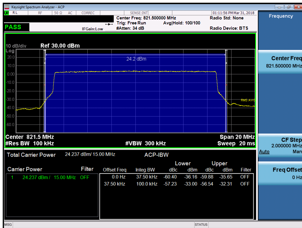
Plot 7-57. Channel Edge Plot (Band 26 - 15MHz QPSK – RB Size 75)
