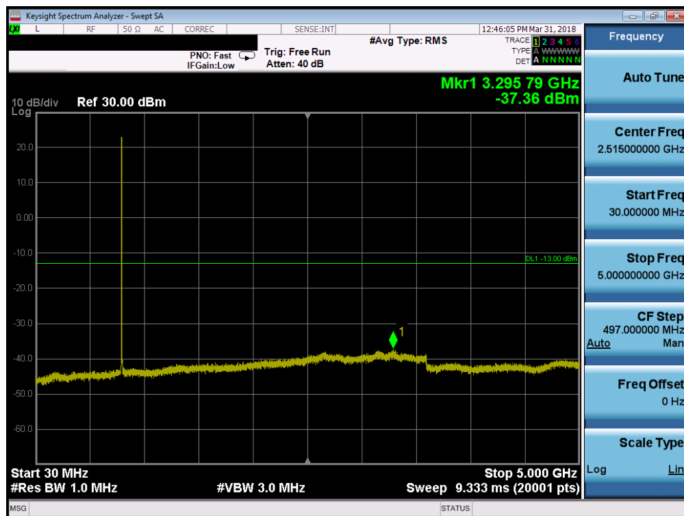
Plot 7-27. Conducted Spurious Plot (Band 26 - 1.4MHz QPSK – RB Size 1, RB Offset 0 – Low Channel)
