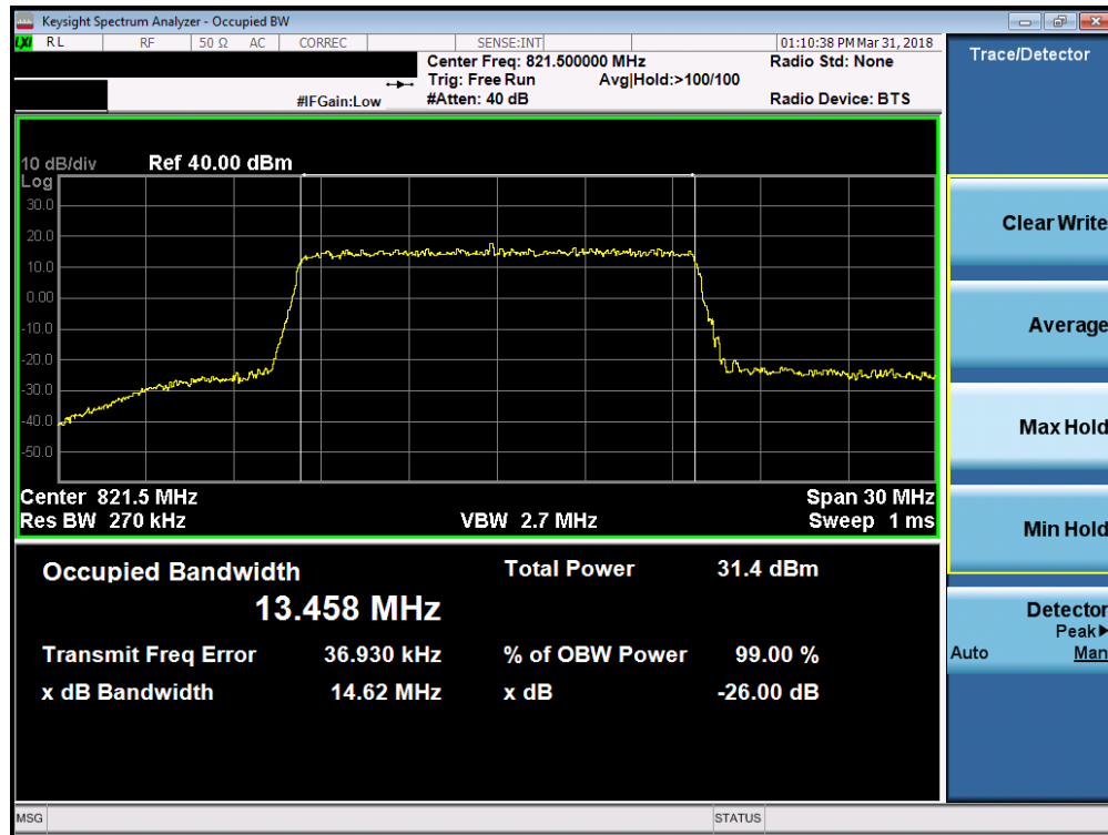
Plot 7-16. Occupied Bandwidth Plot (Band 26 15MHz 64-QAM – RB Size 75)
