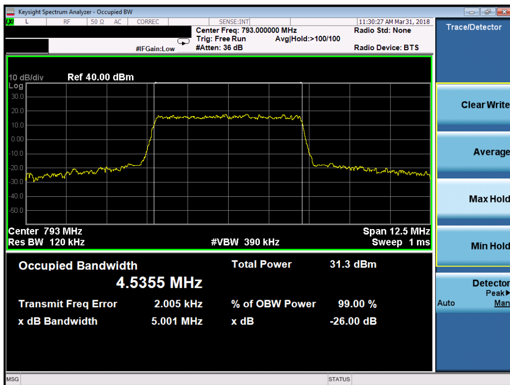
Plot 7-19. Occupied Bandwidth Plot (Band 14 - 5.0MHz 64-QAM - Full RB Configuration)
