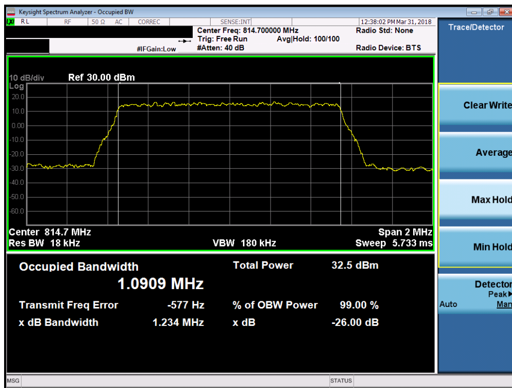
Plot 7-2. Occupied Bandwidth Plot (Band 26 1.4MHz QPSK – RB Size 6– Low Channel)
