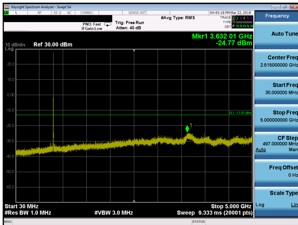
Plot 7-25. Conducted Spurious Plot (CDMA Ch. 684)
