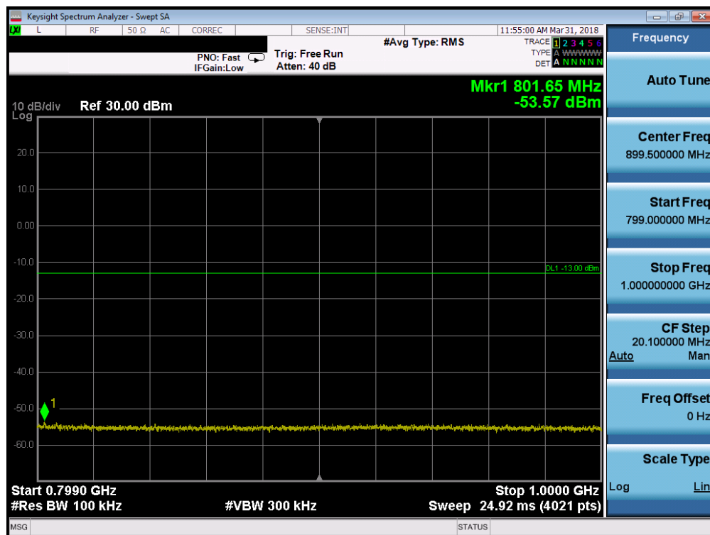
Plot 7-38. Conducted Spurious Plot (Band 14 - 10.0MHz QPSK - RB Size 1, RB Offset 0 High Channel)
