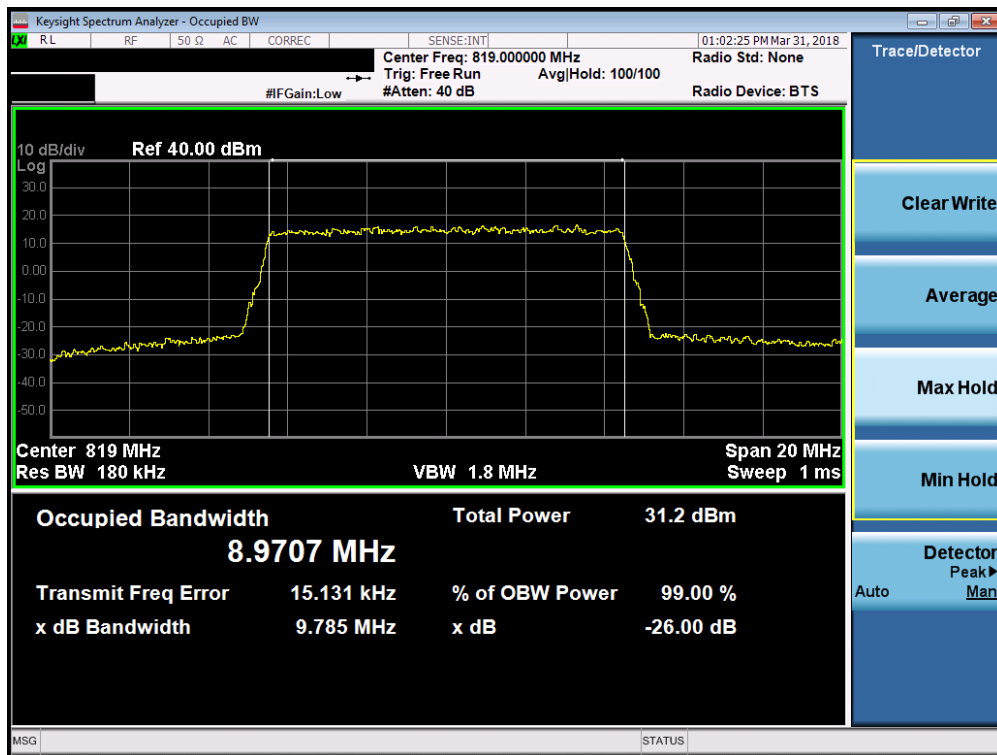
Plot 7-13. Occupied Bandwidth Plot (Band 26 10MHz 64-QAM – RB Size 50)
