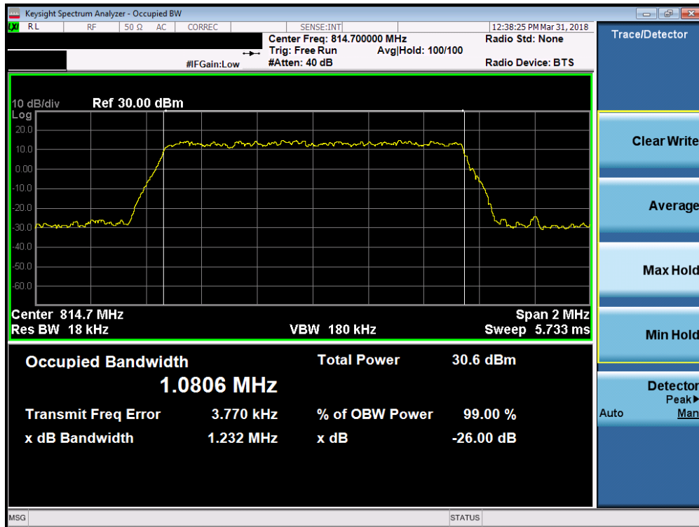
Plot 7-4. Occupied Bandwidth Plot (Band 26 1.4MHz 64-QAM – RB Size 6– Low Channel)
