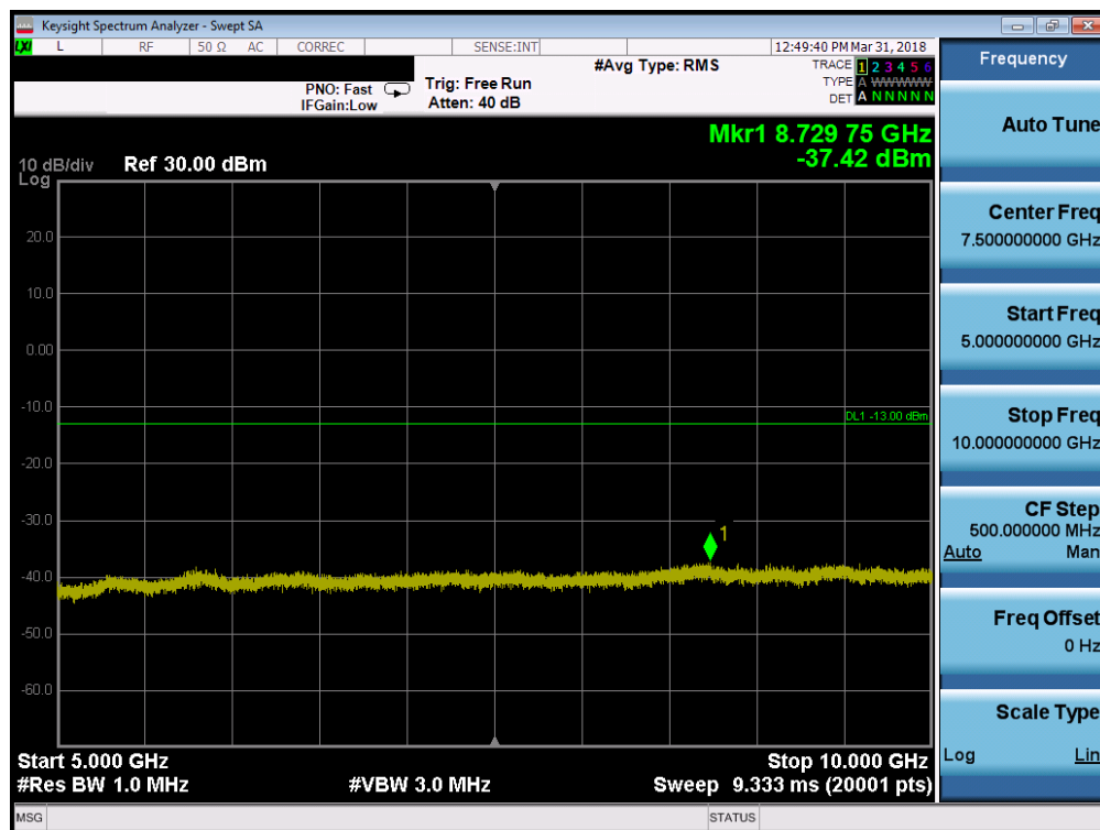
Plot 7-30. Conducted Spurious Plot (Band 26 - 1.4MHz QPSK – RB Size 1, RB Offset 0 – High Channel)
