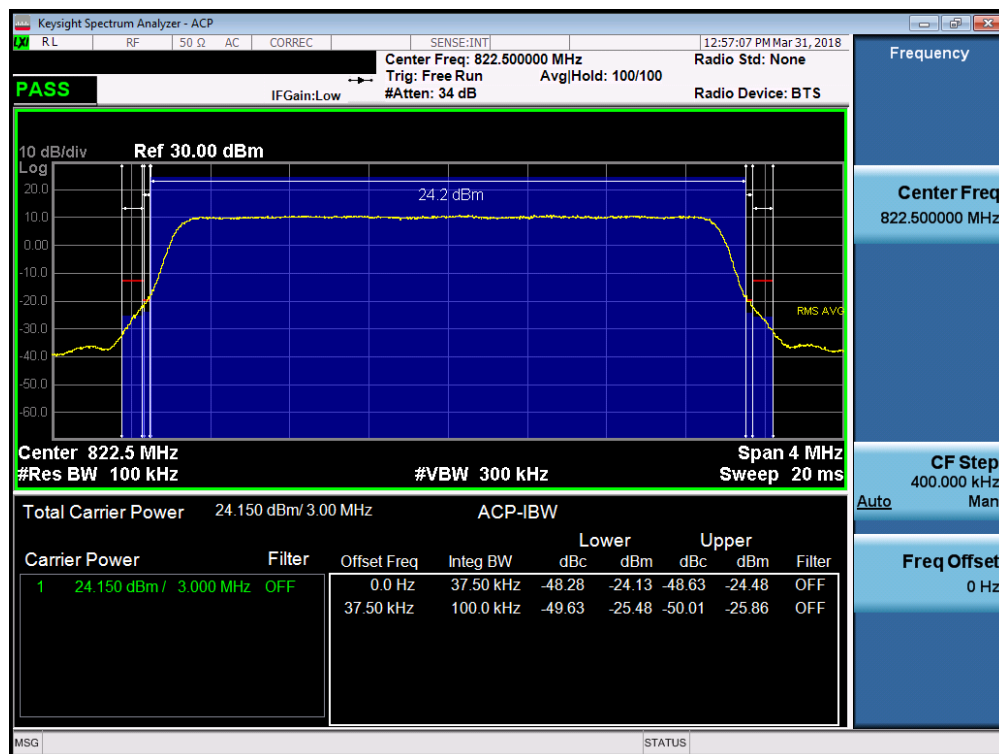
Plot 7-53. Channel Edge Plot (Band 26 - 3MHz QPSK – RB Size 15 – High Channel)
