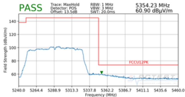
Plot 7-220. Radiated Upper Band Edge Plot SISO ANT2 (Peak – UNII Band 2A)
