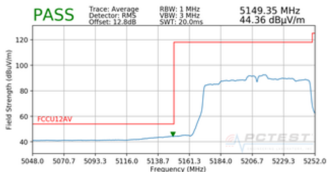
Plot 7-217. Radiated Lower Band Edge Plot SISO ANT2 (Average – UNII Band 1)
