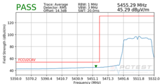
Plot 7-212. Radiated Lower Band Edge Plot SISO ANT2 (Average – UNII Band 2C)
