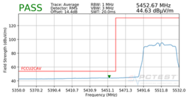
Plot 7-188. Radiated Band Edge Plot SISO ANT1 (Average – WCP)
