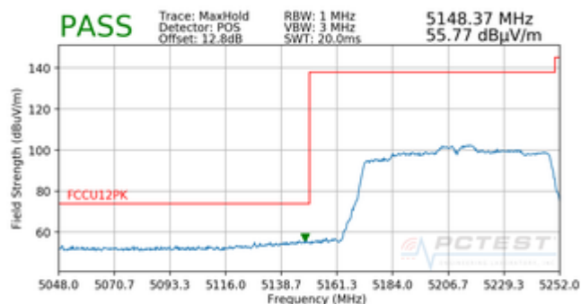
Plot 7-218. Radiated Lower Band Edge Plot SISO ANT2 (Peak – UNII Band 1)
