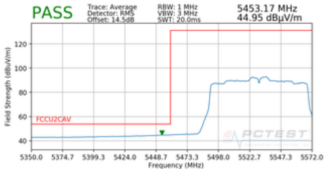
Plot 7-194. Radiated Lower Band Edge Plot SISO ANT1 (Average – UNII Band 2C)
