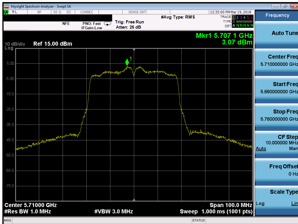
Plot 7-105. Power Spectral Density Plot SISO ANT1 (40MHz BW 802.11n (UNII Band 2C) – Ch. 134142)
