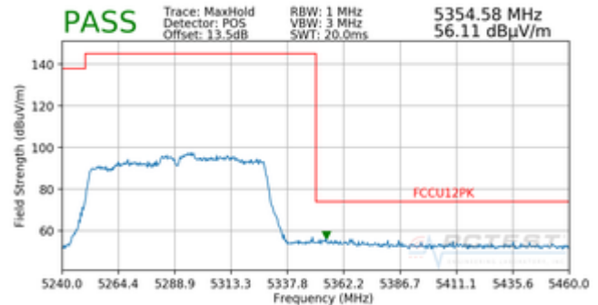
Plot 7-193. Radiated Upper Band Edge Plot SISO ANT1 (Peak – UNII Band 2A)
