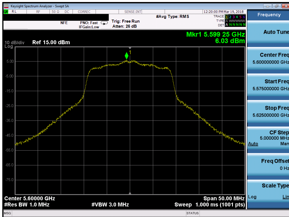
Plot 7-101. Power Spectral Density Plot SISO ANT1 (20MHz BW 802.11n (UNII Band 2C) – Ch. 116120)
