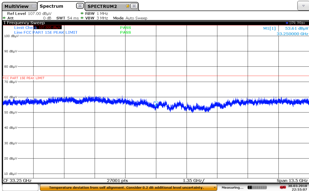
Plot 7-162. Radiated Spurious Plot 26.5GHz - 40GHz SISO ANT1 (802.11a)
