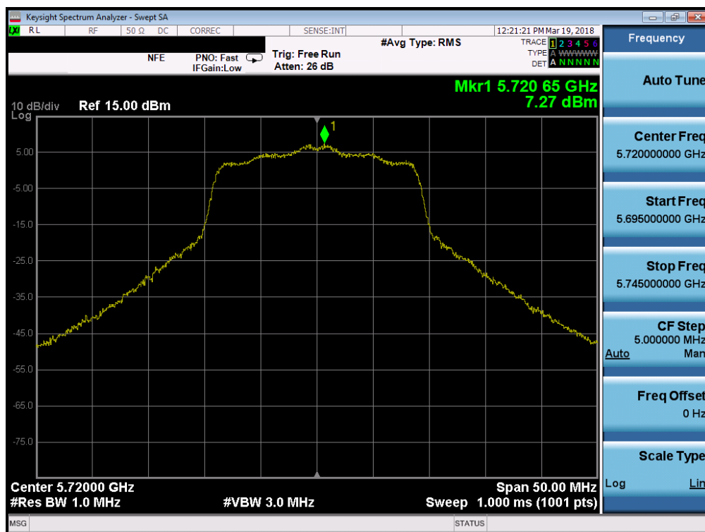
Plot 7-102. Power Spectral Density Plot SISO ANT1 (20MHz BW 802.11n (UNII Band 2C) – Ch. 140144)
