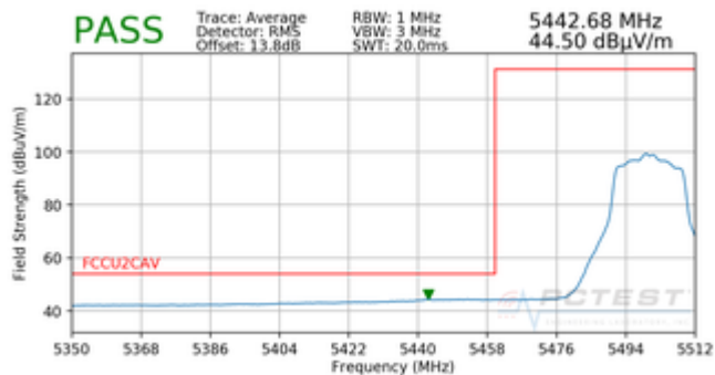
Plot 7-179. Radiated Band Edge Plot SISO ANT1 (Average – WCP)
