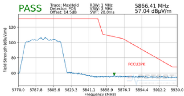
Plot 7-187. Radiated Upper Band Edge Plot SISO ANT1 (Peak – UNII Band 3)
