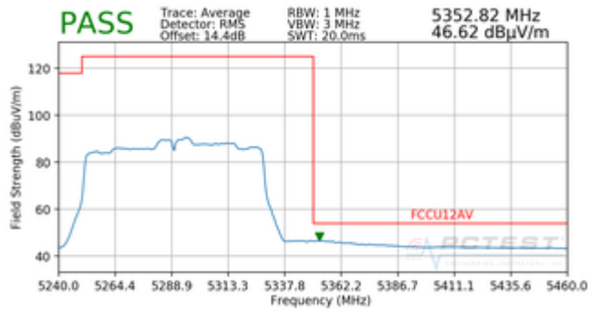
Plot 7-197. Radiated Band Edge Plot SISO ANT1 (Average – WCP)
