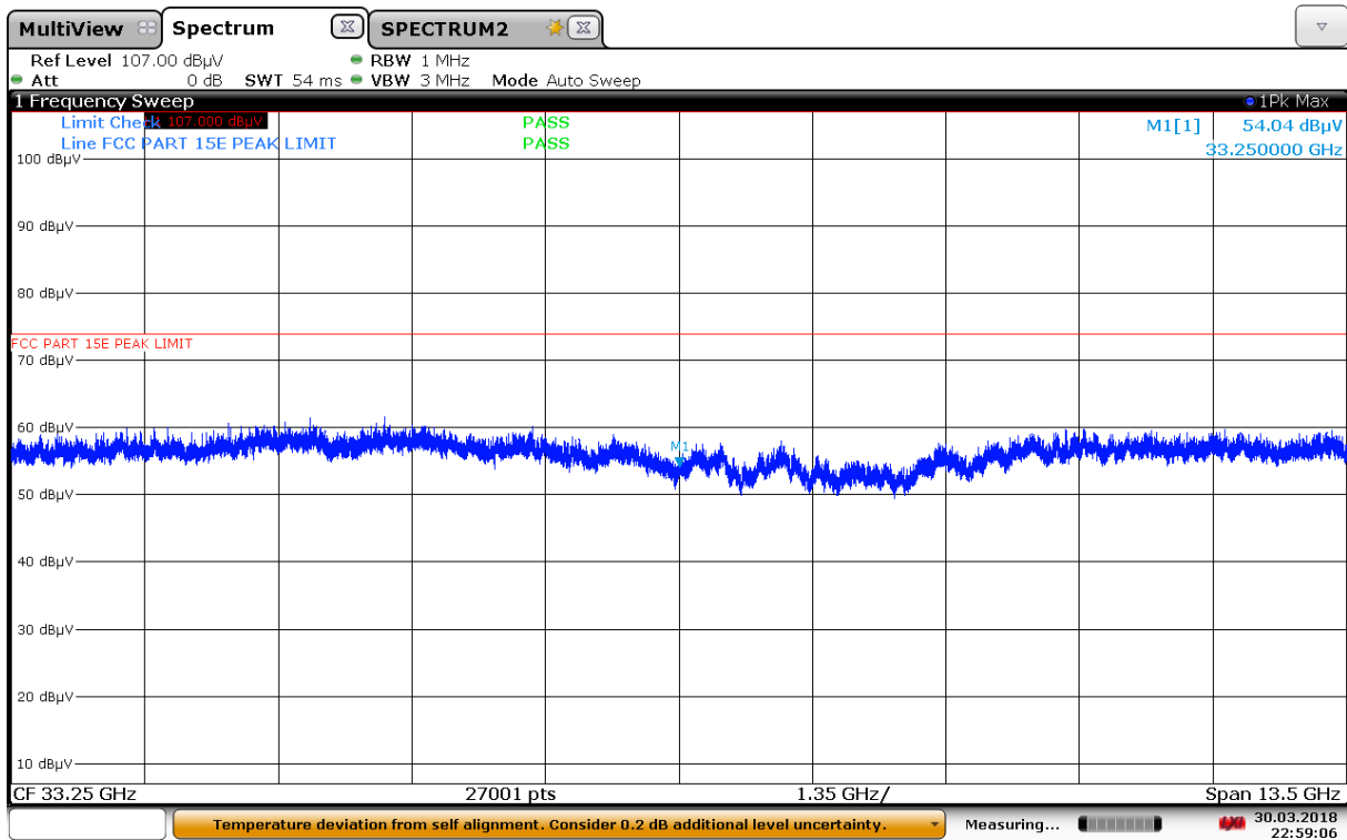
Plot 7-168. Radiated Spurious Plot 26.5GHz - 40GHz SISO ANT2 (802.11a)
