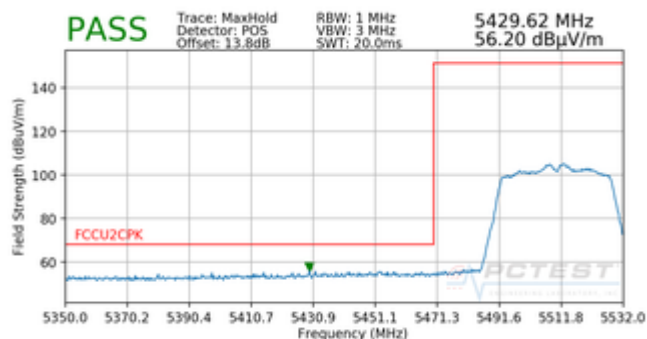
Plot 7-186. Radiated Lower Band Edge Plot SISO ANT1 (Peak – UNII Band 2C)
