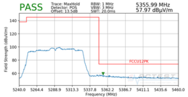
Plot 7-198. Radiated Band Edge Plot SISO ANT1 (Peak – WCP)
