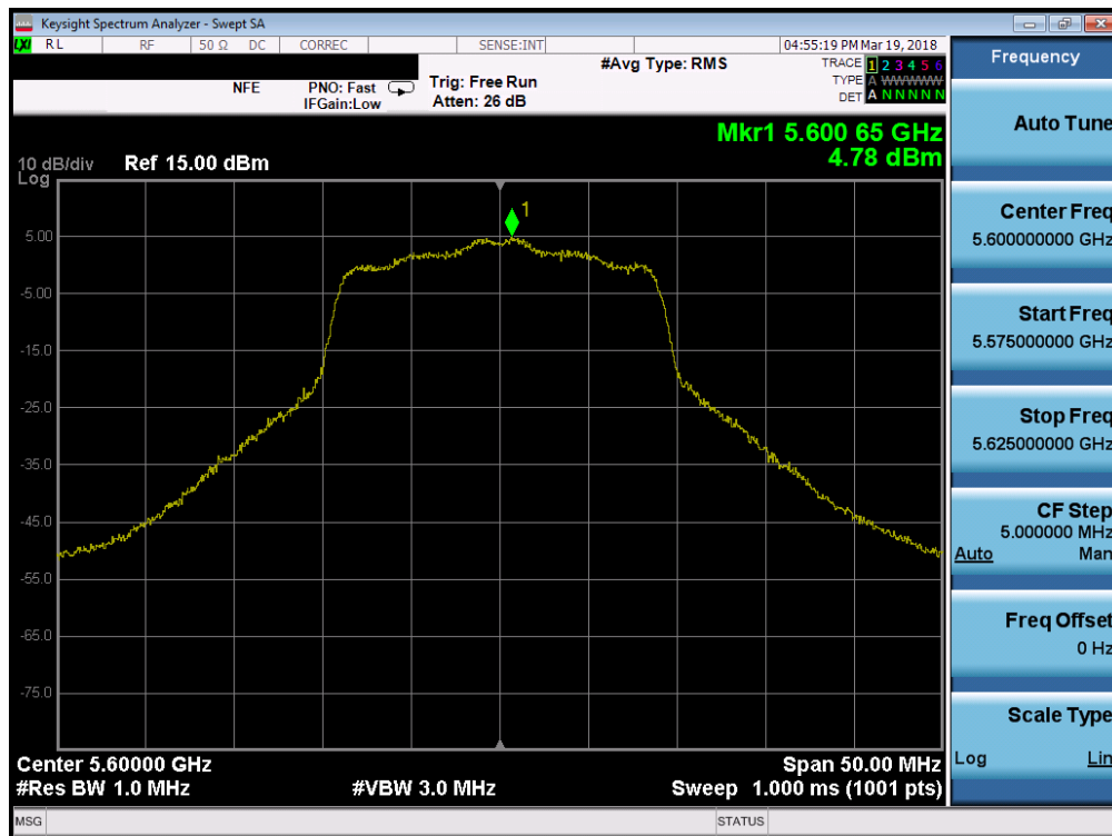
Plot 7-140. Power Spectral Density Plot SISO ANT2 (20MHz BW 802.11n (UNII Band 2C) – Ch. 116120)
