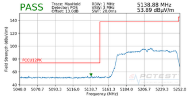
Plot 7-191. Radiated Lower Band Edge Plot SISO ANT1 (Peak – UNII Band 1)
