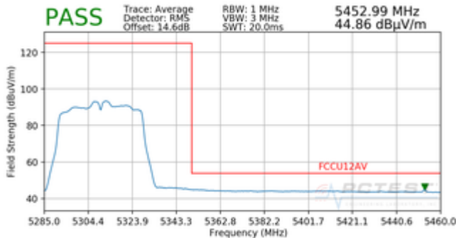
Plot 7-183. Radiated Upper Band Edge Plot SISO ANT1 (Average – UNII Band 2A)
