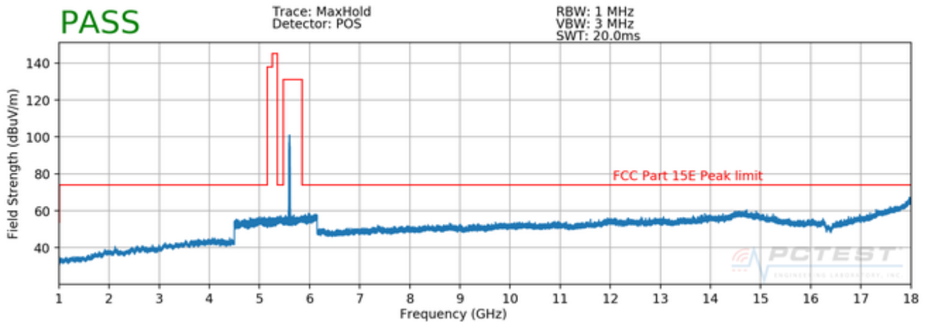
Plot 7-165. Radiated Spurious Plot above 1GHz SISO ANT2 (802.11a – U2C Ch. 116120)
