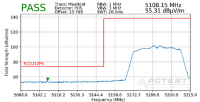
Plot 7-182. Radiated Lower Band Edge Plot SISO ANT1 (Peak – UNII Band 1)
