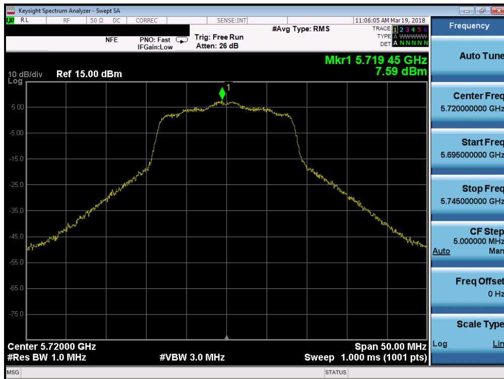
Plot 7-99. Power Spectral Density Plot SISO ANT1 (802.11a (UNII Band 2C) – Ch. 140144)
