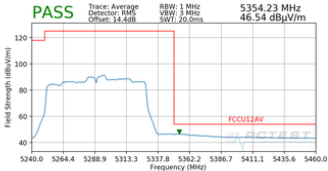
Plot 7-192. Radiated Upper Band Edge Plot SISO ANT1 (Average – UNII Band 2A)
