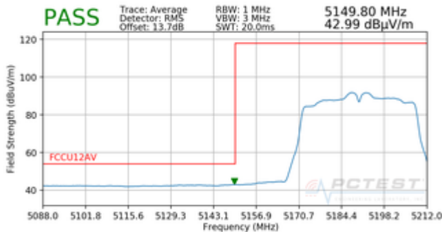
Plot 7-181. Radiated Lower Band Edge Plot SISO ANT1 (Average – UNII Band 1)
