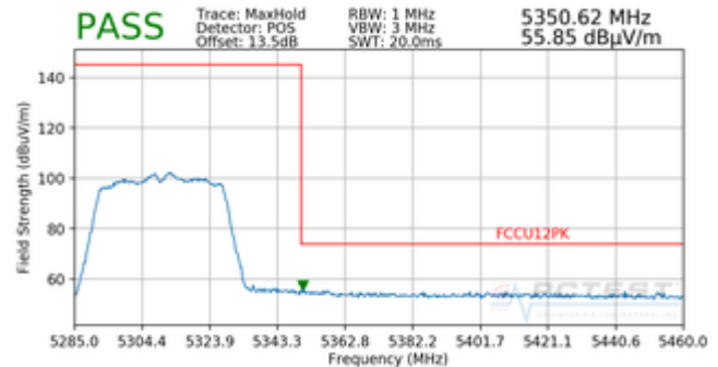
Plot 7-184. Radiated Upper Band Edge Plot SISO ANT1 (Peak – UNII Band 2A)
