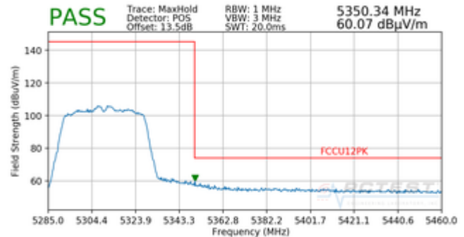
Plot 7-211. Radiated Upper Band Edge Plot SISO ANT2 (Peak – UNII Band 2A)
