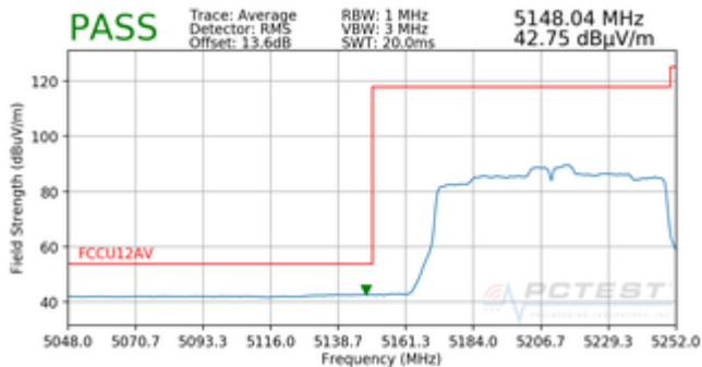
Plot 7-190. Radiated Lower Band Edge Plot SISO ANT1 (Average – UNII Band 1)
