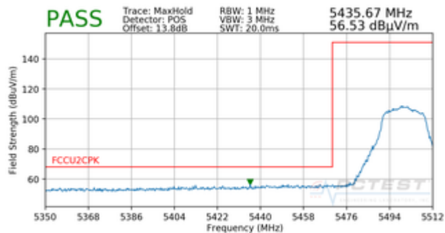
Plot 7-180. Radiated Band Edge Plot SISO ANT1 (Peak – WCP)
