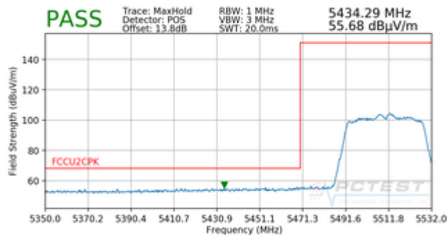
Plot 7-189. Radiated Band Edge Plot SISO ANT1 (Peak – WCP)
