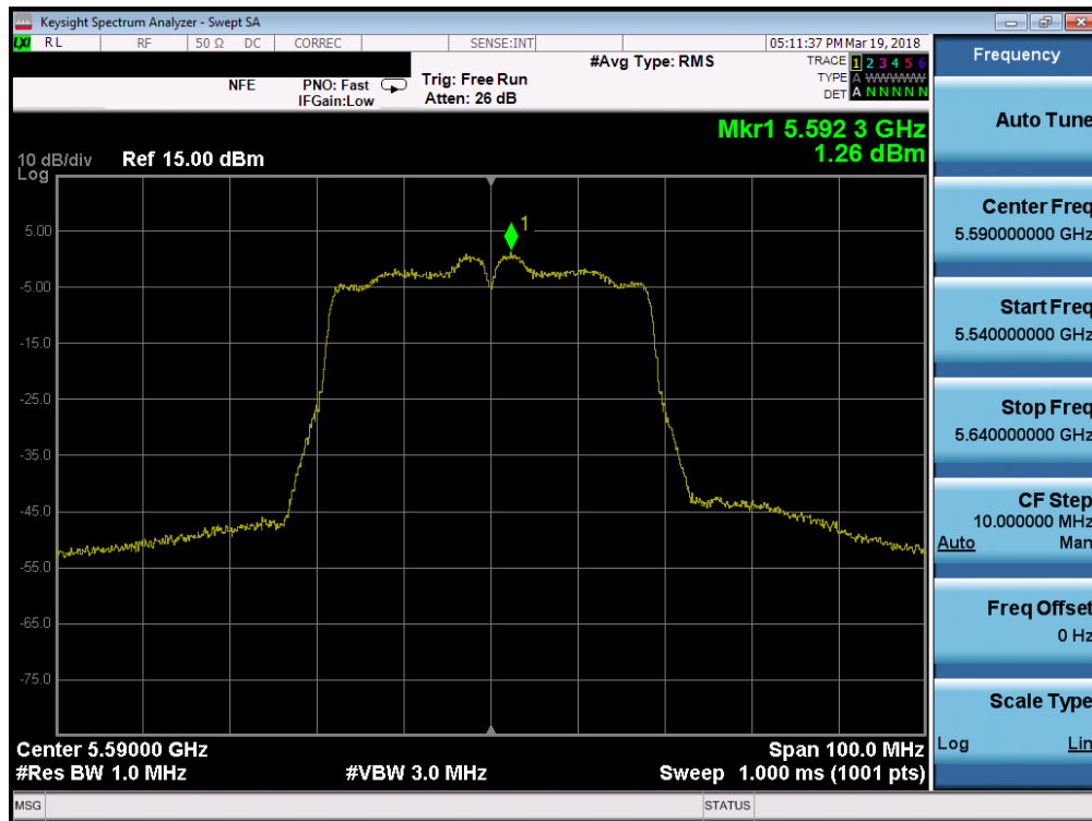
Plot 7-143. Power Spectral Density Plot SISO ANT2 (40MHz BW 802.11n (UNII Band 2C) – Ch. 110118)
