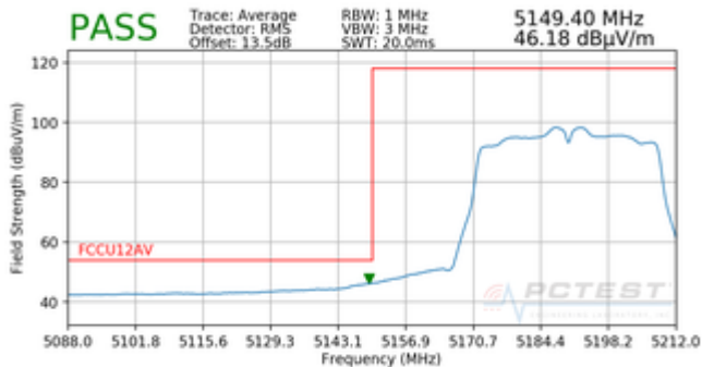
Plot 7-208. Radiated Lower Band Edge Plot SISO ANT2 (Average – UNII Band 1)
