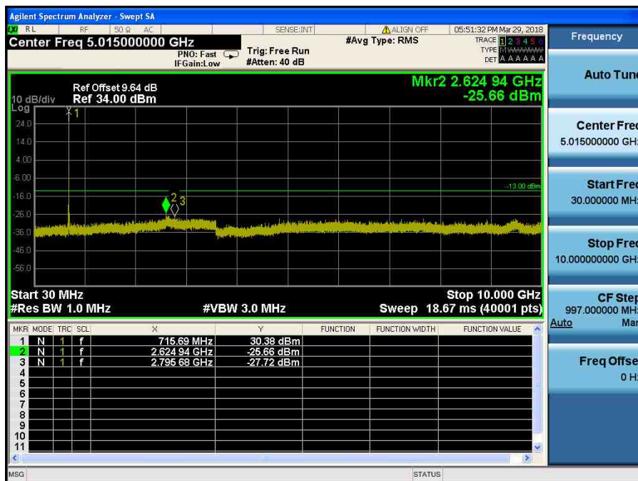
LTE Band 12,17 / 10MHz / QPSK - RB Size/Offset (1/49) – High Channel
