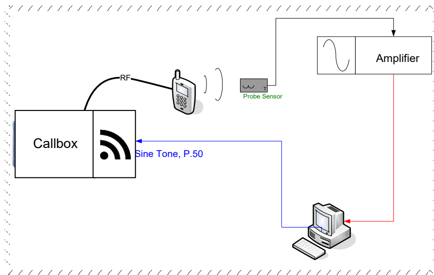
Figure 4-2 T-Coil Test Setup
