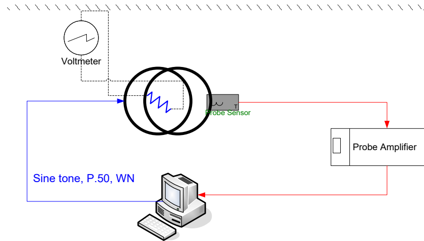
Figure 4-1 Validation Setup with Helmholtz Coil
