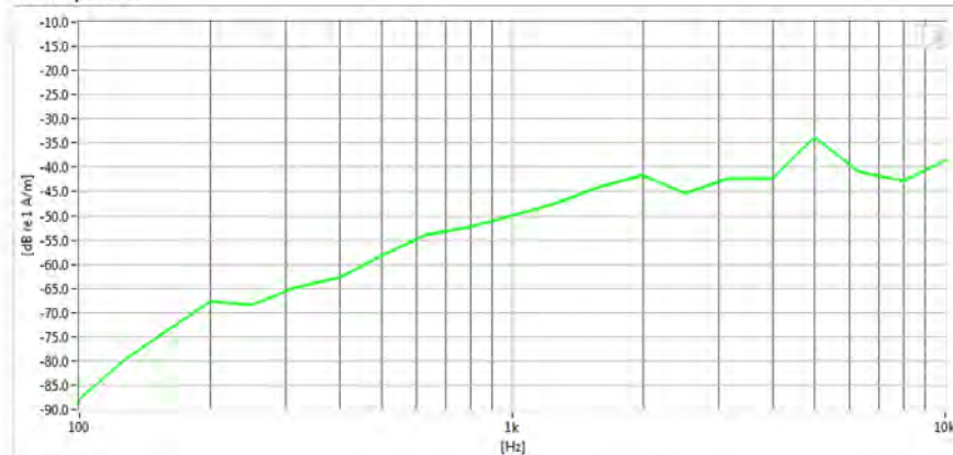
Noise Spectrum
