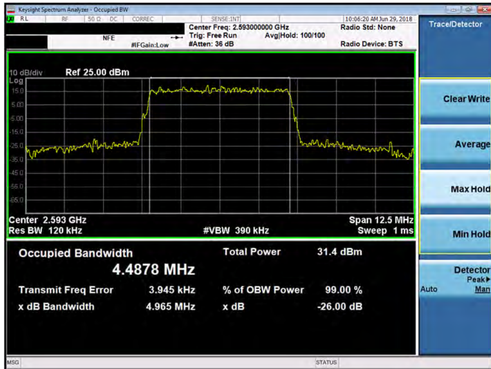
Plot 7-101. Occupied Bandwidth Plot (Band 41 - 5.0MHz 16-QAM - Full RB Configuration)
