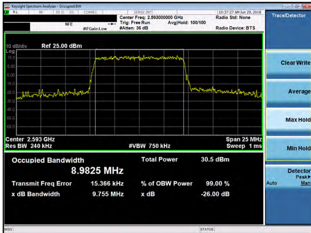
Plot 7-105. Occupied Bandwidth Plot (Band 41 - 10.0MHz 64-QAM - Full RB Configuration)
