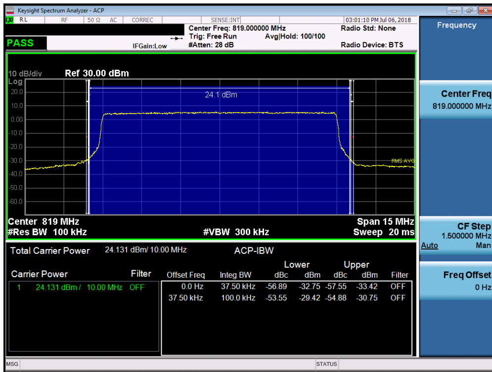
Plot 7-46. Channel Edge Plot (LTE Band 26, 10MHz QPSK – RB Size 50)
