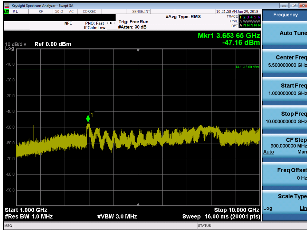
Plot 7-26. Conducted Spurious Plot (Ch. 476)
