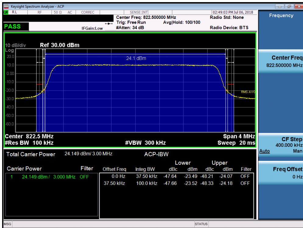
Plot 7-43. Channel Edge Plot (LTE Band 26, 3MHz QPSK – RB Size 15 – High Channel)
