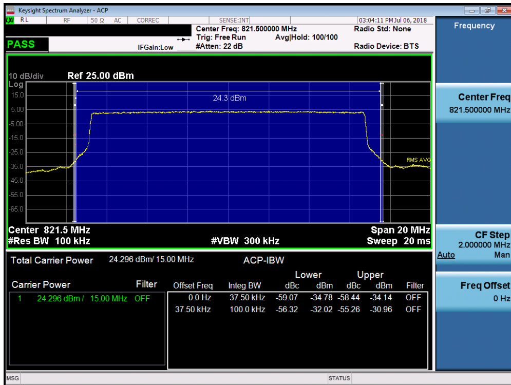
Plot 7-47. Channel Edge Plot (LTE Band 26, 15MHz QPSK – RB Size 75)
