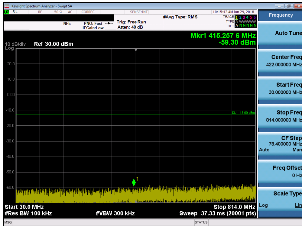
Plot 7-27. Conducted Spurious Plot (Ch. 684)
