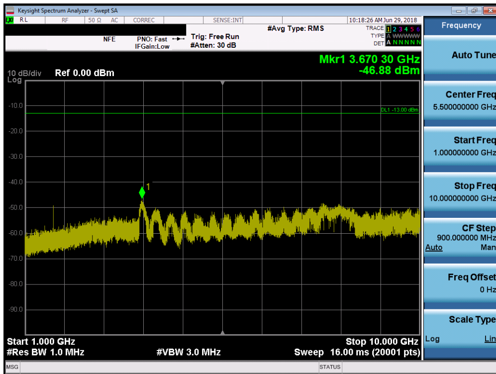
Plot 7-29. Conducted Spurious Plot (Ch. 684)
