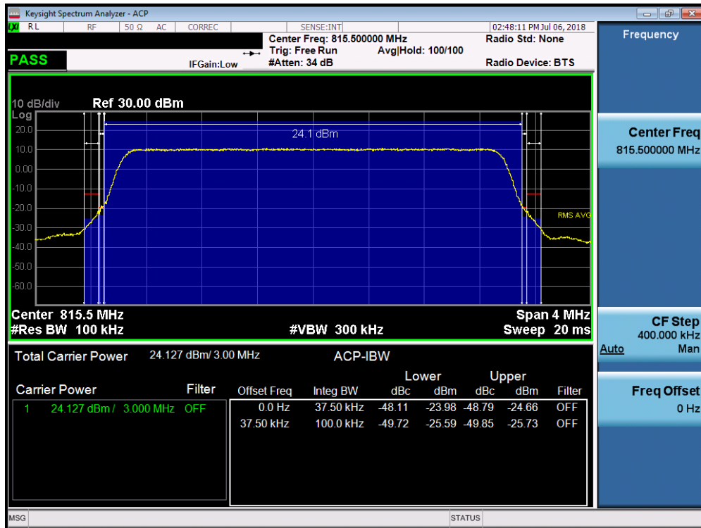
Plot 7-42. Channel Edge Plot (LTE Band 26, 3MHz QPSK – RB Size 15– Low Channel)
