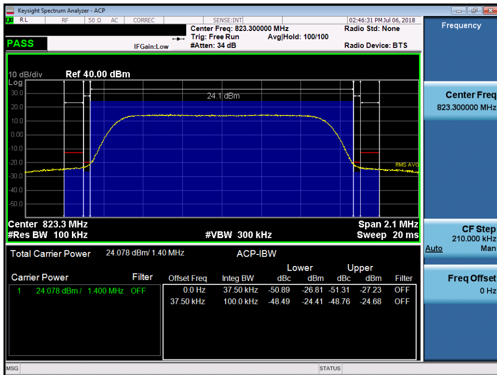
Plot 7-41. Channel Edge Plot (LTE Band 26, 1.4MHz QPSK – RB Size 6 – High Channel)
