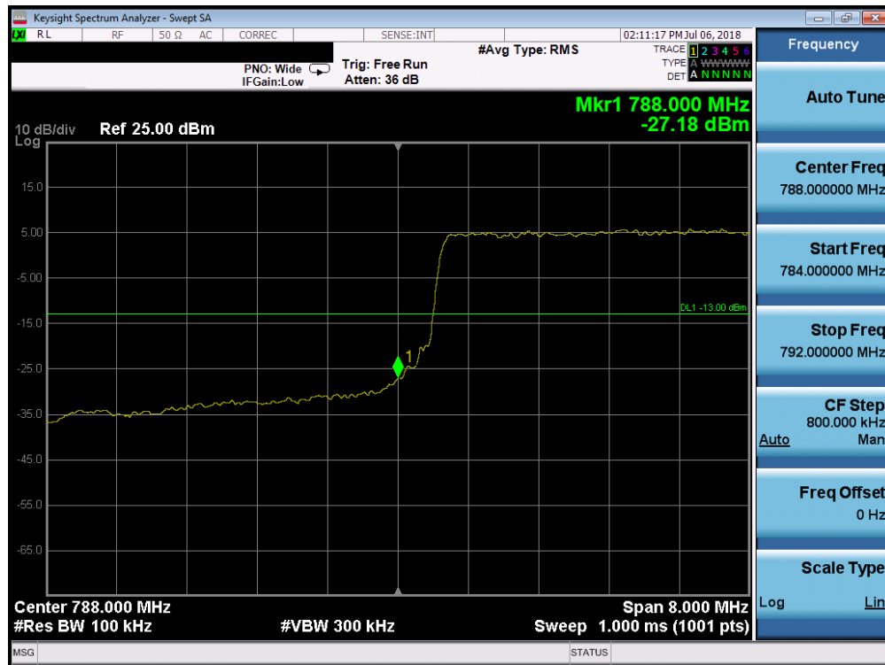
Plot 7-52. Lower Band Edge Plot (LTE Band 14, 10MHz QPSK – RB Size 50)
