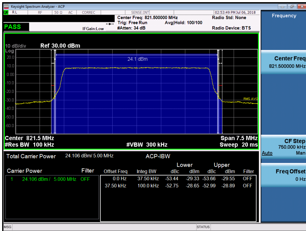
Plot 7-45. Channel Edge Plot (LTE Band 26, 5MHz QPSK – RB Size 25– High Channel)
