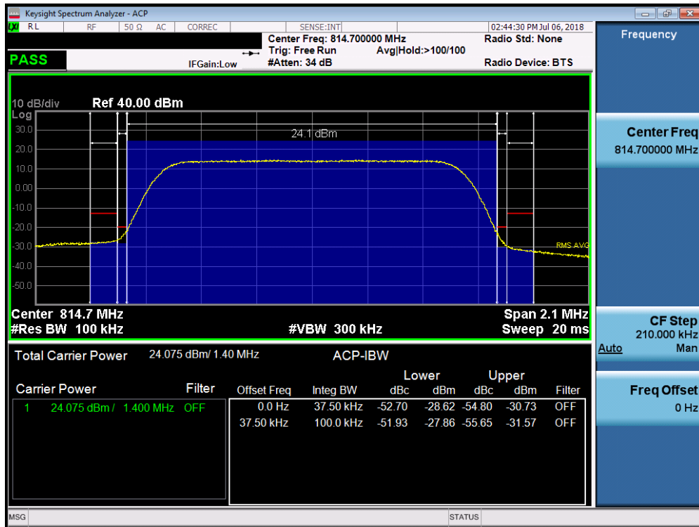
Plot 7-40. Channel Edge Plot (LTE Band 26, 1.4MHz QPSK – RB Size 6– Low Channel)
