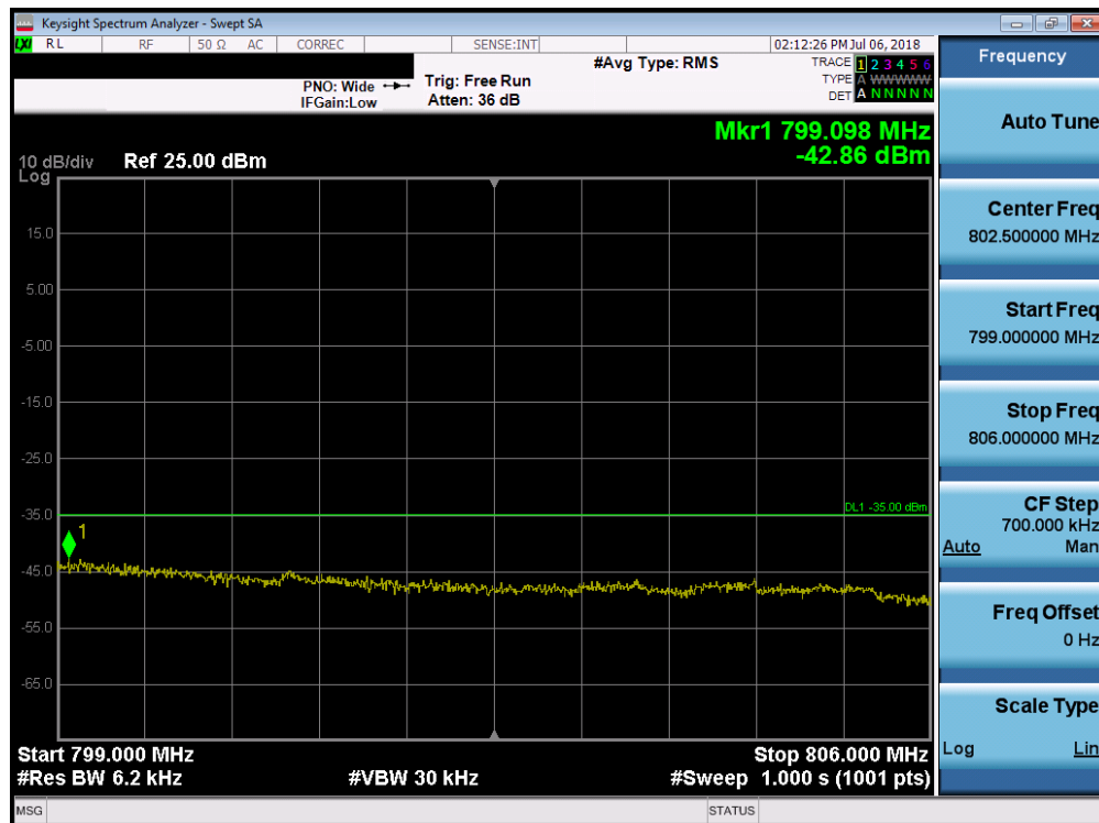
Plot 7-55. Upper Emission Mask Plot (LTE Band 14, 10MHz QPSK – RB Size 50)
