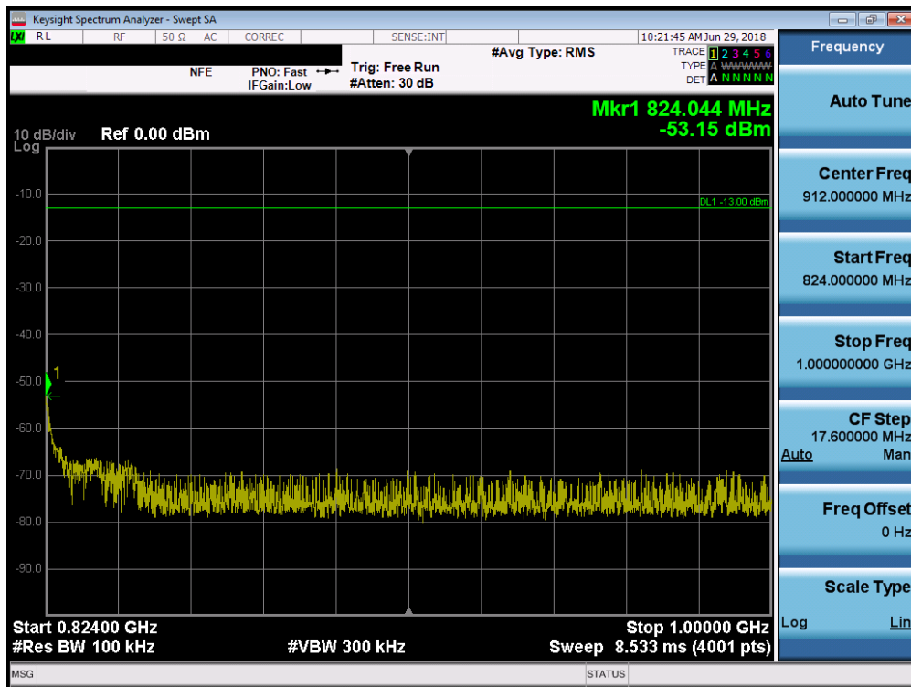
Plot 7-25. Conducted Spurious Plot (Ch. 476)
