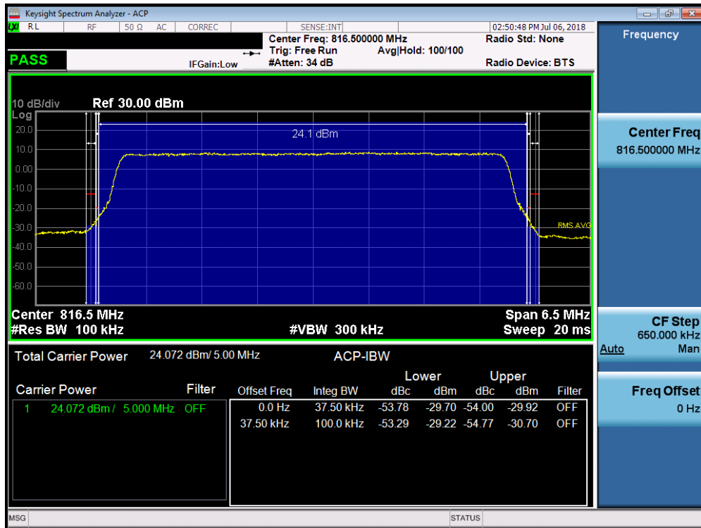
Plot 7-44. Channel Edge Plot (LTE Band 26, 5MHz QPSK – RB Size 25– Low Channel)
