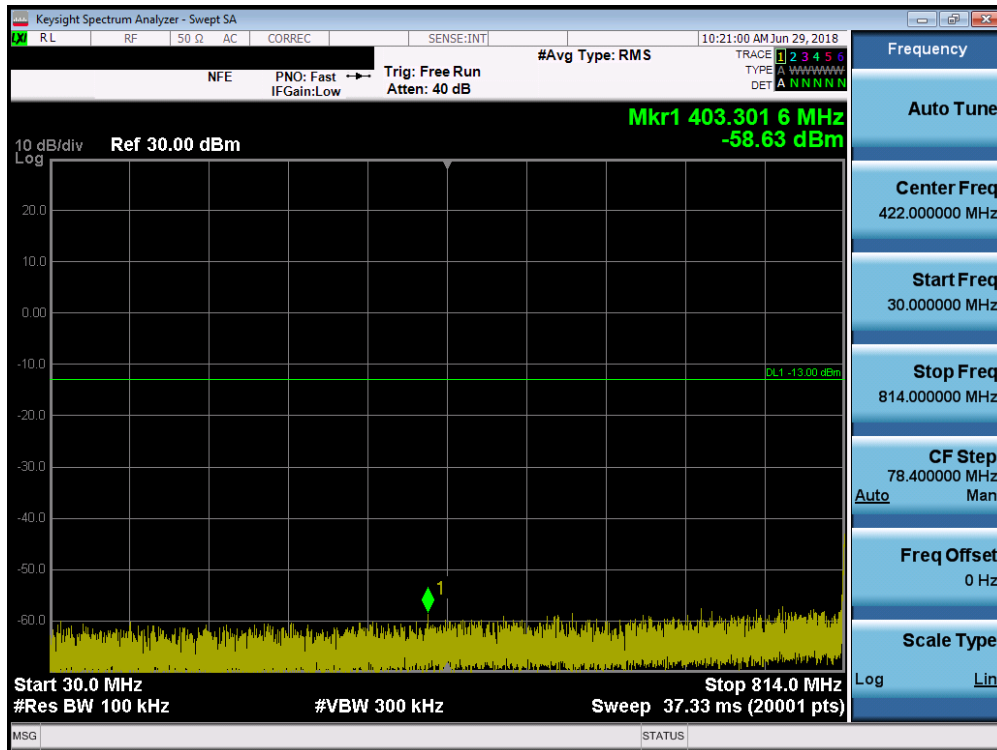
Plot 7-24. Conducted Spurious Plot (Ch. 476)
