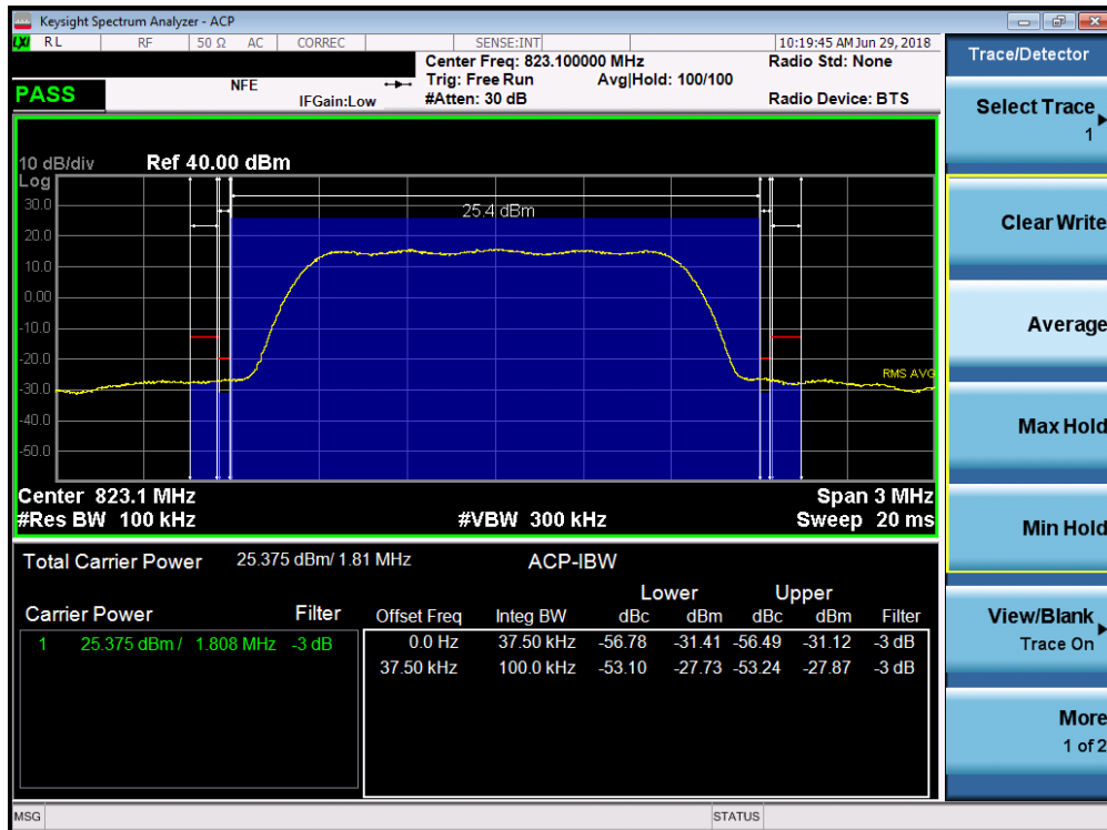
Plot 7-39. Channel Edge Plot (CDMA Ch. 684)
