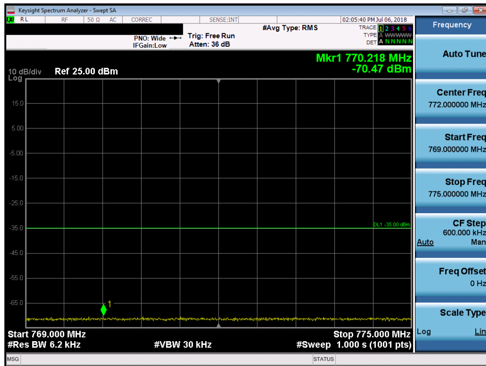
Plot 7-49. Lower Emission Mask Plot (LTE Band 14, 5MHz QPSK – RB Size 25)
