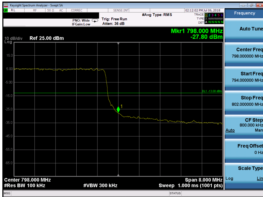
Plot 7-54. Upper Band Edge Plot (LTE Band 14, 10MHz QPSK – RB Size 50)
