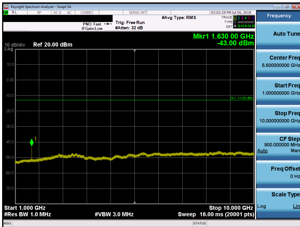
Plot 7-32. Conducted Spurious Plot (LTE Band 26, 15MHz QPSK – RB Size 1, RB Offset 0 – Mid Channel)
