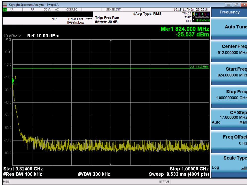
Plot 7-28. Conducted Spurious Plot (Ch. 684)
