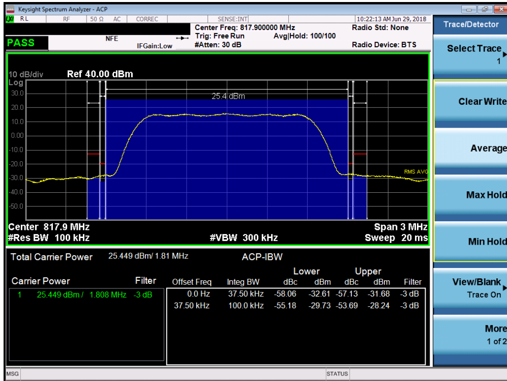
Plot 7-38. Channel Edge Plot (CDMA Ch. 476)
