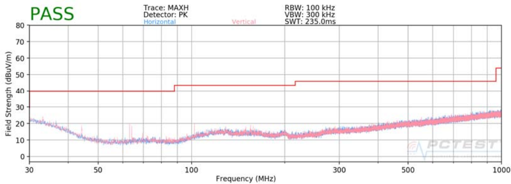
Plot 7-50. Radiated Spurious Plot below 1GHz
