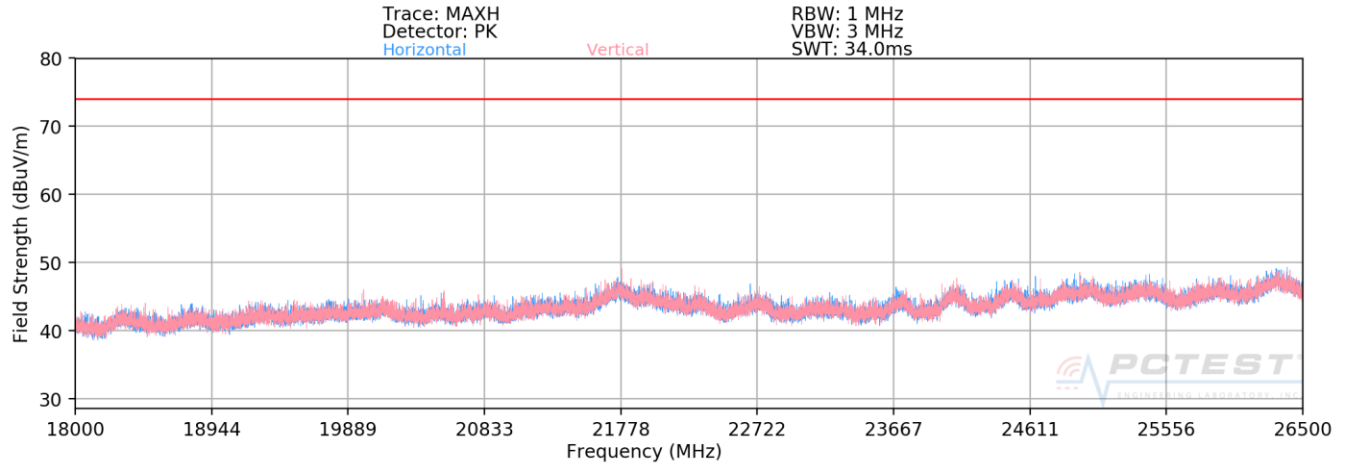
Plot 7-4. Radiated Spurious Plot above 18GHz
