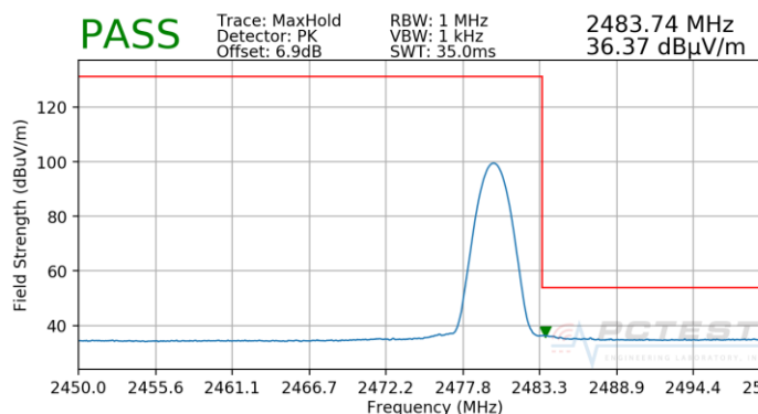
Plot 7-7. Radiated Restricted Upper Band Edge Measurement with WCP (Average)
