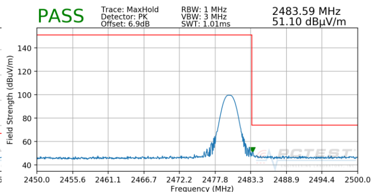
Plot 7-8. Radiated Restricted Upper Band Edge Measurement with WCP (Peak)
