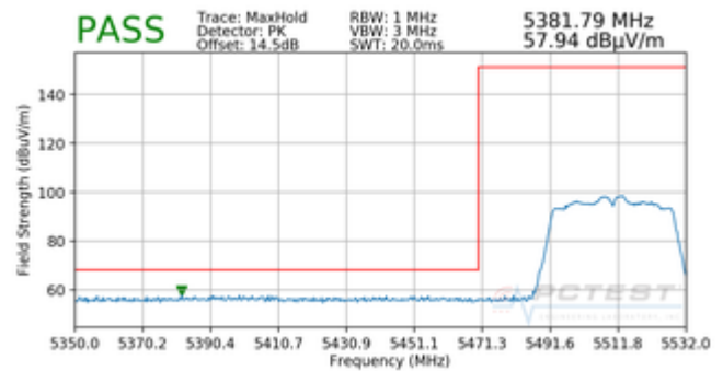
Plot 7-182. Radiated Lower Band Edge Plot (Peak – UNII Band 2C)
