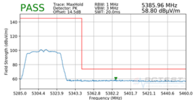
Plot 7-207. Radiated Upper Band Edge Plot (Peak – UNII Band 2A)
