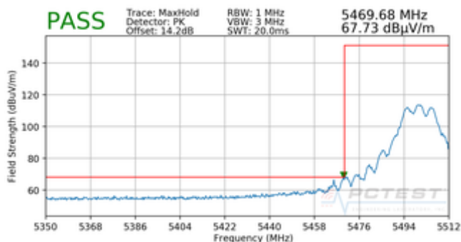
Plot 7-75. Radiated Lower Band Edge Plot (Peak – UNII Band 2C)
