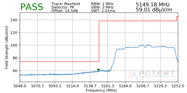
Plot 7-35. Radiated Lower Band Edge Plot SISO ANT1 (Peak – UNII Band 1)
