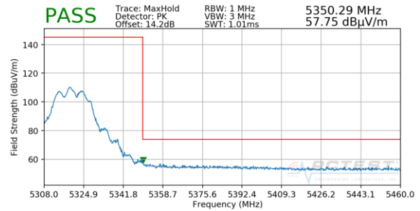
Plot 7-78. Radiated Band Edge Plot (Peak – WCP)
