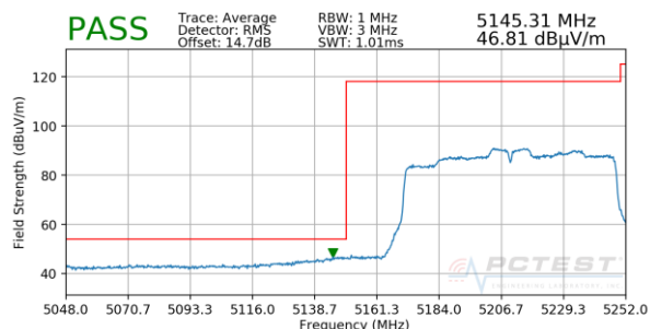
Plot 7-61. Radiated Lower Band Edge Plot SISO ANT2 (Average – UNII Band 1)
