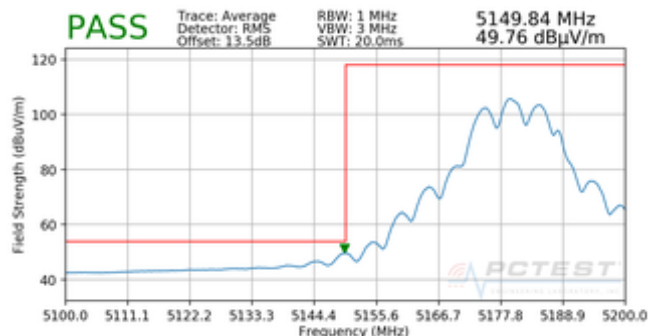
Plot 7-70. Radiated Lower Band Edge Plot (Average – UNII Band 1)
