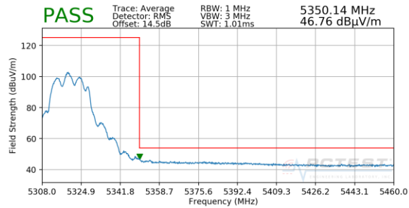
Plot 7-77. Radiated Band Edge Plot (Average – WCP)
