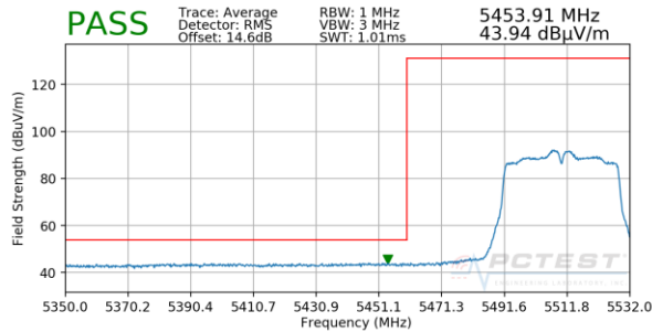
Plot 7-90. Radiated Lower Band Edge Plot MIMO (Average – UNII Band 2C)
