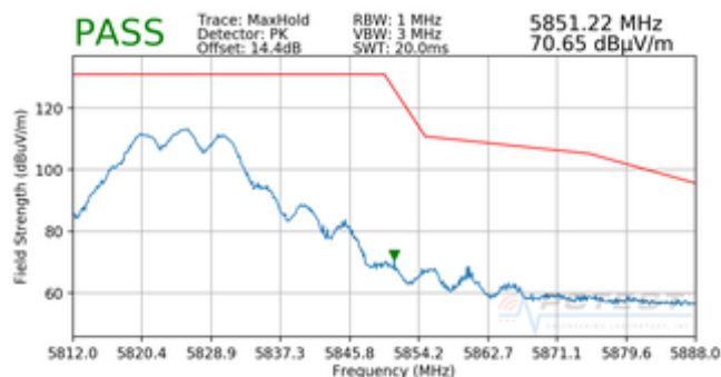
Plot 7-76. Radiated Upper Band Edge Plot (Peak – UNII Band 3)
