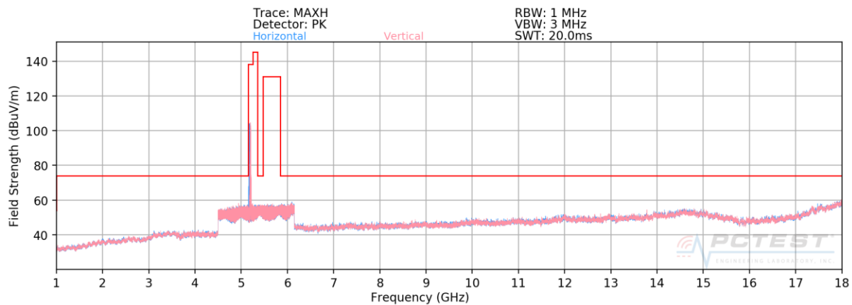
Plot 7-1. Radiated Spurious Plot above 1GHz SISO ANT1 (802.11a – U1 Ch. 40)
