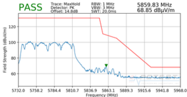
Plot 7-101. Radiated Upper Band Edge Plot MIMO (Peak – UNII Band 3)
