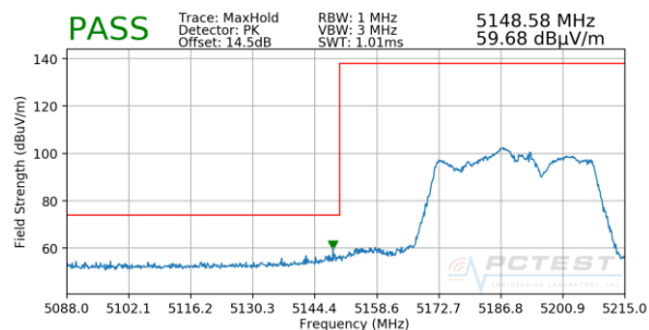
Plot 7-94. Radiated Band Edge Plot ANT (Peak – WCP)
