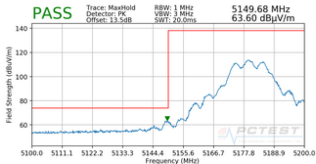
Plot 7-71. Radiated Lower Band Edge Plot (Peak – UNII Band 1)
