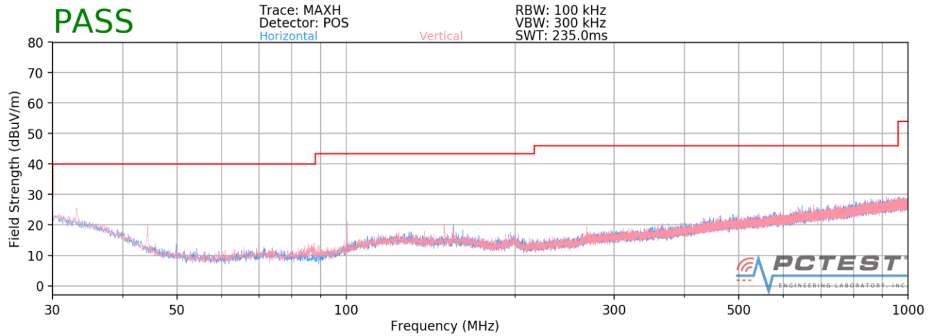
Plot 7-104. Radiated Spurious Plot below 1GHz SISO ANT1 (802.11a – U3 Ch. 157)
