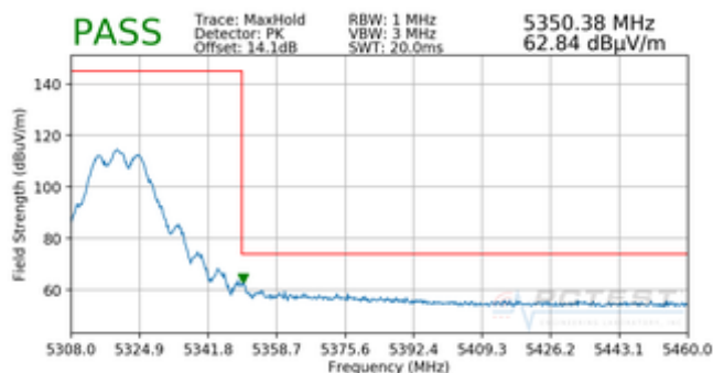
Plot 7-73. Radiated Upper Band Edge Plot (Peak – UNII Band 2A)
