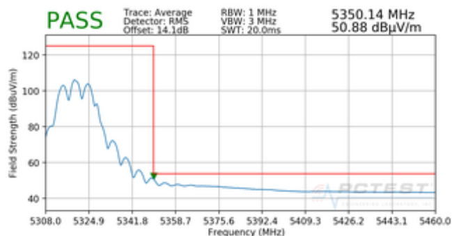
Plot 7-72. Radiated Upper Band Edge Plot (Average – UNII Band 2A)
