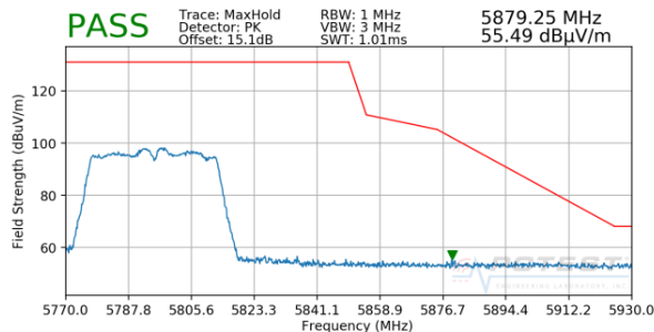
Plot 7-92. Radiated Upper Band Edge Plot MIMO (Peak – UNII Band 3)
