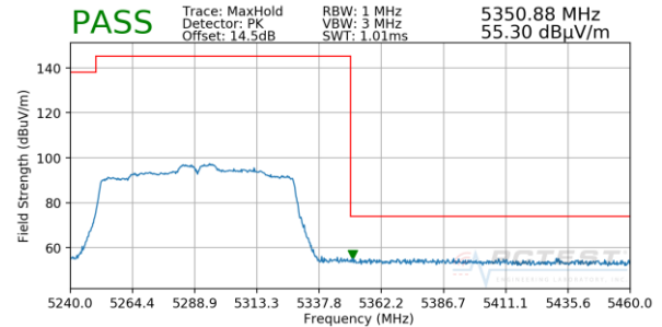
Plot 7-37. Radiated Upper Band Edge Plot SISO ANT1 (Peak – UNII Band 2A)
