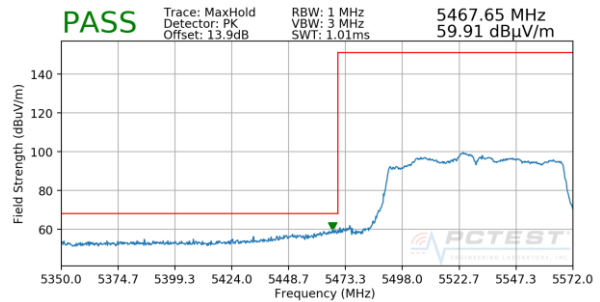
Plot 7-103. Radiated Band Edge Plot MIMO (Peak – WCP)
