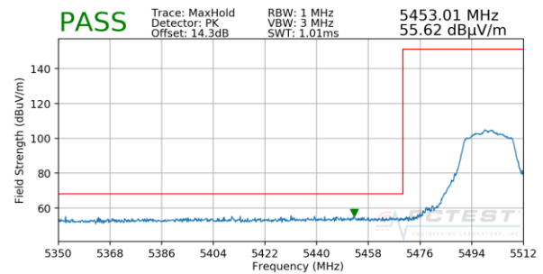
Plot 7-48. Radiated Lower Band Edge Plot SISO ANT2 (Peak – UNII Band 2C)
