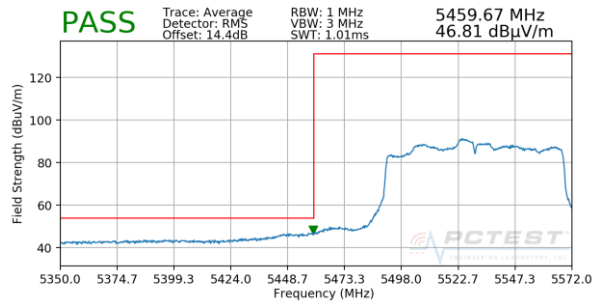
Plot 7-102. Radiated Band Edge Plot MIMO (Average – WCP)
