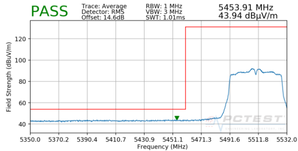
Plot 7-56. Radiated Lower Band Edge Plot SISO ANT2 (Average - UNII Band 2C)
