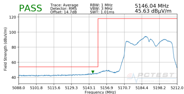
Plot 7-93. Radiated Band Edge Plot ANT (Average – WCP)
