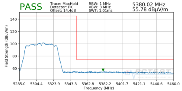
Plot 7-89. Radiated Upper Band Edge Plot MIMO (Peak – UNII Band 2A)
