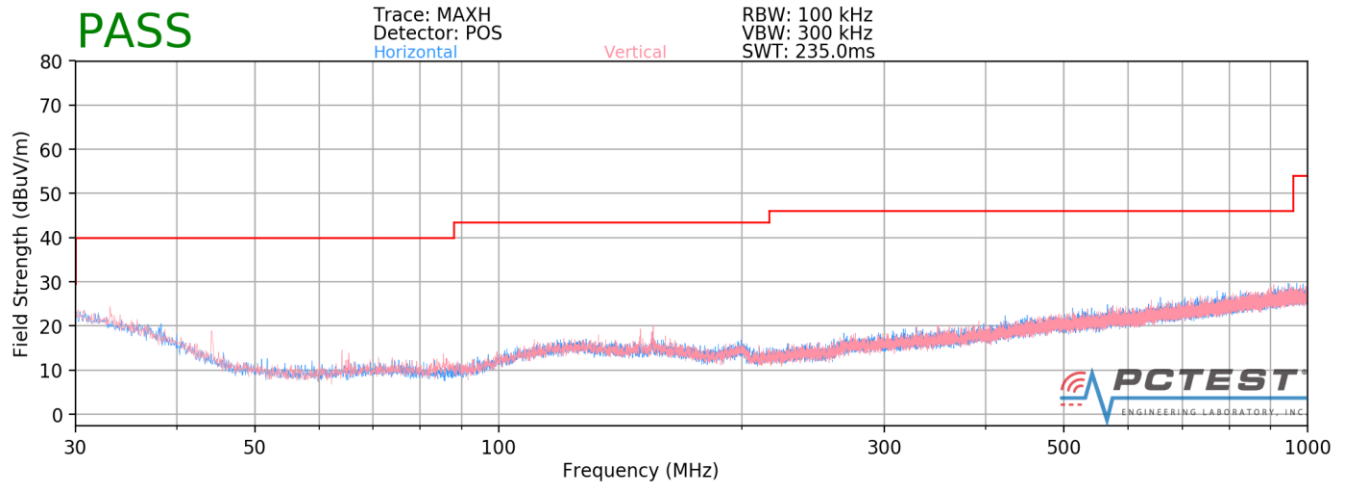
Plot 7-105. Radiated Spurious Plot below 1GHz SISO ANT2 (802.11a – U3 Ch. 157)
