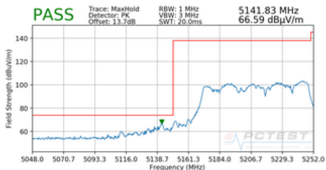
Plot 7-96. Radiated Lower Band Edge Plot MIMO (Peak – UNII Band 1)
