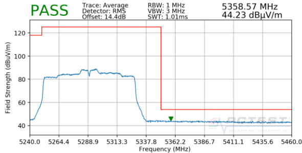
Plot 7-36. Radiated Upper Band Edge Plot SISO ANT1 (Average – UNII Band 2A)
