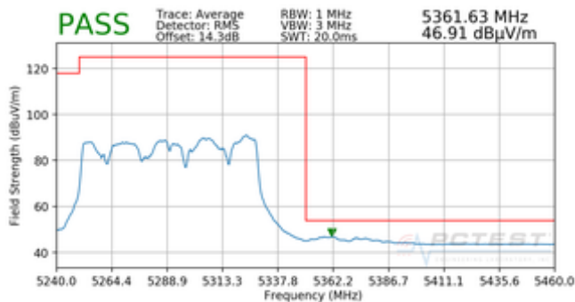
Plot 7-97. Radiated Upper Band Edge Plot MIMO (Average – UNII Band 2A)
