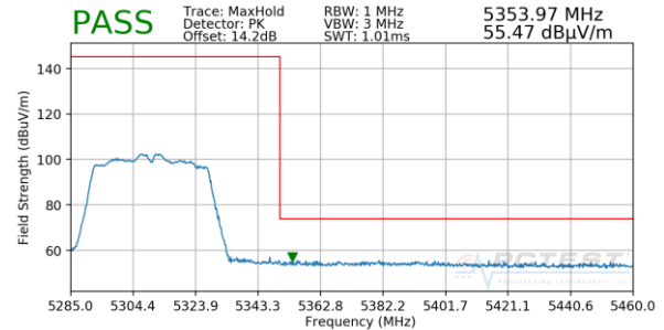
Plot 7-28. Radiated Upper Band Edge Plot SISO ANT1 (Peak – UNII Band 2A)
