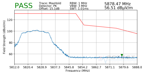
Plot 7-49. Radiated Upper Band Edge Plot SISO ANT2 (Peak – UNII Band 3)
