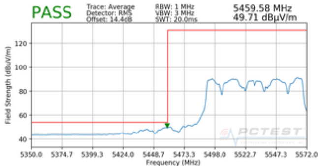
Plot 7-99. Radiated Lower Band Edge Plot MIMO (Average – UNII Band 2C)
