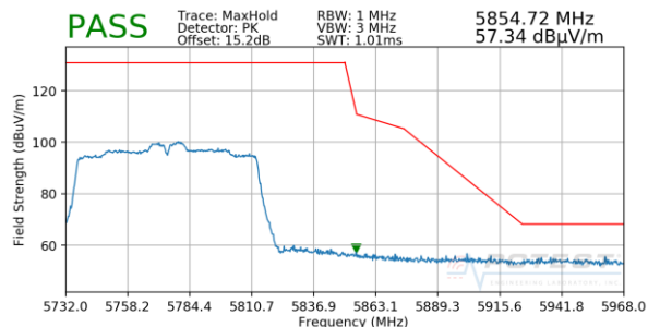
Plot 7-40. Radiated Upper Band Edge Plot SISO ANT1 (Peak - UNII Band 3)
