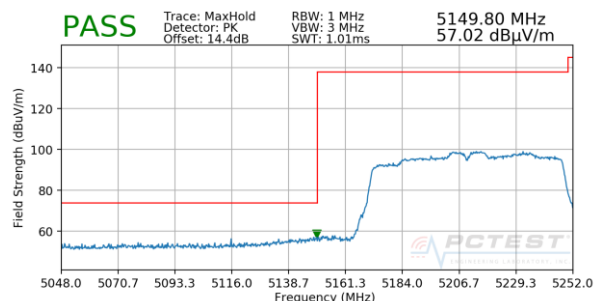
Plot 7-62. Radiated Lower Band Edge Plot SISO ANT2 (Peak – UNII Band 1)
