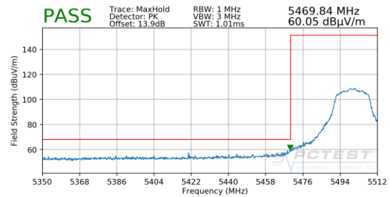
Plot 7-21. Radiated Lower Band Edge Plot SISO ANT1 (Peak – UNII Band 2C)
