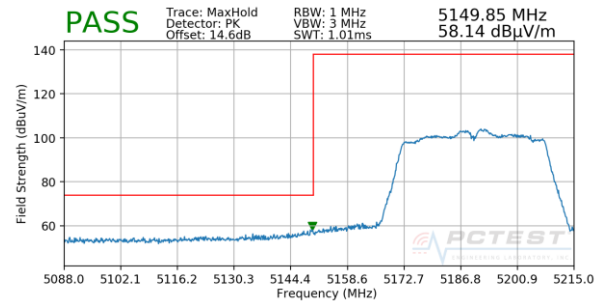
Plot 7-26. Radiated Lower Band Edge Plot SISO ANT1 (Peak – UNII Band 1)
