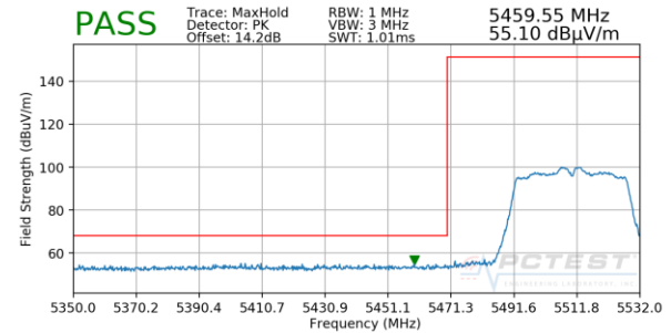
Plot 7-91. Radiated Lower Band Edge Plot MIMO (Peak – UNII Band 2C)
