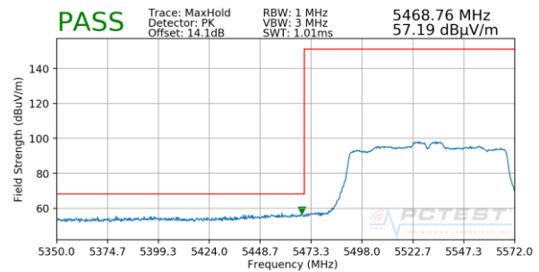
Plot 7-66. Radiated Lower Band Edge Plot SISO ANT2 (Peak – UNII Band 2C)
