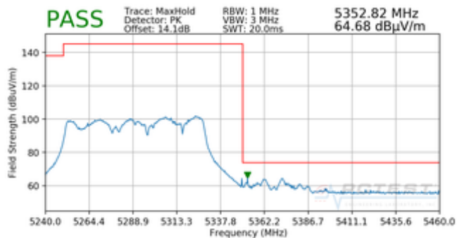
Plot 7-98. Radiated Upper Band Edge Plot MIMO (Peak – UNII Band 2A)
