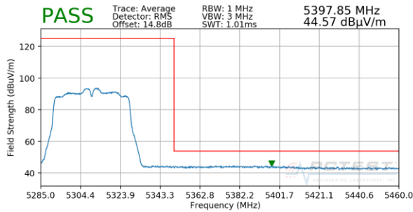
Plot 7-88. Radiated Upper Band Edge Plot MIMO (Average – UNII Band 2A)
