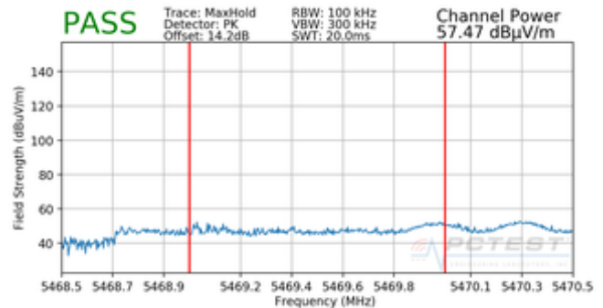
Plot 7-100. Radiated Lower Band Edge Plot MIMO (Peak – UNII Band 2C)
