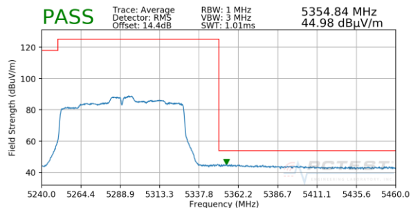
Plot 7-63. Radiated Upper Band Edge Plot SISO ANT2 (Average – UNII Band 2A)
