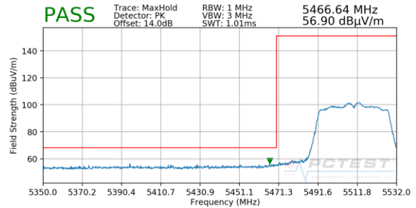
Plot 7-30. Radiated Lower Band Edge Plot SISO ANT1 (Peak – UNII Band 2C)
