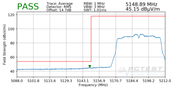
Plot 7-86. Radiated Lower Band Edge Plot MIMO (Average – UNII Band 1)
