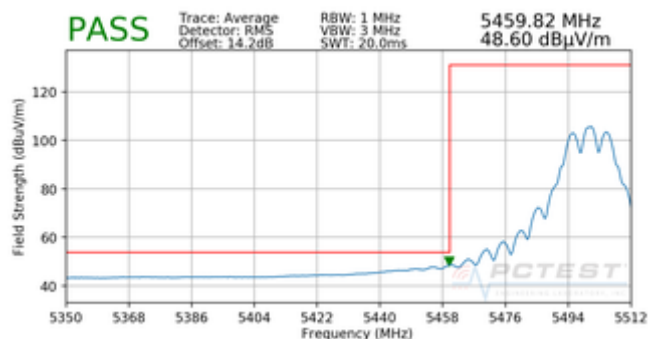
Plot 7-74. Radiated Lower Band Edge Plot (Average – UNII Band 2C)
