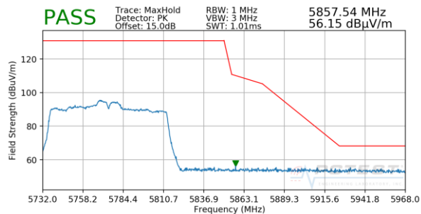
Plot 7-67. Radiated Upper Band Edge Plot SISO ANT2 (Peak – UNII Band 3)
