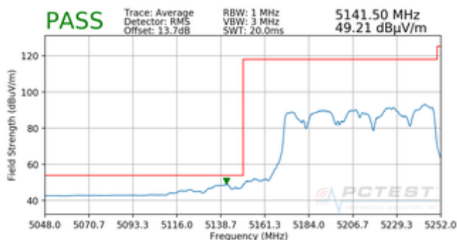
Plot 7-95. Radiated Lower Band Edge Plot MIMO (Average – UNII Band 1)
