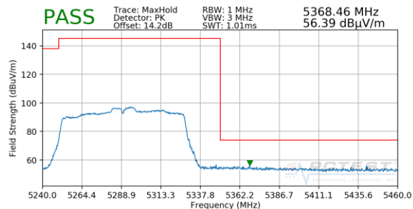
Plot 7-64. Radiated Upper Band Edge Plot SISO ANT2 (Peak – UNII Band 2A)
