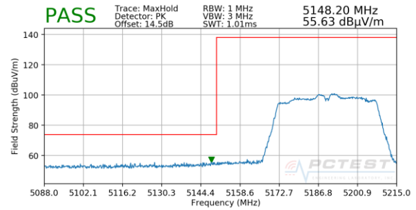
Plot 7-87. Radiated Lower Band Edge Plot MIMO (Peak – UNII Band 1)
