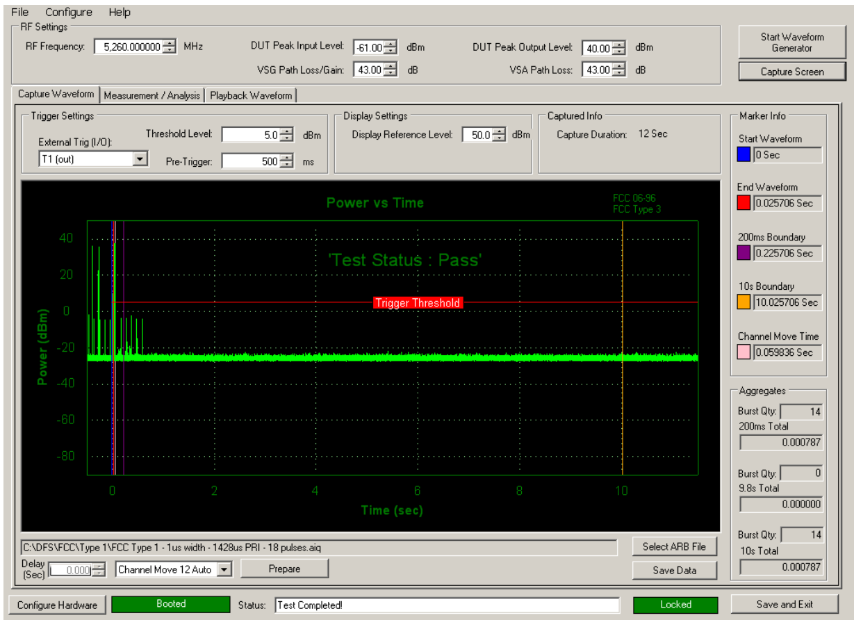
Figure 5-1. Band 2A Move Time and Aggregate Time
