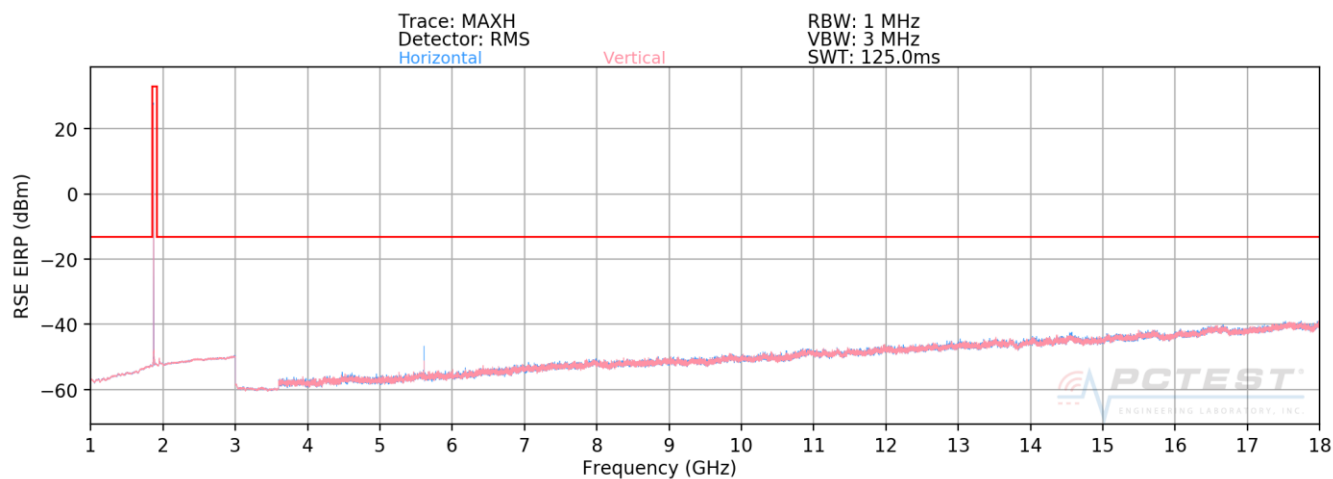
Plot 7-5. Radiated Spurious Plot above 1GHz (PCS GPRS Mode)
