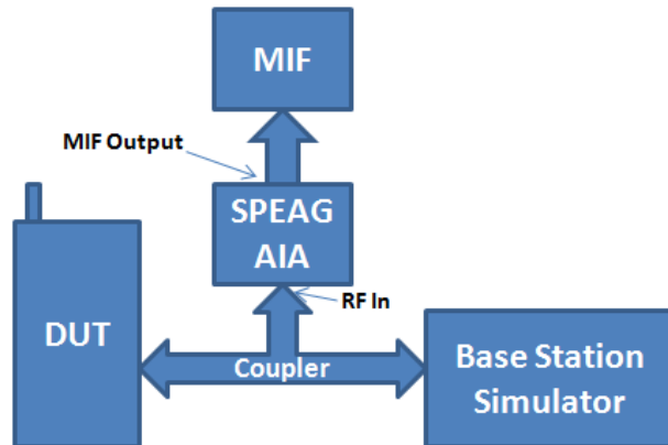
Figure 7-1 MIF Measurement Setup for licensed modes
