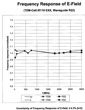
Figure 4-2 E-Field Probe Frequency Response
