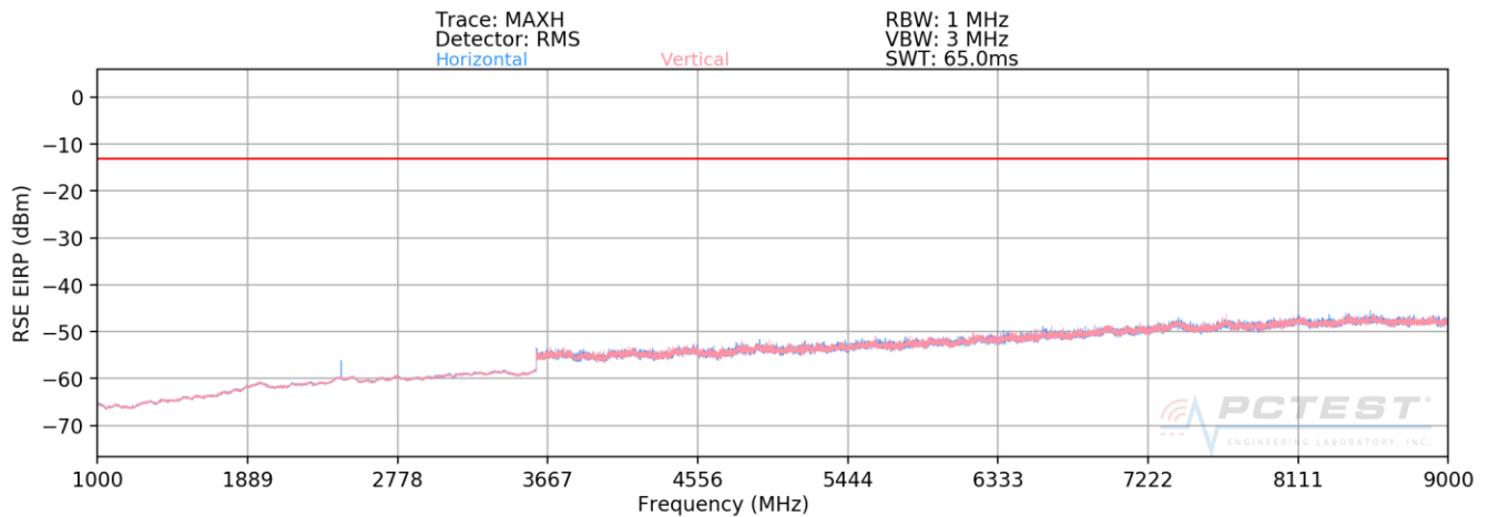
Plot 7-3. Radiated Spurious Plot above 1GHz (Band 26, Pt. 90)
