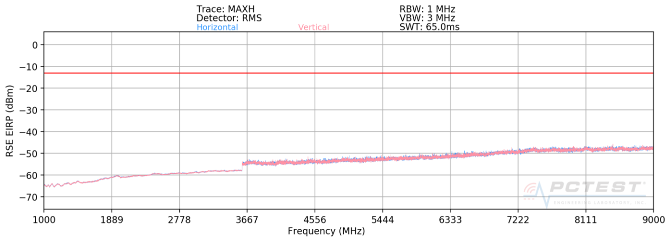
Plot 7-2. Radiated Spurious Plot above 1GHz (CDMA, Pt. 90)
