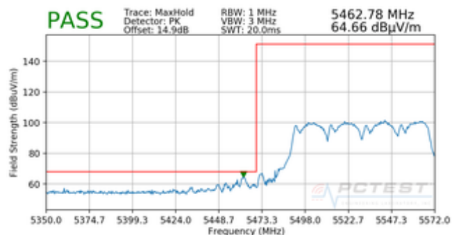
Plot 7-102. Radiated Lower Band Edge Plot MIMO (Peak – UNII Band 2C)
