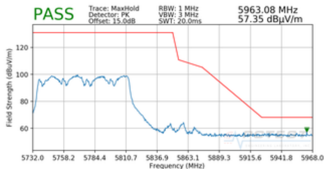
Plot 7-103. Radiated Upper Band Edge Plot MIMO (Peak – UNII Band 3)
