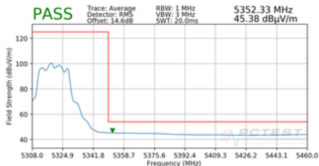
Plot 7-77. Radiated Band Edge Plot CDD (Average – WCP)
