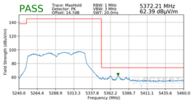
Plot 7-105. Radiated Band Edge Plot ANT (Peak – WCP)
