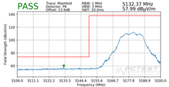
Plot 7-71. Radiated Lower Band Edge Plot CDD (Peak – UNII Band 1)
