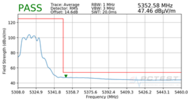
Plot 7-72. Radiated Upper Band Edge Plot CDD (Average – UNII Band 2A)
