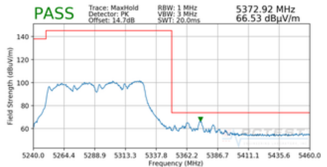
Plot 7-100. Radiated Upper Band Edge Plot MIMO (Peak – UNII Band 2A)
