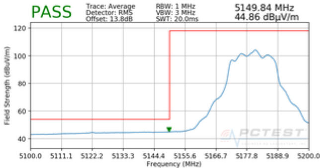
Plot 7-70. Radiated Lower Band Edge Plot CDD (Average – UNII Band 1)
