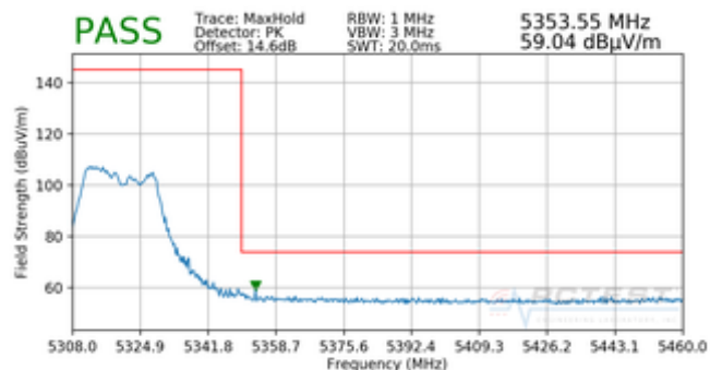
Plot 7-87. Radiated Band Edge Plot MIMO (Peak – WCP)
