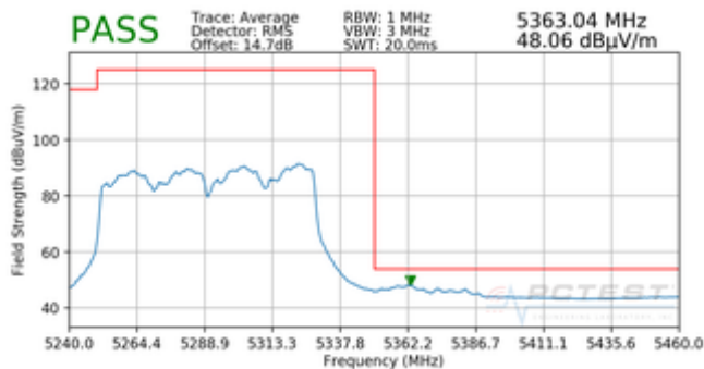
Plot 7-99. Radiated Upper Band Edge Plot MIMO (Average – UNII Band 2A)
