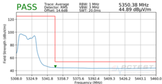
Plot 7-86. Radiated Band Edge Plot MIMO (Average – WCP)
