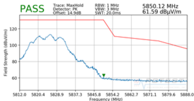
Plot 7-76. Radiated Upper Band Edge Plot CDD (Peak – UNII Band 3)
