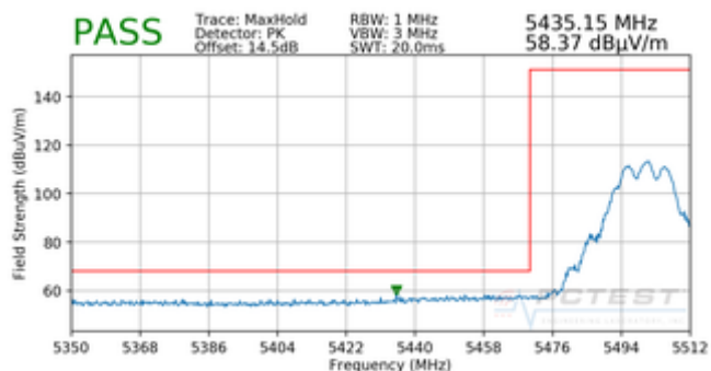
Plot 7-75. Radiated Lower Band Edge Plot CDD (Peak – UNII Band 2C)
