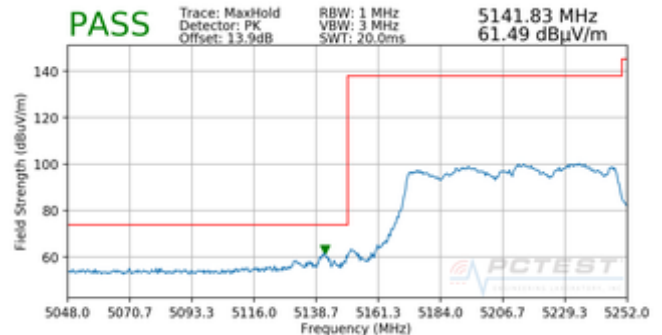
Plot 7-98. Radiated Lower Band Edge Plot MIMO (Peak – UNII Band 1)
