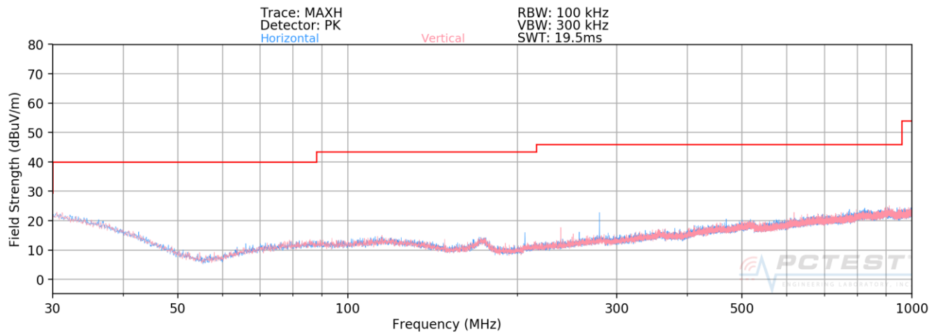
Plot 7-108. Radiated Spurious Plot below 1GHz (2.4GHz – 5GHz)
