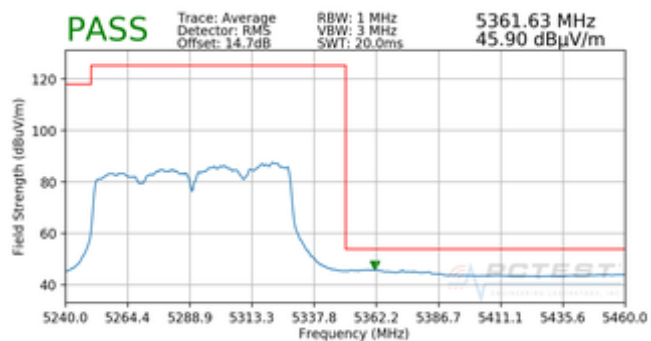
Plot 7-104. Radiated Band Edge Plot ANT (Average – WCP)
