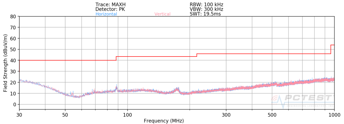
Plot 7-107. Radiated Spurious Plot below 1GHz SISO ANT2 (802.11a – U3 Ch. 157)
