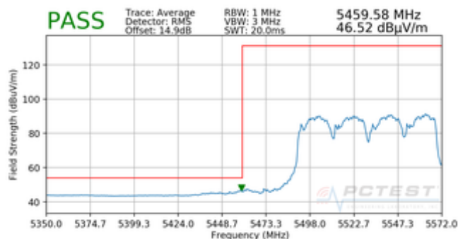
Plot 7-101. Radiated Lower Band Edge Plot MIMO (Average – UNII Band 2C)
