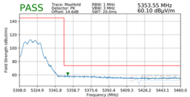
Plot 7-73. Radiated Upper Band Edge Plot CDD (Peak – UNII Band 2A)
