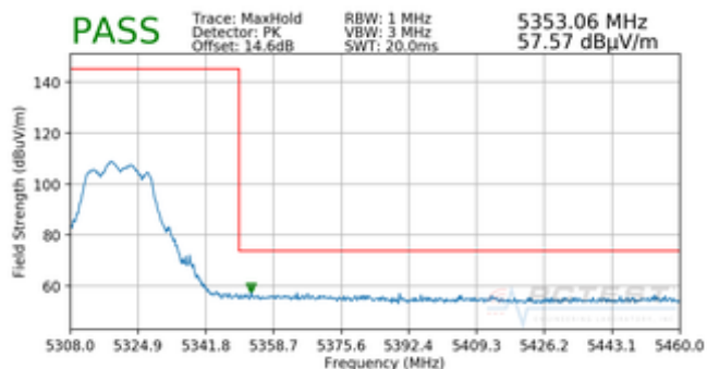
Plot 7-78. Radiated Band Edge Plot CDD (Peak – WCP)
