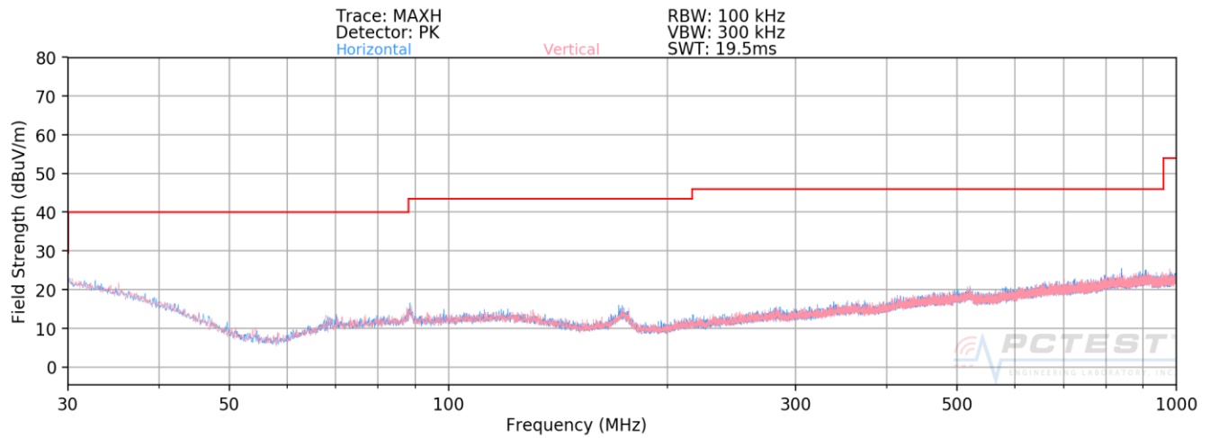
Plot 7-106. Radiated Spurious Plot below 1GHz SISO ANT1 (802.11a – U3 Ch. 157)
