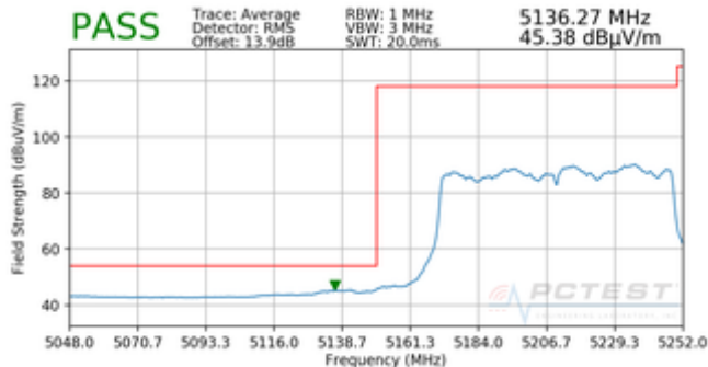
Plot 7-97. Radiated Lower Band Edge Plot MIMO (Average – UNII Band 1)
