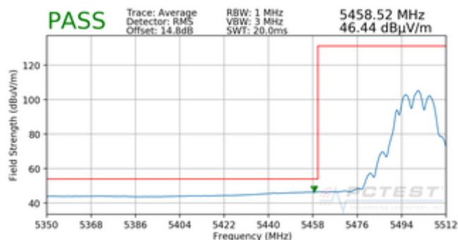
Plot 7-74. Radiated Lower Band Edge Plot CDD (Average – UNII Band 2C)
