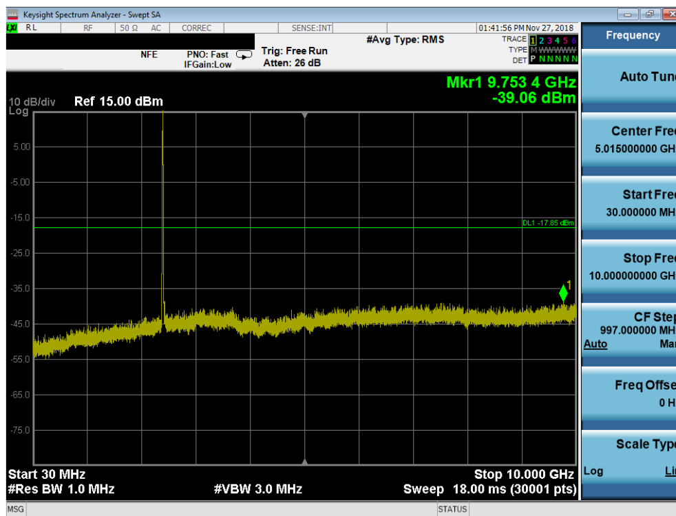
Plot 7-55. Conducted Spurious Plot SISO ANT2 (802.11b – Ch. 1)
