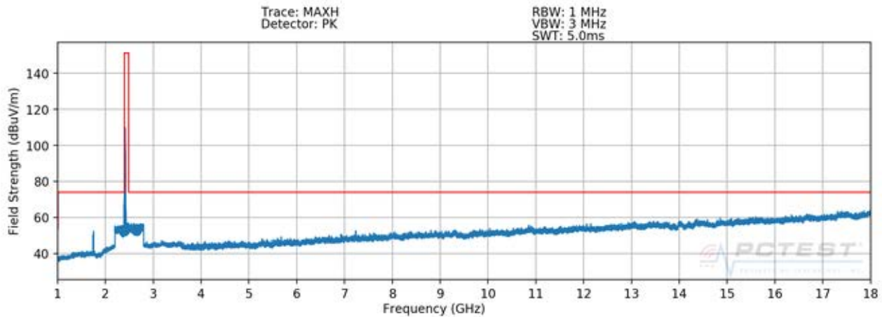
Plot 7-61. Radiated Spurious Plot above 1GHz SISO ANT1 (802.11b – Ch. 1)
