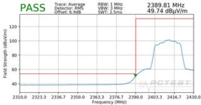
Plot 7-85. Radiated Restricted Band Edge Measurement MIMO with WCP (Average)
