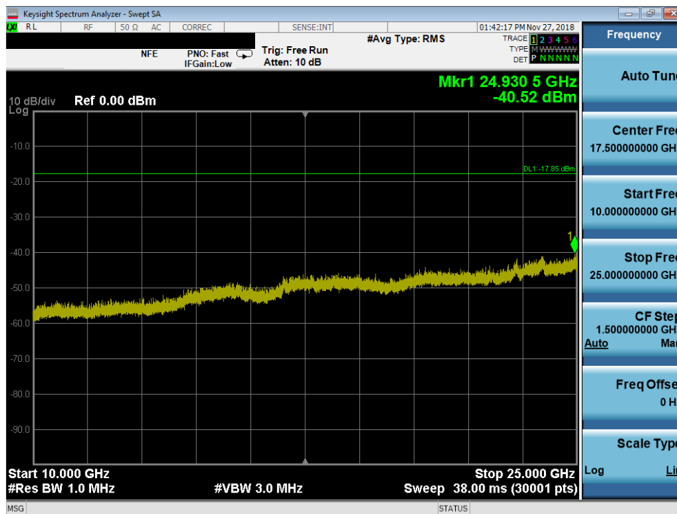
Plot 7-56. Conducted Spurious Plot SISO ANT2 (802.11b – Ch. 1)
