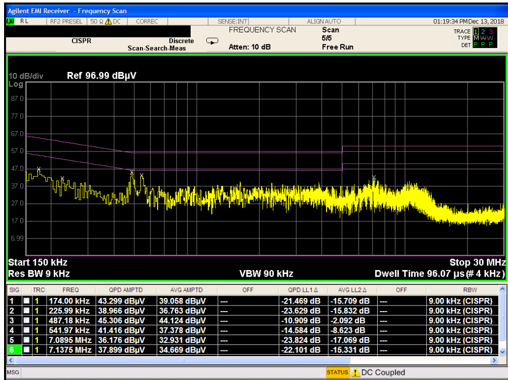
Plot 7-89. Line Conducted Plot with 802.11b (L1)
