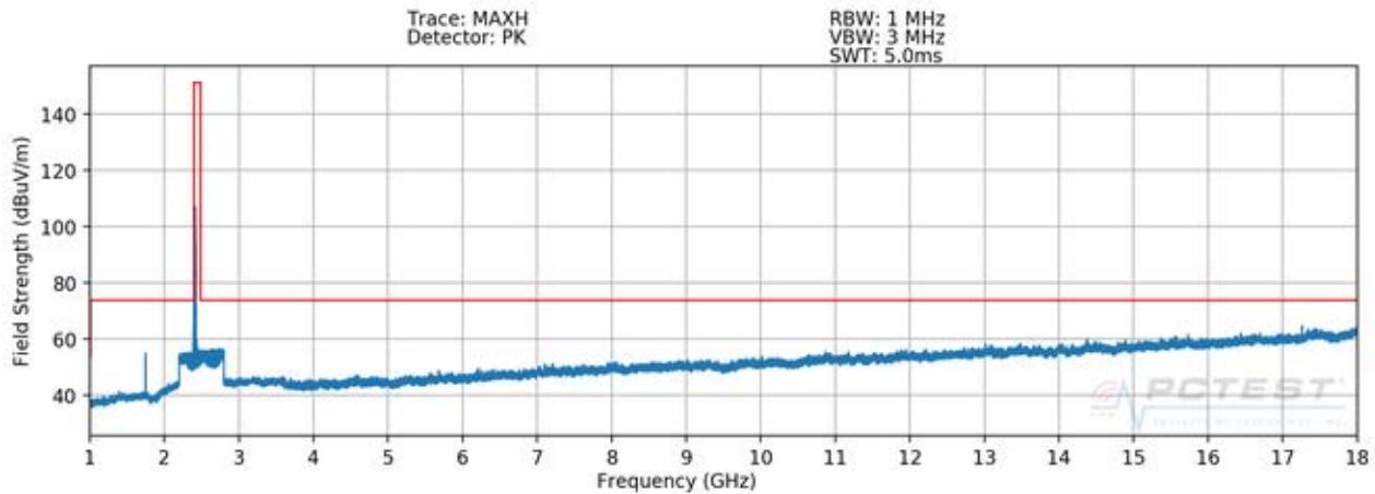
Plot 7-65. Radiated Spurious Plot above 1GHz SISO ANT2 (802.11b – Ch. 1)
