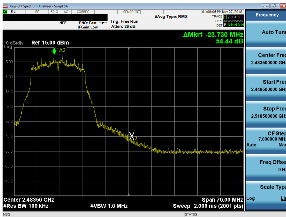
Plot 7-40. Band Edge Plot SISO ANT1 (802.11g - Ch. 11)
