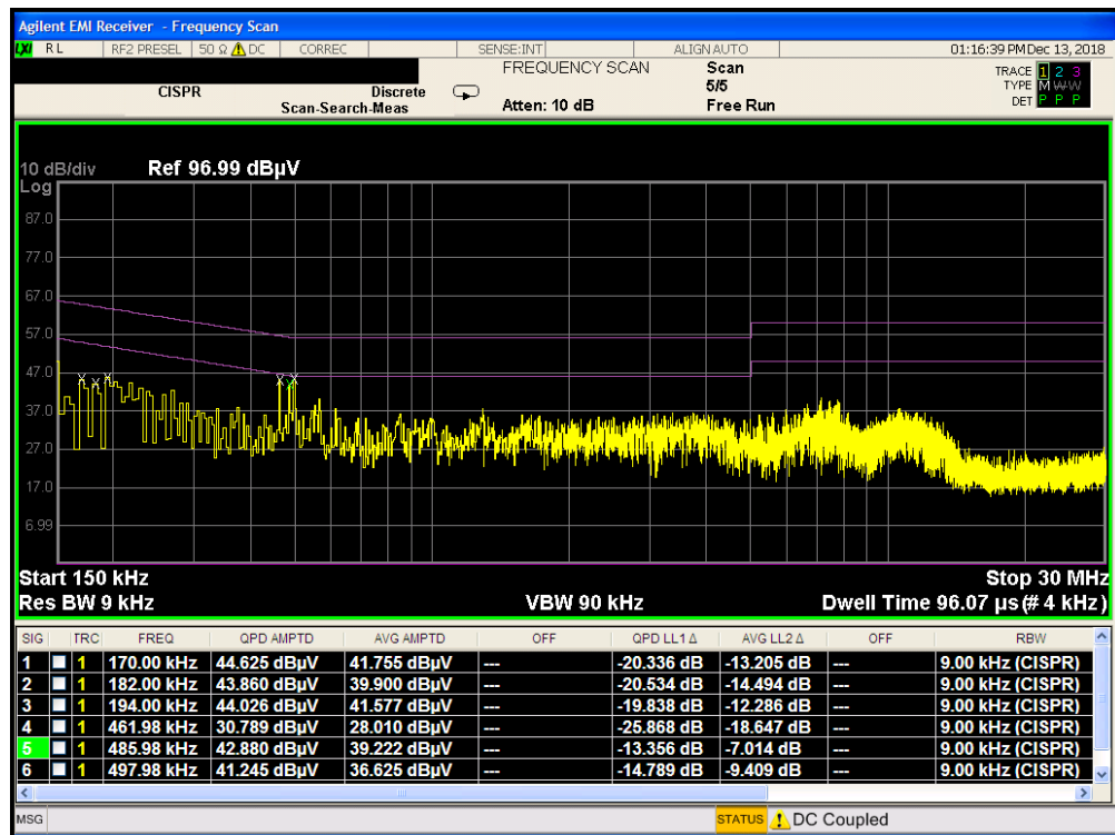
Plot 7-90. Line Conducted Plot with 802.11b (N)
