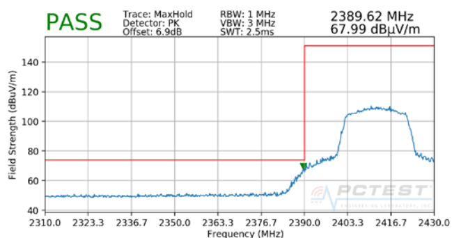
Plot 7-82. Radiated Restricted Lower Band Edge Measurement MIMO (Peak)
