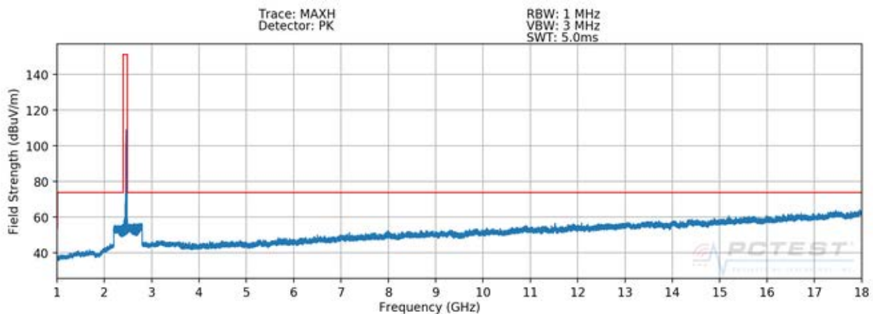
Plot 7-67. Radiated Spurious Plot above 1GHz SISO ANT2 (802.11b – Ch. 11)
