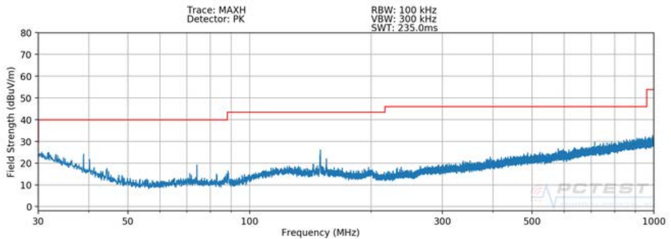
Plot 7-87. Radiated Spurious Plot below 1GHz SISO ANT1
