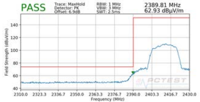
Plot 7-86. Radiated Restricted Band Edge Measurement MIMO with WCP (Peak)
