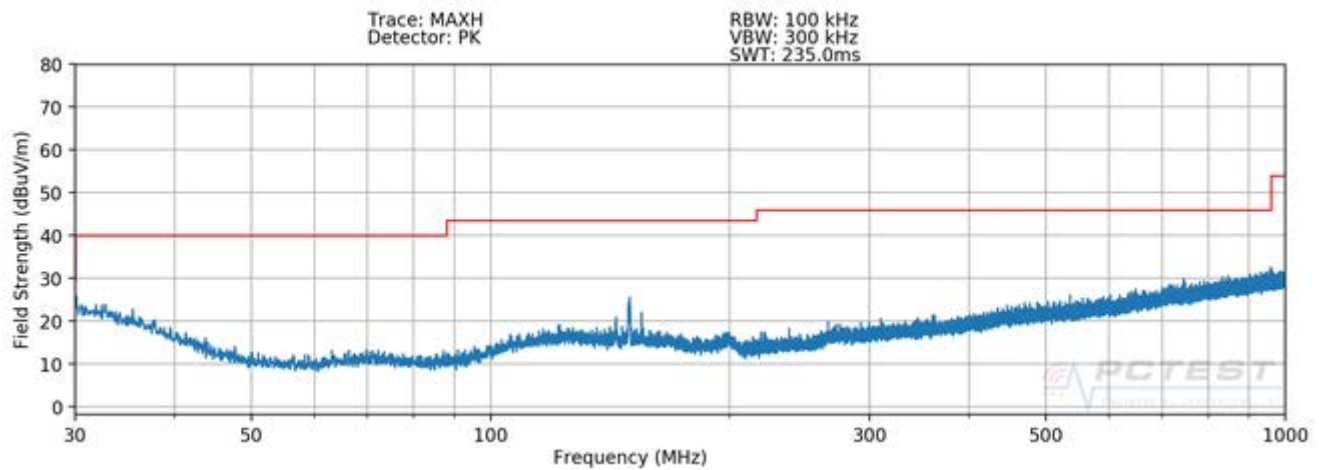
Plot 7-88. Radiated Spurious Plot below 1GHz SISO ANT2
