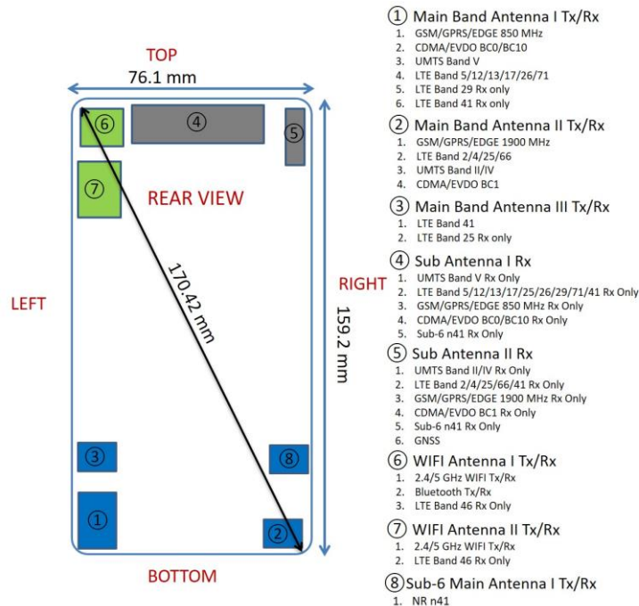
Figure F-1 DUT Antenna Locations
