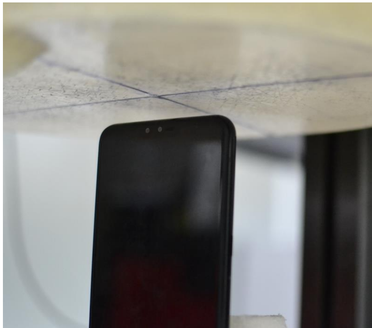
SAR Test Setup Photo 14 – Top Edge at 10mm
