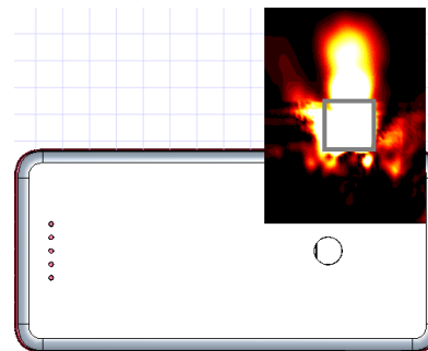
(b) Simulation(0mm)
