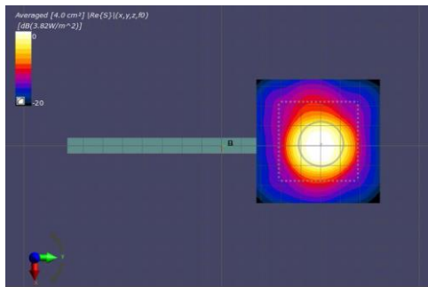
(a) Measurement(2mm)
