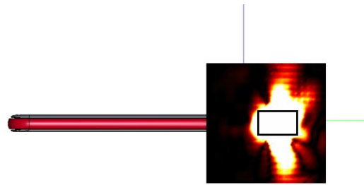
(b) Simulation(0mm)
