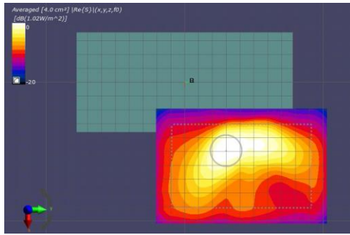
(a) Measurement(2mm)
