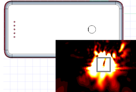
(b) Simulation(0mm)
