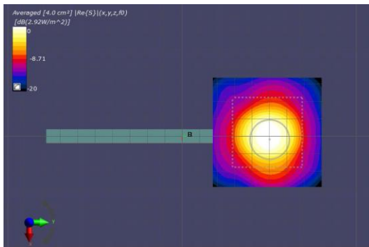
(a) Measurement(2mm)
