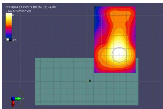
(a) Measurement(2mm)
