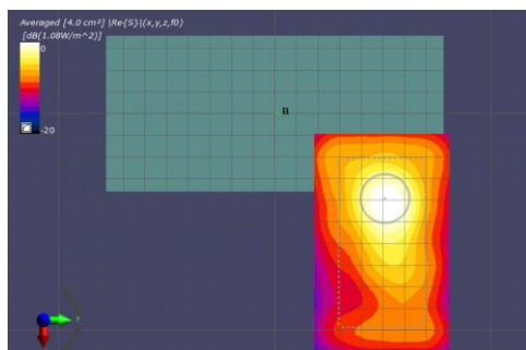
(a) Measurement(2mm)
