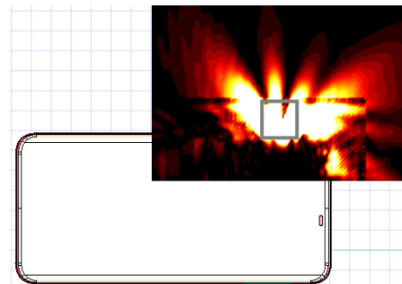
(b) Simulation(0mm)
