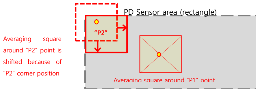
Fig 5.9 PD averaging algorithm
