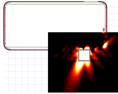
(b) Simulation(0mm)
