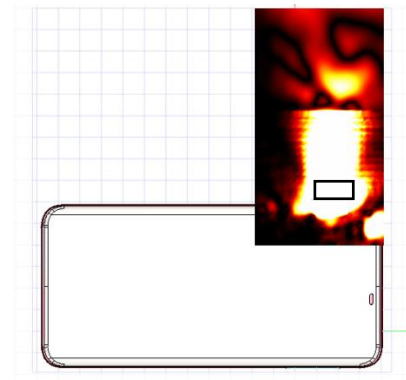
(b) Simulation(0mm)
