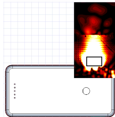
(b) Simulation(0mm)
