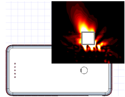
(b) Simulation(0mm)
