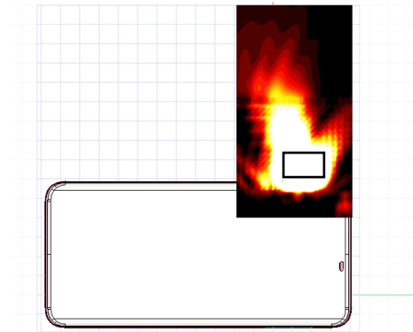
(b) Simulation(0mm)
