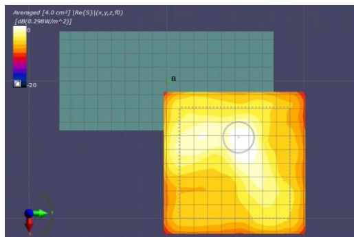
(a) Measurement(2mm)
