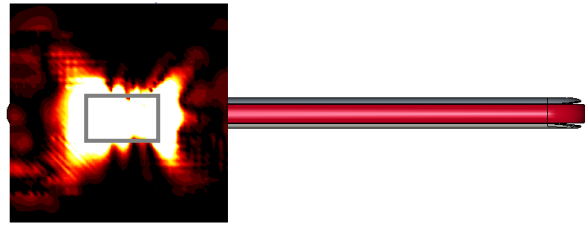
(b) Simulation(0mm)
