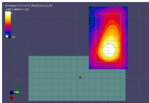
(a) Measurement(2mm)
