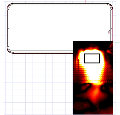
(b) Simulation(0mm)
