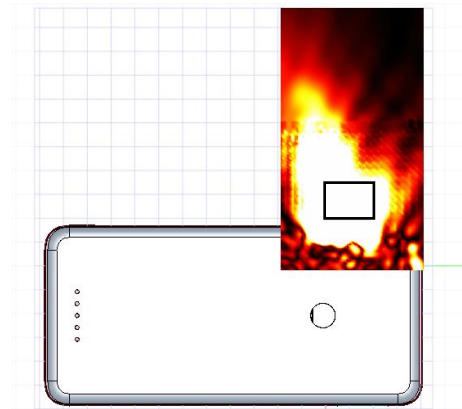
(b) Simulation(0mm)
