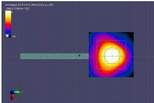
(a) Measurement(2mm)
