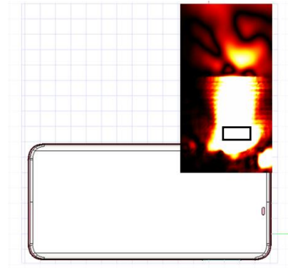
(b) Simulation(0mm)
