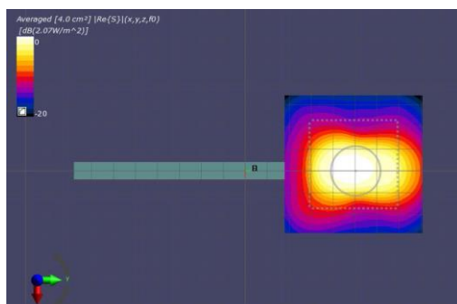
(a) Measurement(2mm)
