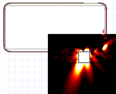
(b) Simulation(0mm)
