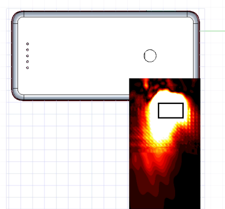
(b) Simulation(0mm)
