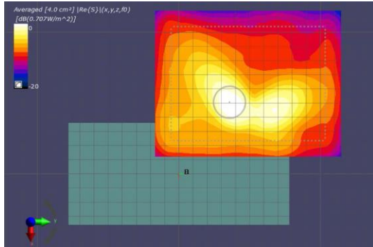
(a) Measurement(2mm)
