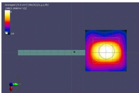
(a) Measurement(2mm)
