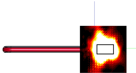
(b) Simulation(0mm)
