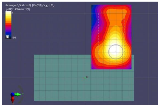
(a) Measurement(2mm)
