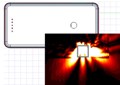
(b) Simulation(0mm)
