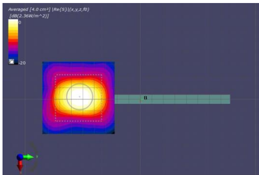
(a) Measurement(2mm)
