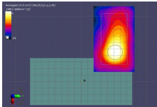
(a) Measurement(2mm)
