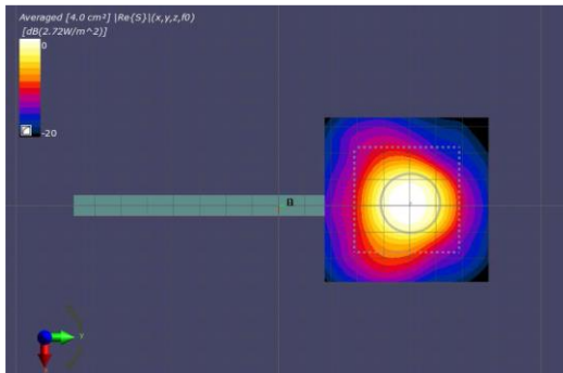
(a) Measurement(2mm)
