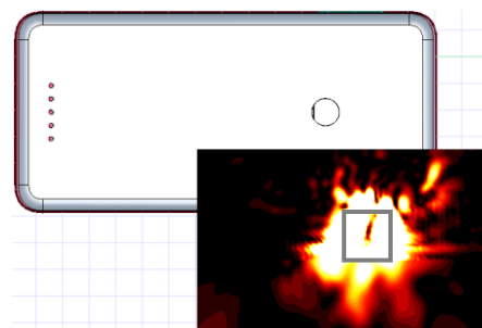
(b) Simulation(0mm)
