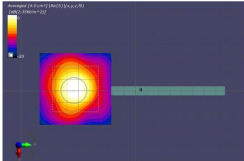
(a) Measurement(2mm)
