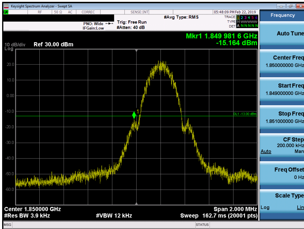
Plot 7-45. Band Edge Plot (PCS GPRS Mode - Low Channel)
