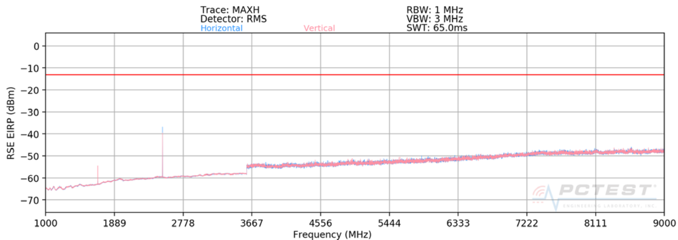
Plot 7-58. Radiated Spurious Emission Plot >1GHz (Cellular GPRS Mode)
