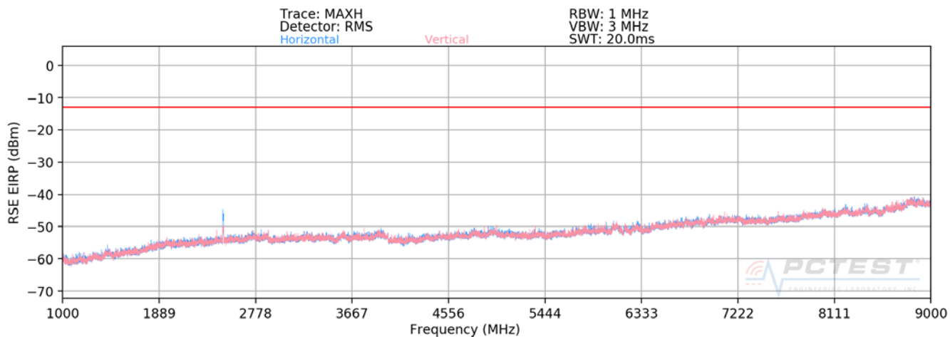
Plot 7-59. Radiated Spurious Emission Plot >1GHz (Cellular WCDMA Mode)
