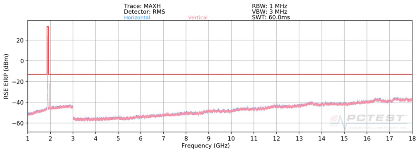
Plot 7-61. Radiated Spurious Emission Plot >1GHz (PCS WCDMA Mode)
