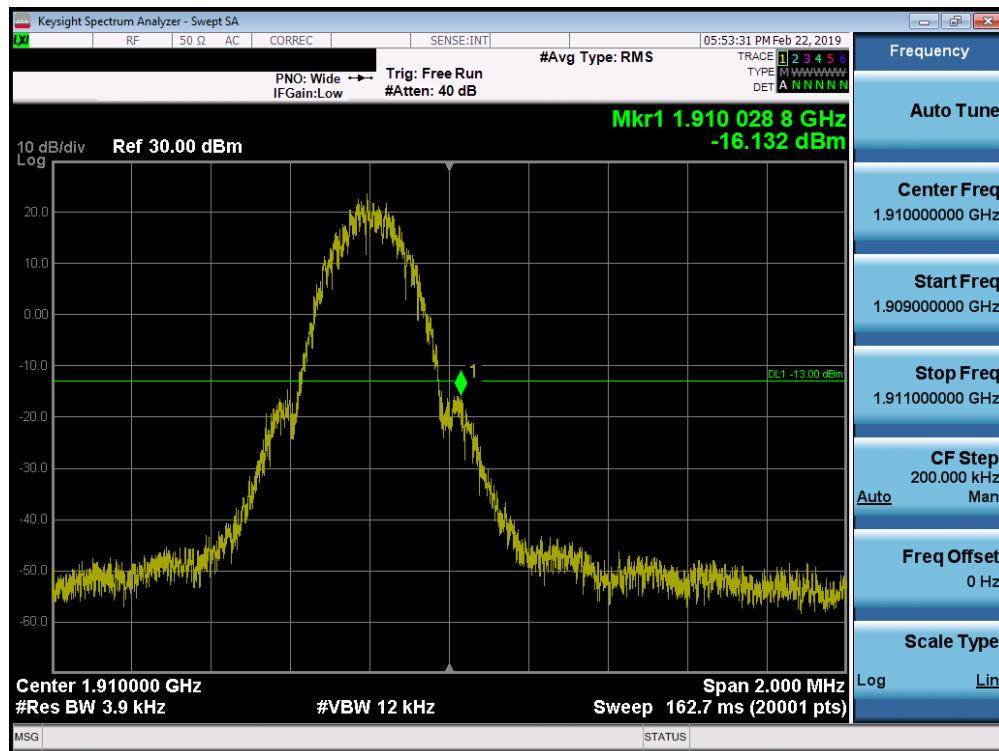
Plot 7-47. Band Edge Plot (PCS GPRS Mode - High Channel)
