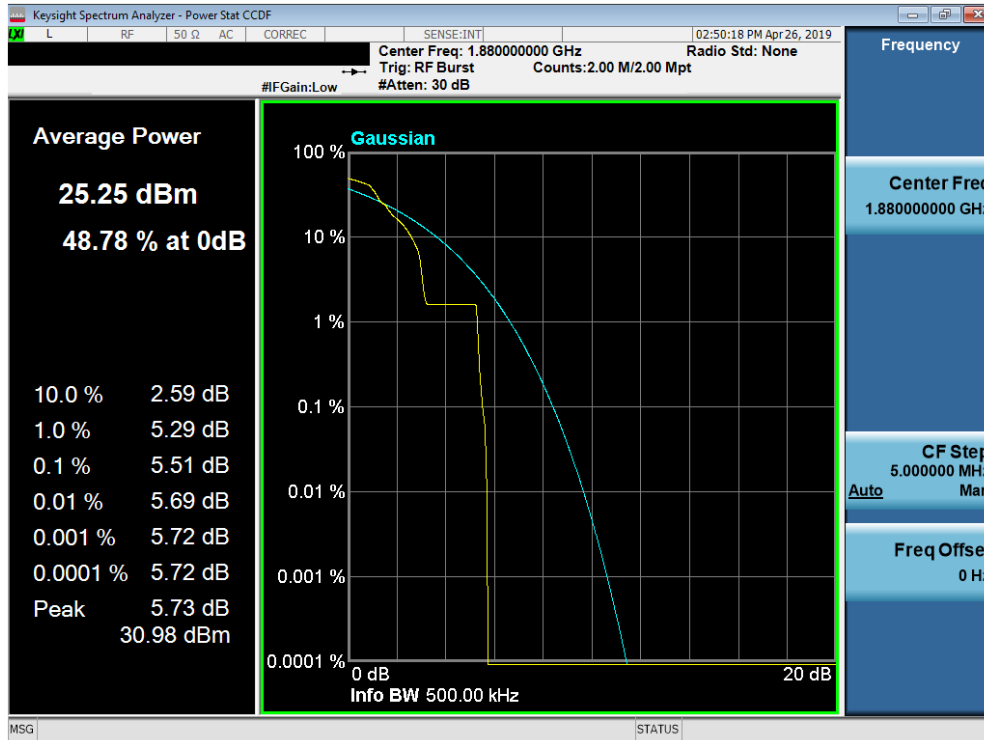
Plot 7-56. Peak-Average Ratio Plot (EDGE PCS GPRS Mode)
