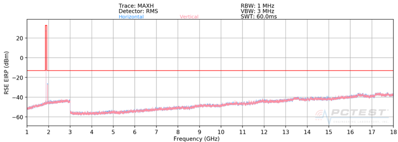
Plot 7-60. Radiated Spurious Emission Plot >1GHz (PCS GPRS Mode)
