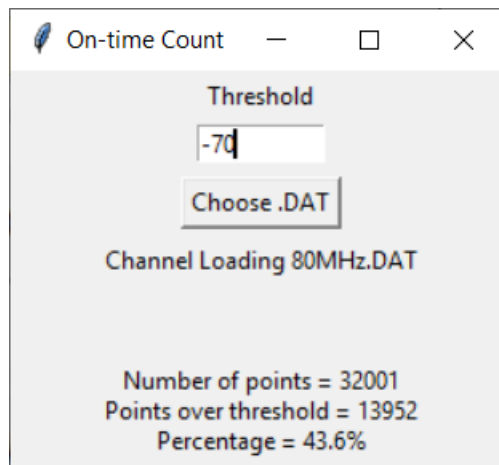
Figure 5-2. Band 2C Channel Loading Calculation
