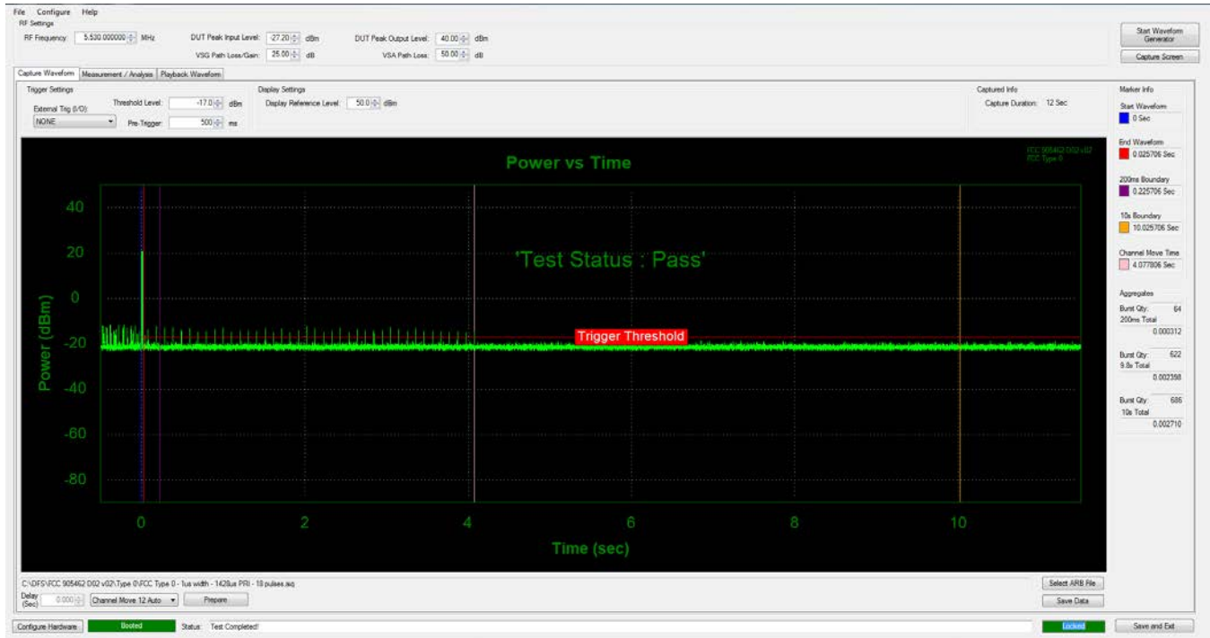
Figure 5-3. Band 2C Move Time and Aggregate Time
