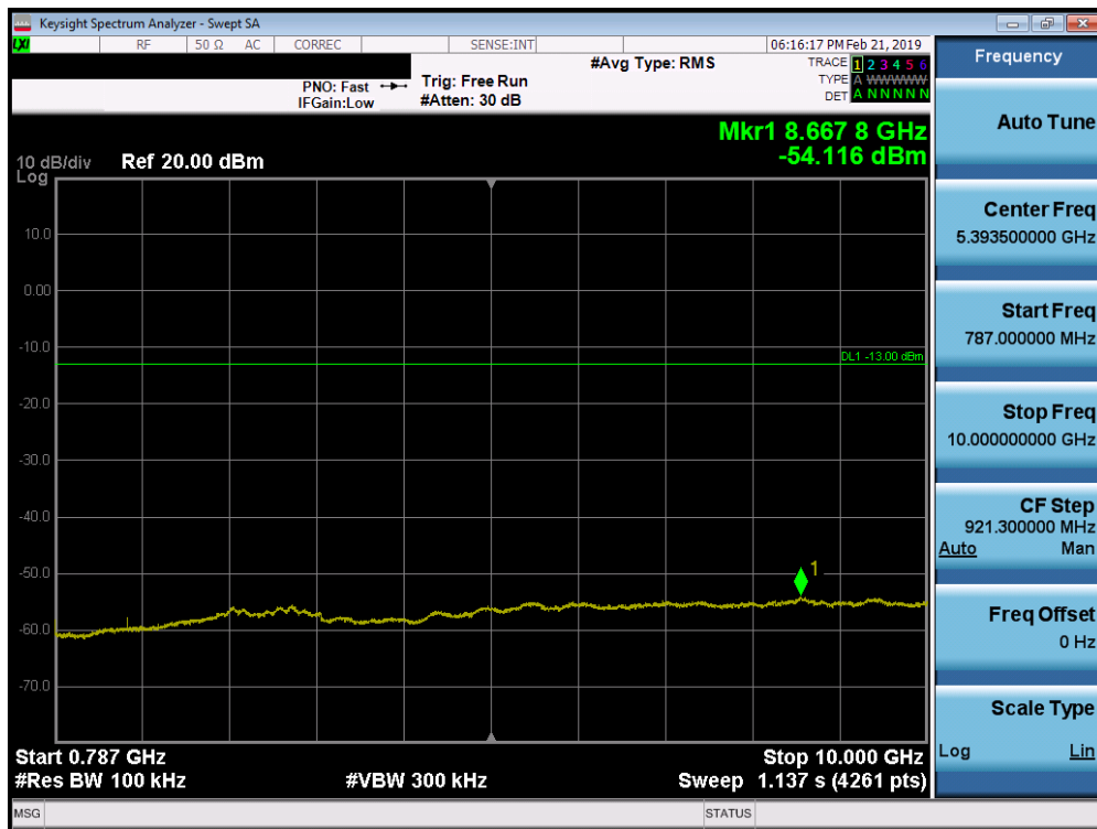
Plot 7-56. Conducted Spurious Plot (Band 13 - 10.0MHz QPSK - RB Size 1, RB Offset 0 - Mid Channel)
