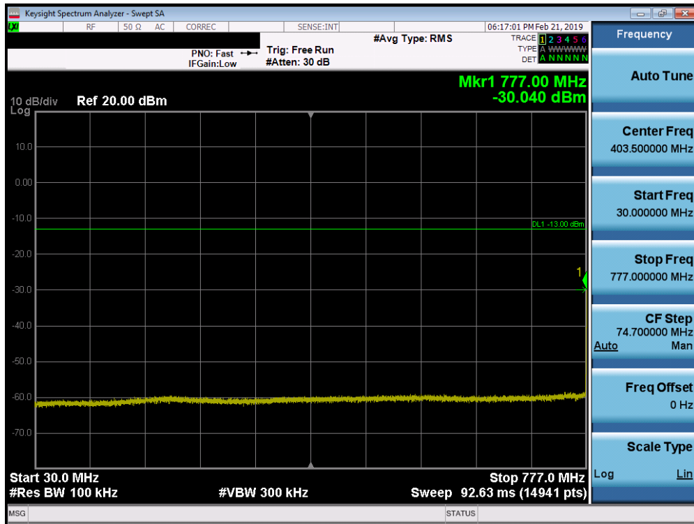
Plot 7-55. Conducted Spurious Plot (Band 13 - 10.0MHz QPSK - RB Size 1, RB Offset 0 - Mid Channel)
