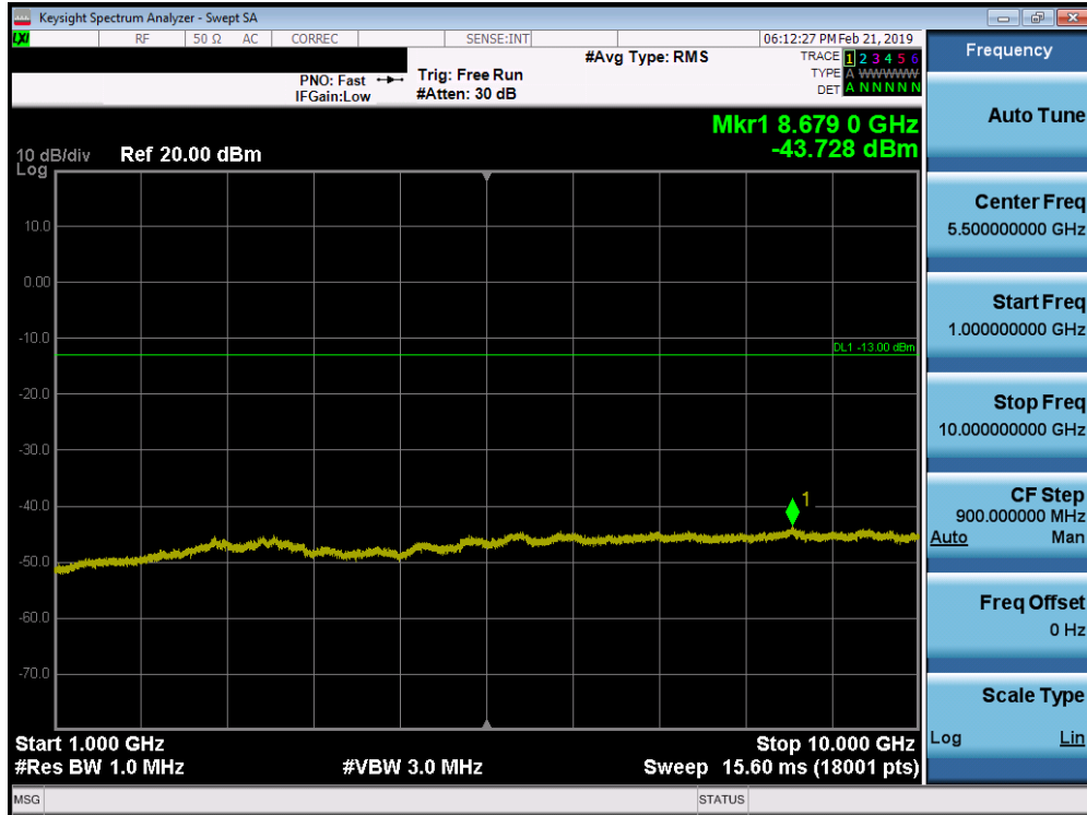
Plot 7-57. Conducted Spurious Plot (Band 13 - 10.0MHz QPSK - RB Size 1, RB Offset 0 - Mid Channel)
