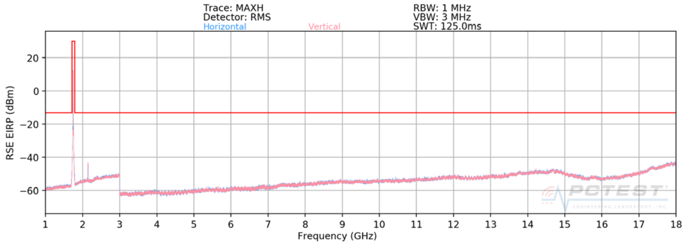
Plot 7-3. Radiated Spurious Plot above 1GHz (Band 66/4)
