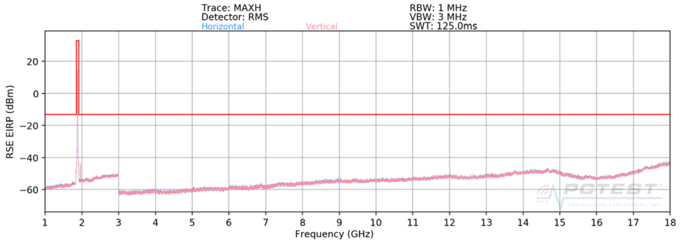
Plot 7-4. Radiated Spurious Plot above 1GHz (Band 2)
