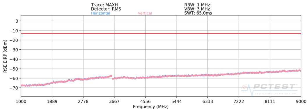
Plot 7-2. Radiated Spurious Plot above 1GHz (Band 5)
