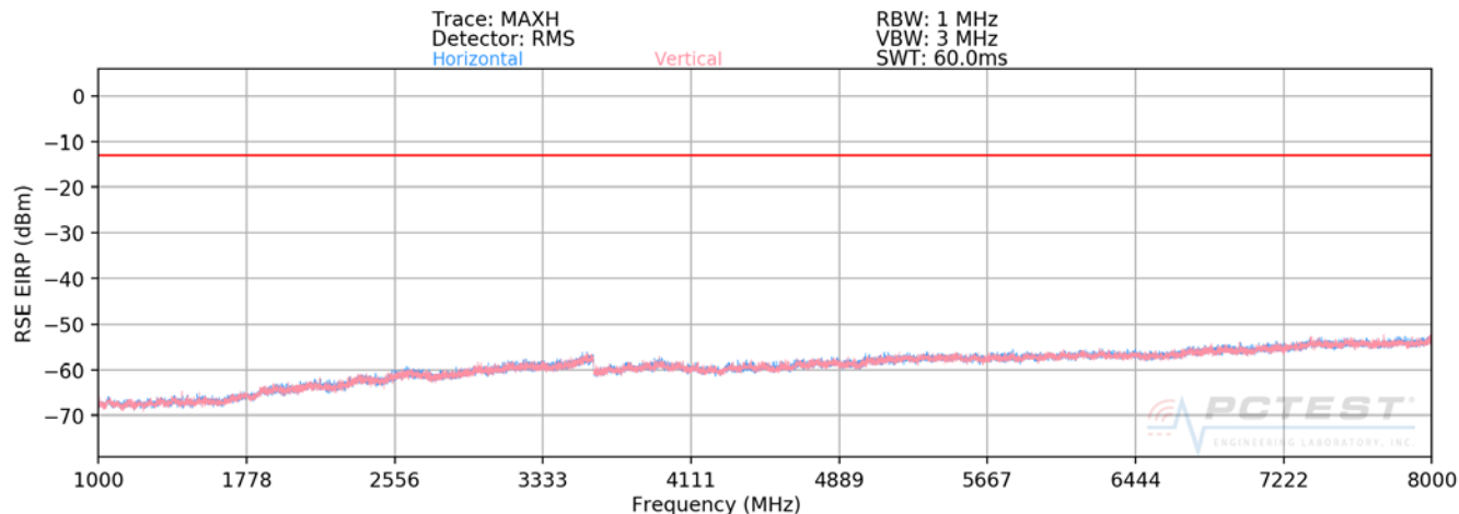
Plot 7-1. Radiated Spurious Plot above 1GHz (Band 13)
