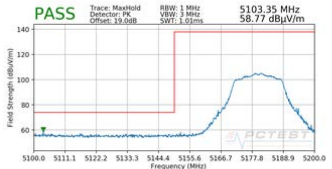
Plot 7-200. Radiated Lower Band Edge Plot SISO ANT2 (Peak – UNII Band 1)
