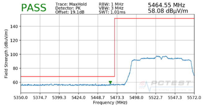
Plot 7-110. Radiated Lower Band Edge Plot MIMO (Peak – UNII Band 2C)
