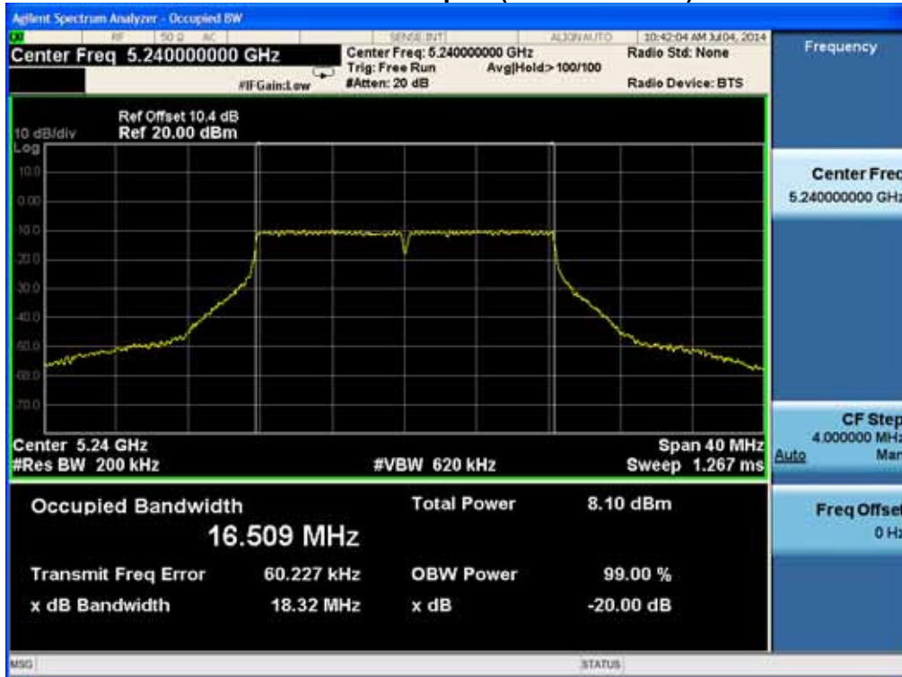
20 dB Bandwidth plot (802.11a-CH 48)
