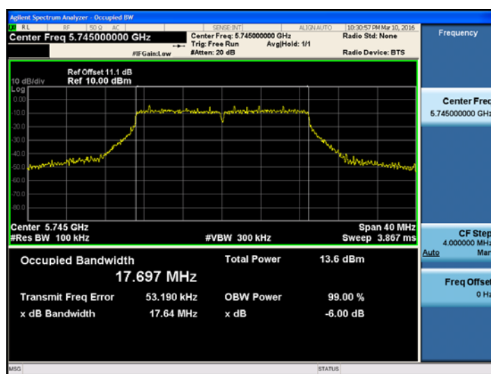
802.11n_20 MHz BW UNII 3 BAND 6dB Bandwidth(CH.149)
