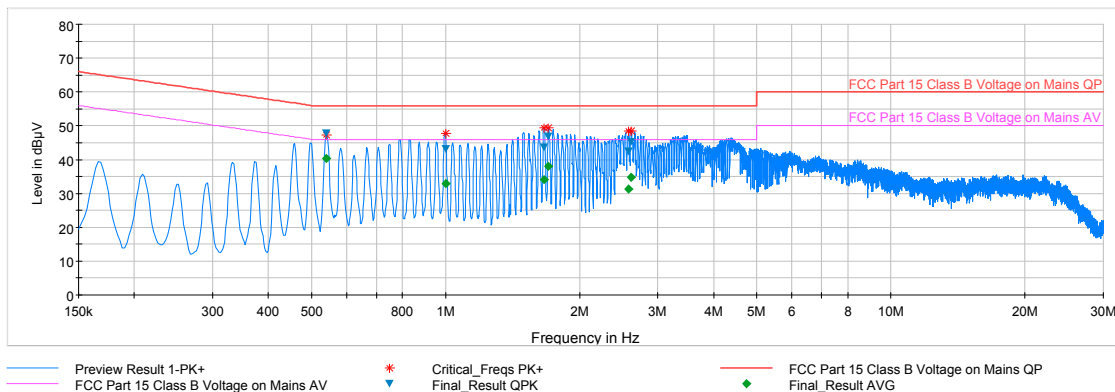
Plot 6-31. Line Conducted Plot with Bluetooth LE (N)
