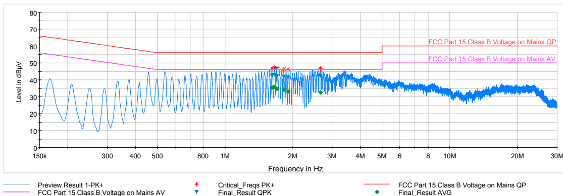
Plot 6-30. Line Conducted Plot with Bluetooth LE (L1)
