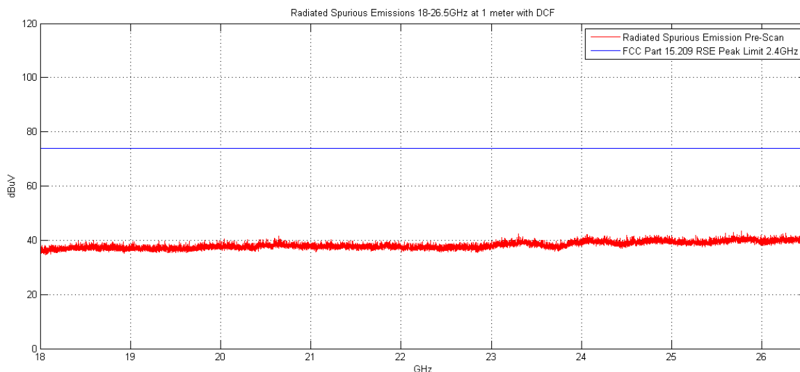
Plot 6-24. Radiated Spurious Plot above 18GHz (Pol. H)
