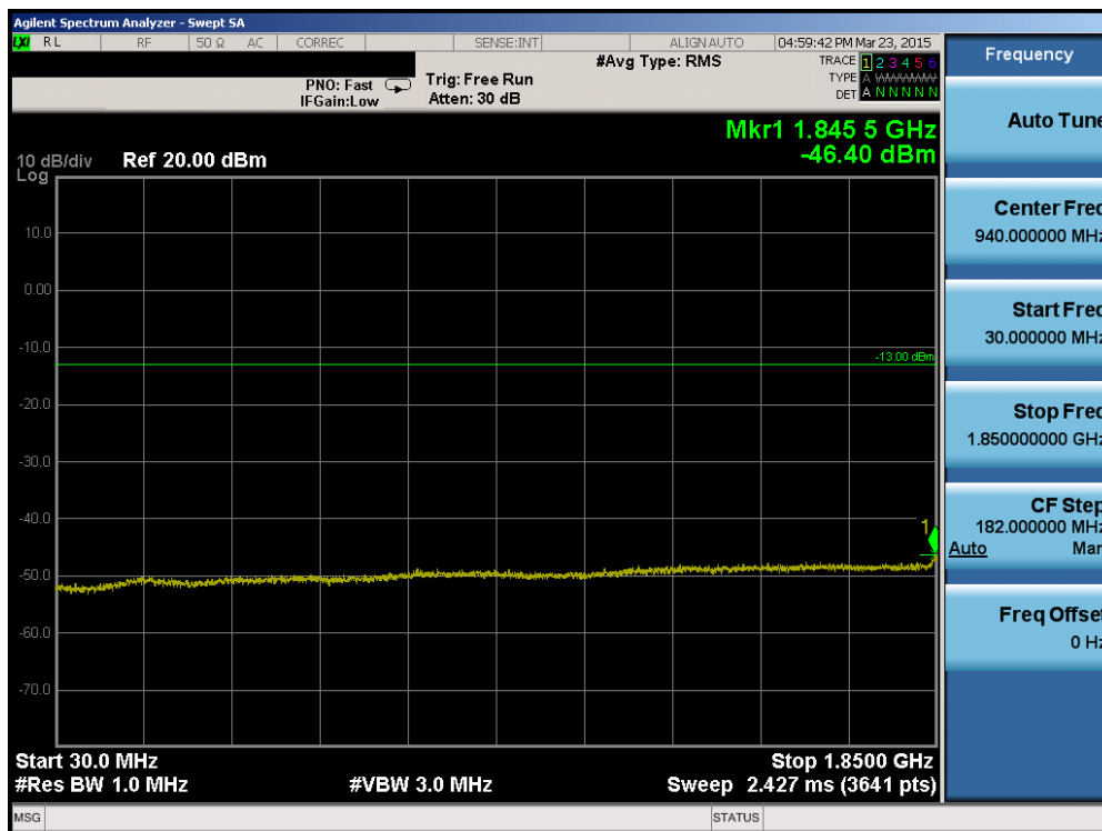
Plot 6-82. Conducted Spurious Plot (Band 2 – 20.0MHz QPSK – RB Size 1, RB Offset 0 – High Channel)
