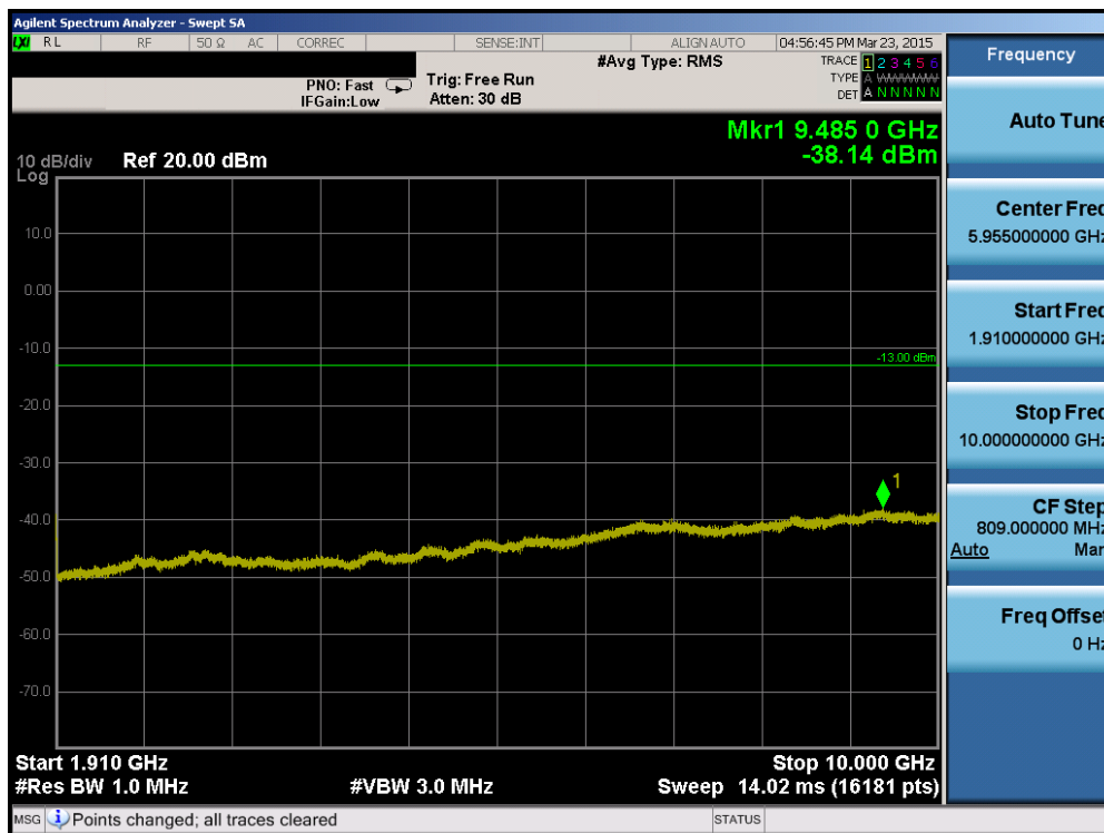
Plot 6-80. Conducted Spurious Plot (Band 2 – 20.0MHz QPSK – RB Size 1, RB Offset 0 – Mid Channel)
