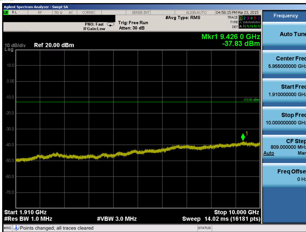
Plot 6-77. Conducted Spurious Plot (Band 2 – 20.0MHz QPSK – RB Size 1, RB Offset 0 – Low Channel)
