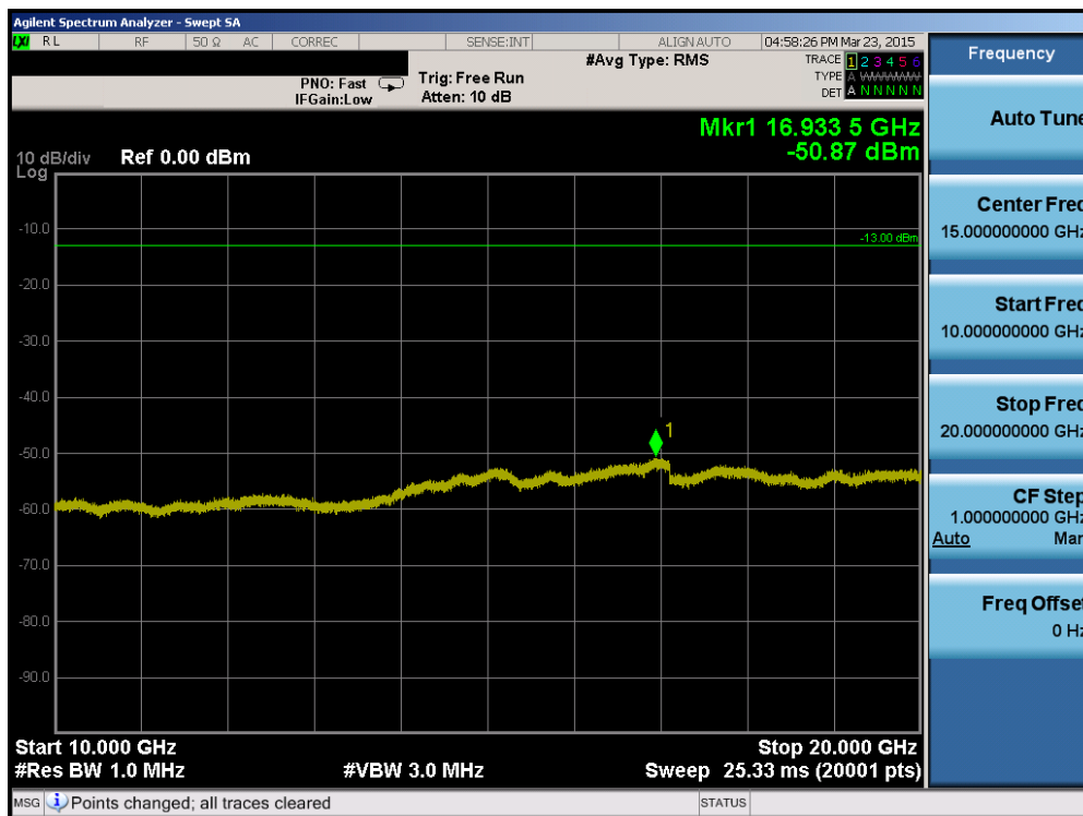
Plot 6-78. Conducted Spurious Plot (Band 2 – 20.0MHz QPSK – RB Size 1, RB Offset 0 – Low Channel)
