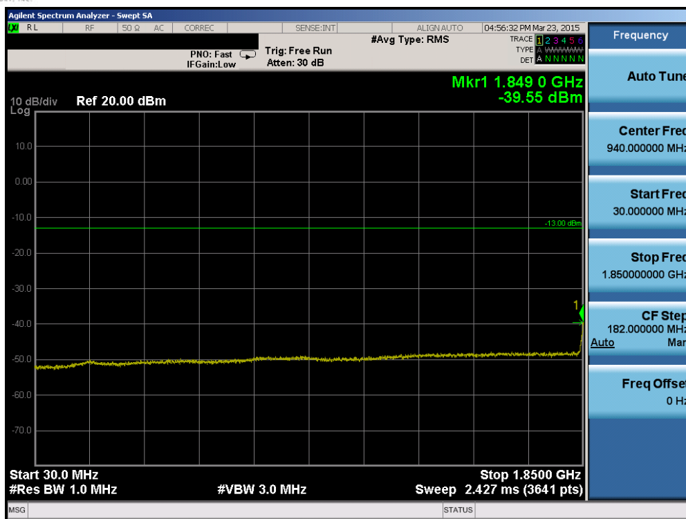
Plot 6-79. Conducted Spurious Plot (Band 2 – 20.0MHz QPSK – RB Size 1, RB Offset 0 – Mid Channel)
