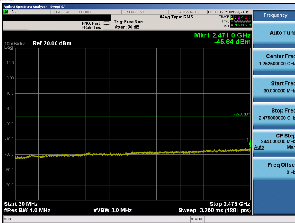
Plot 6-85. Conducted Spurious Plot (Band 7 – 20.0MHz QPSK – RB Size 1, RB Offset 0– Low Channel)
