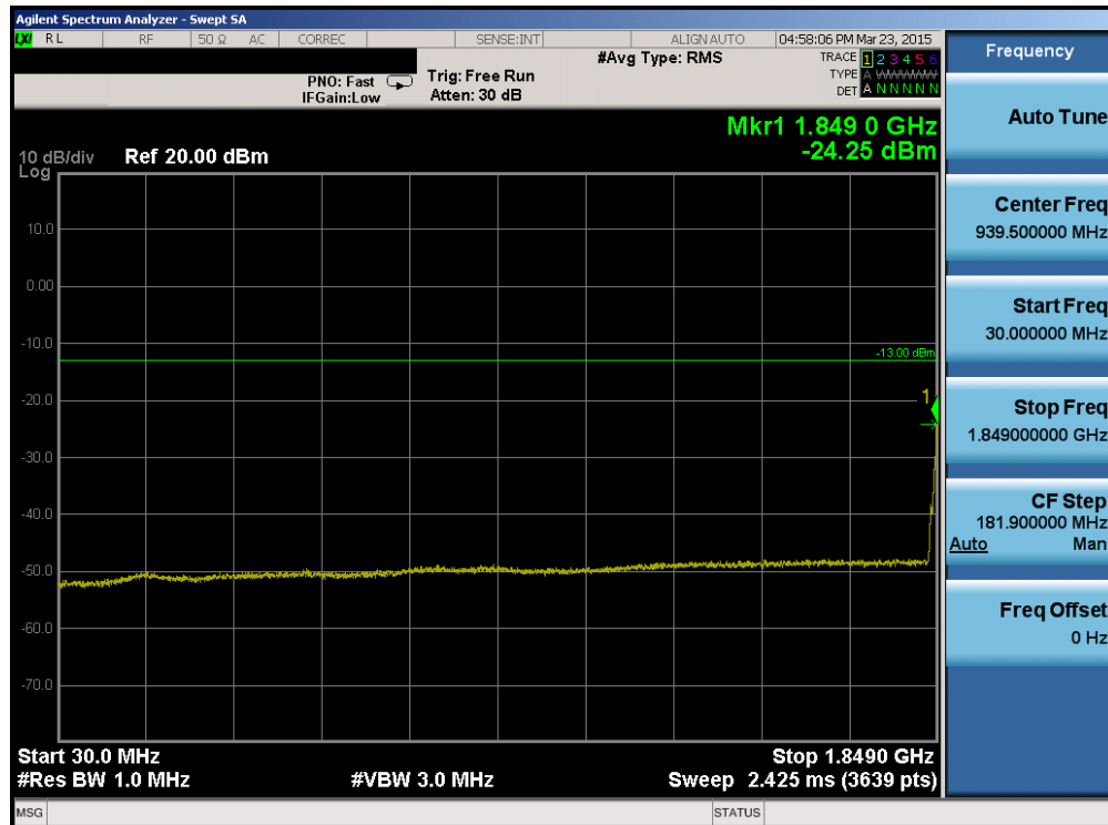
Plot 6-76. Conducted Spurious Plot (Band 2 – 20.0MHz QPSK – RB Size 1, RB Offset 0– Low Channel)
