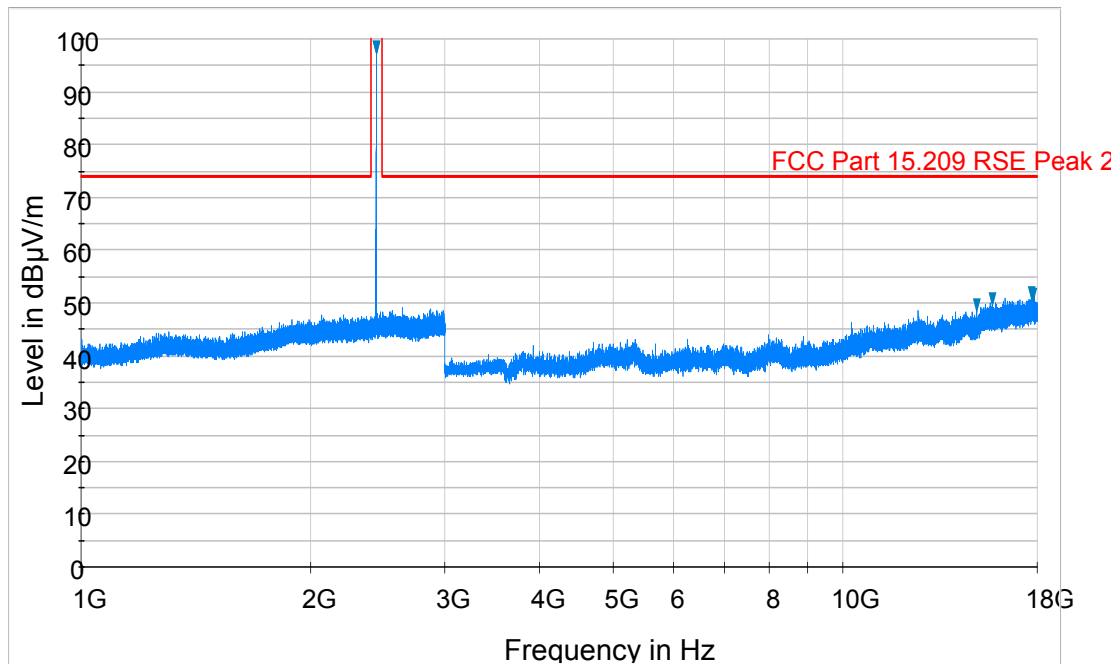
Plot 6-44. Radiated Spurious Plot above 1GHz (BT – Ch. 39, Ant. Pol. H)
