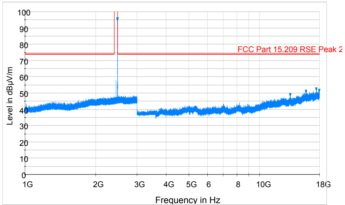
Plot 6-47. Radiated Spurious Plot above 1GHz (BT – Ch. 78, Ant. Pol. V)
