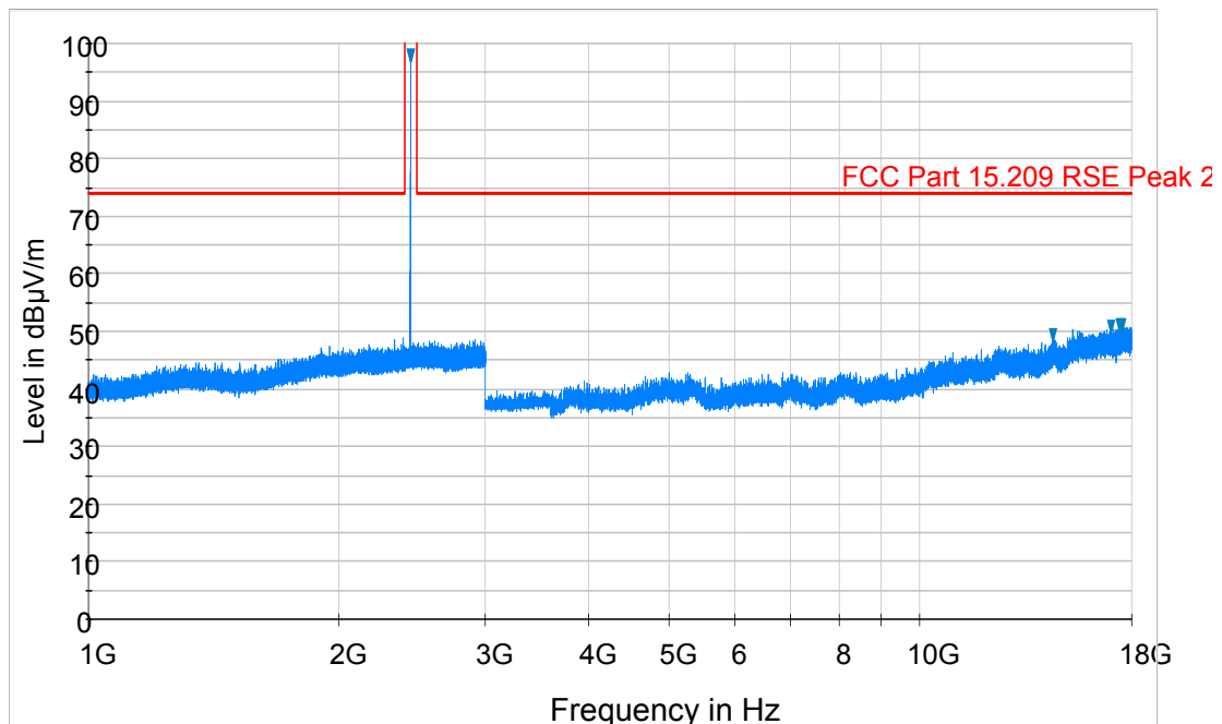
Plot 6-45. Radiated Spurious Plot above 1GHz (BT – Ch. 39, Ant. Pol. V)
