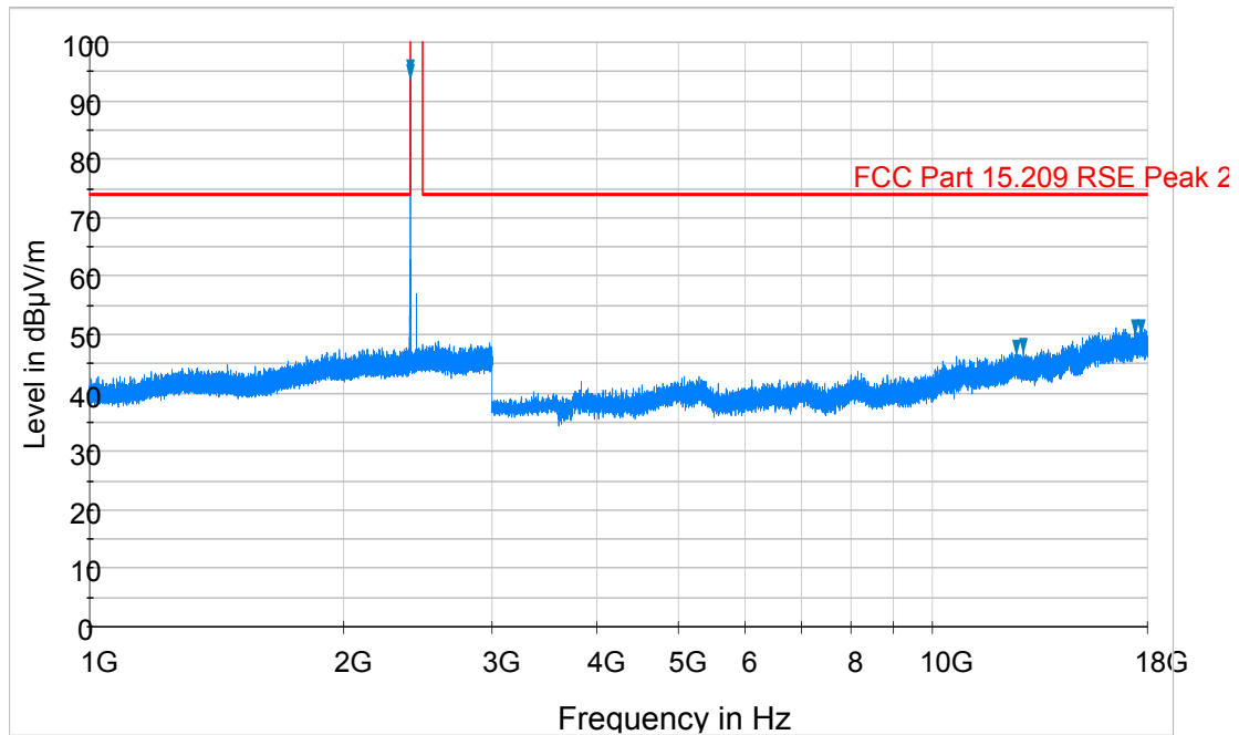
Plot 6-43. Radiated Spurious Plot above 1GHz (BT – Ch. 0, Ant. Pol. V)
