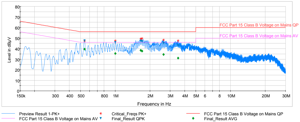
Plot 6-55. Line-Conducted Test Plot (N)
