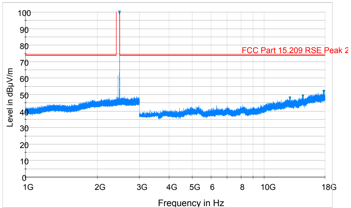
Plot 6-46. Radiated Spurious Plot above 1GHz (BT – Ch. 78, Ant. Pol. H)
