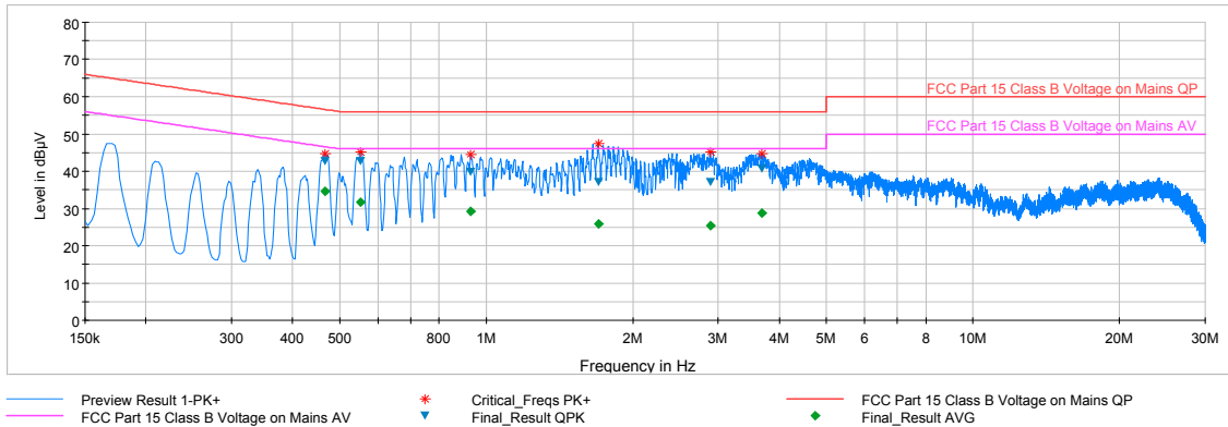
Plot 6-54. Line-Conducted Test Plot (L1)
