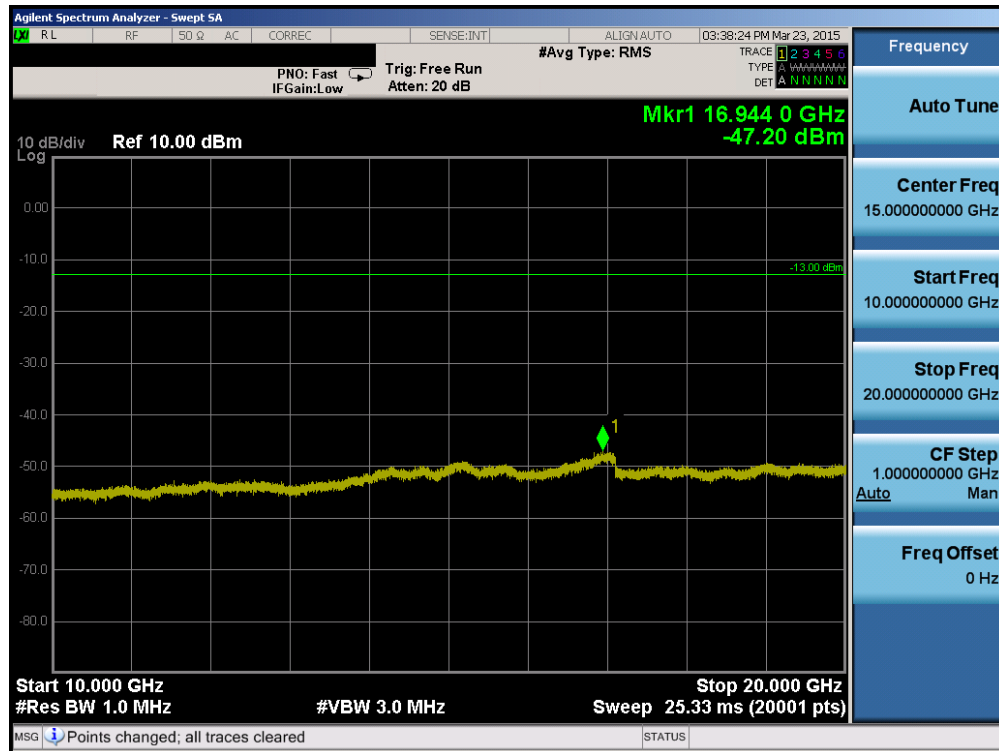
Plot 6-15. Conducted Spurious Plot (AWS WCDMA Mode – Ch. 1312)
