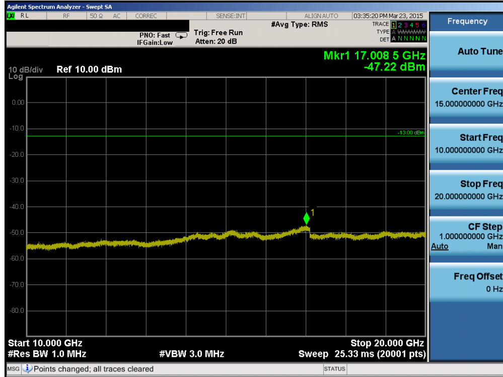
Plot 6-30. Conducted Spurious Plot (PCS WCDMA Mode – Ch. 9538)
