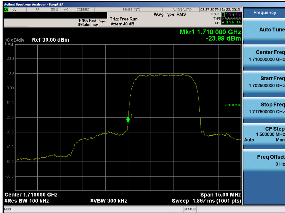
Plot 6-33. Band Edge Plot (AWS WCDMA Mode – Ch. 1312)
