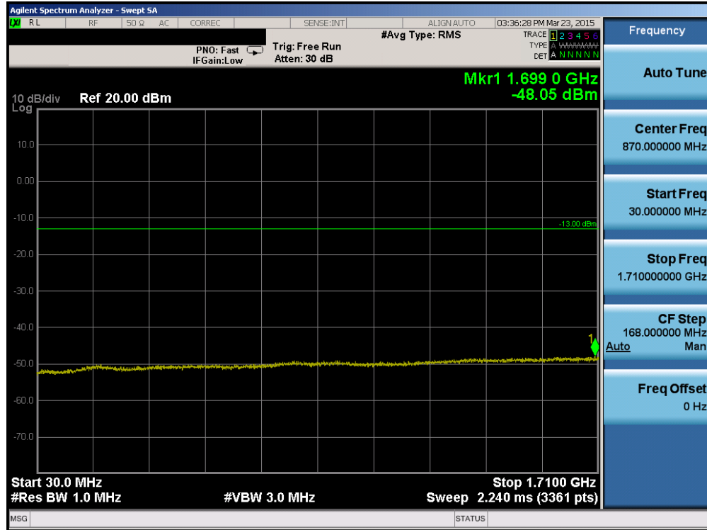
Plot 6-16. Conducted Spurious Plot (AWS WCDMA Mode – Ch. 1412)
