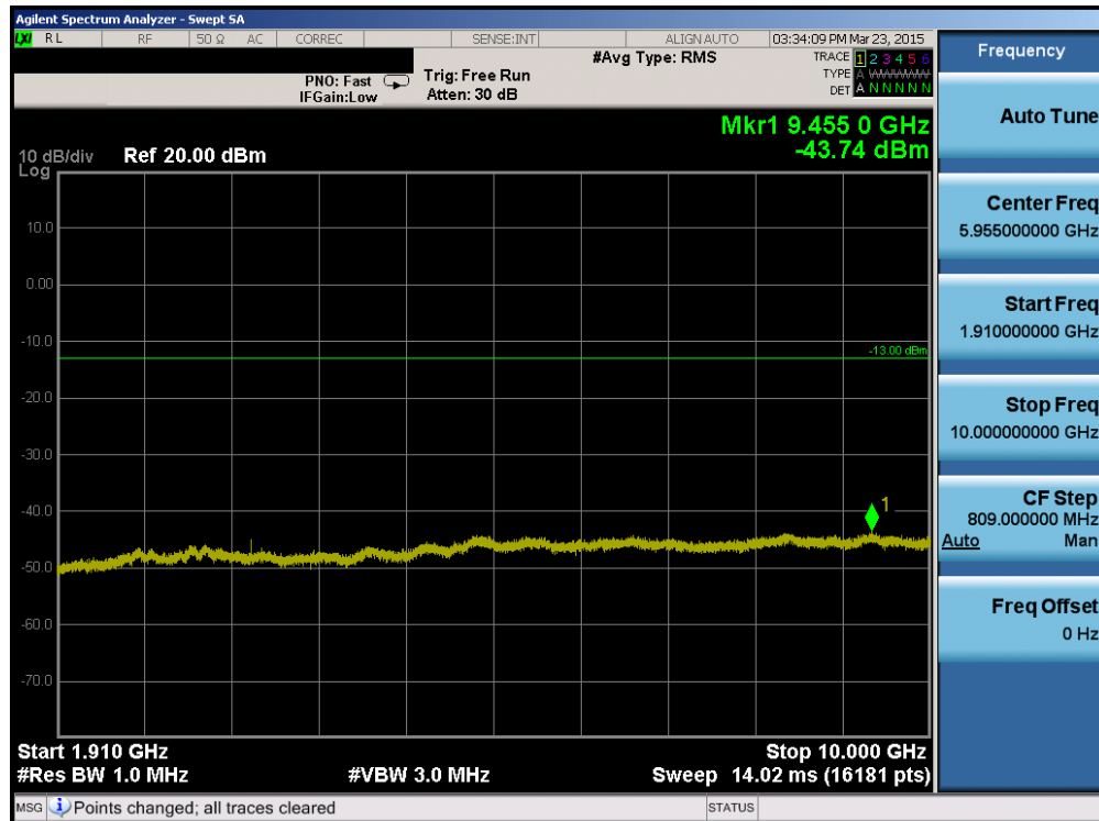
Plot 6-23. Conducted Spurious Plot (PCS WCDMA Mode – Ch. 9262)
