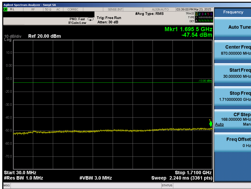
Plot 6-19. Conducted Spurious Plot (AWS WCDMA Mode – Ch. 1862)
