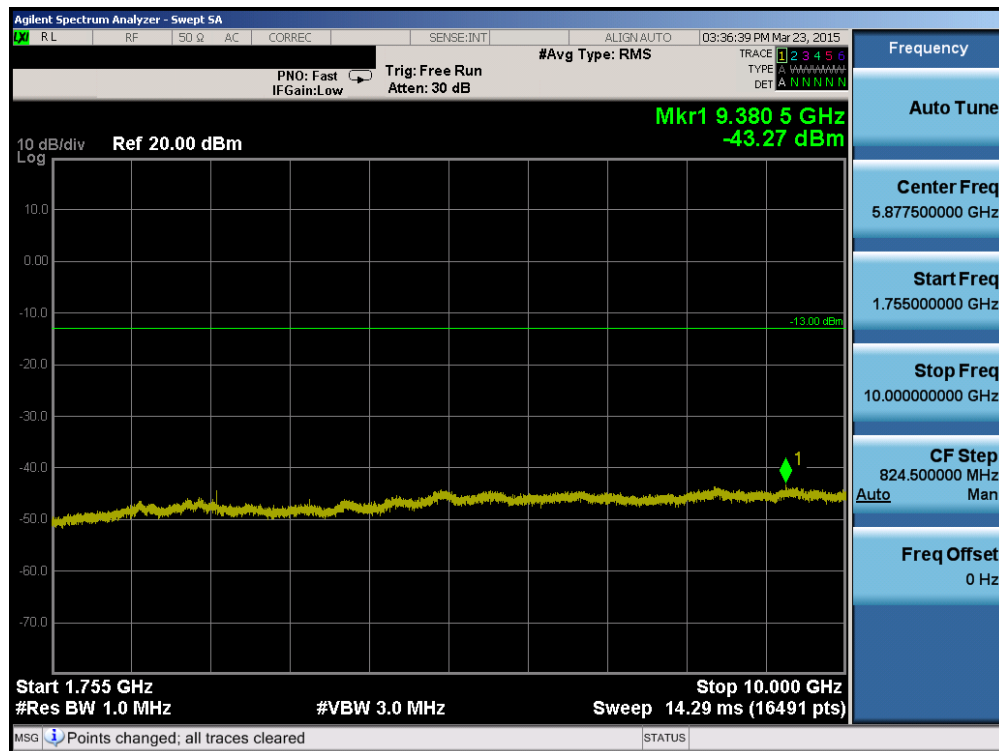
Plot 6-17. Conducted Spurious Plot (AWS WCDMA Mode – Ch. 1412)
