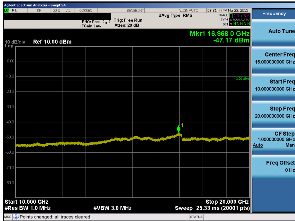
Plot 6-27. Conducted Spurious Plot (PCS WCDMA Mode – Ch. 9400)
