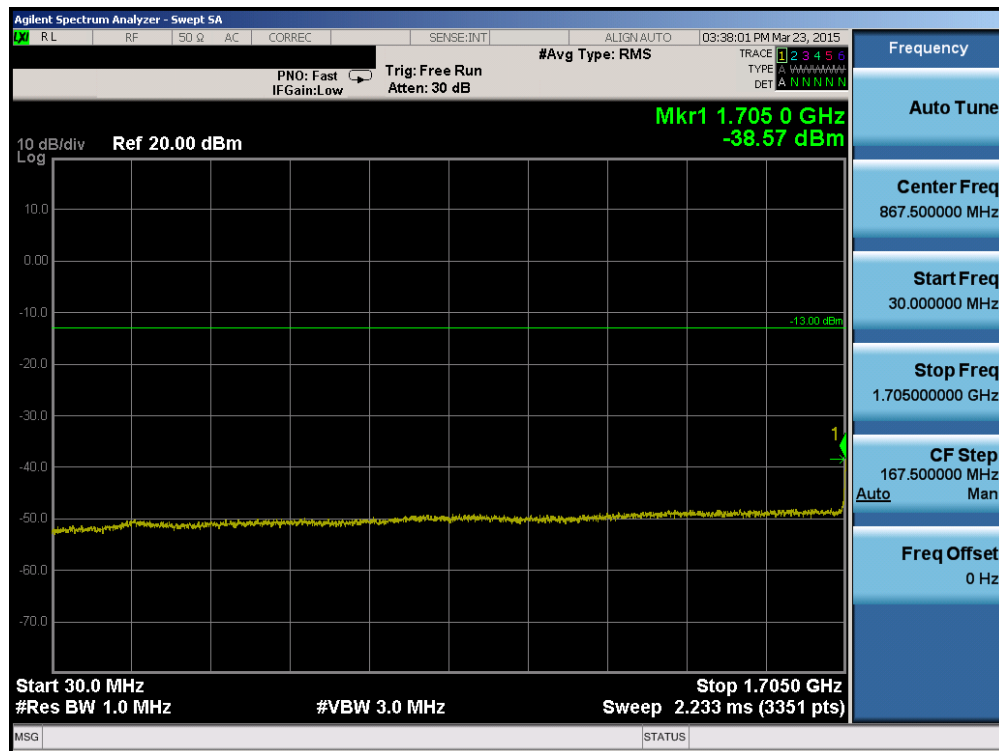
Plot 6-13. Conducted Spurious Plot (AWS WCDMA Mode – Ch. 1312)
