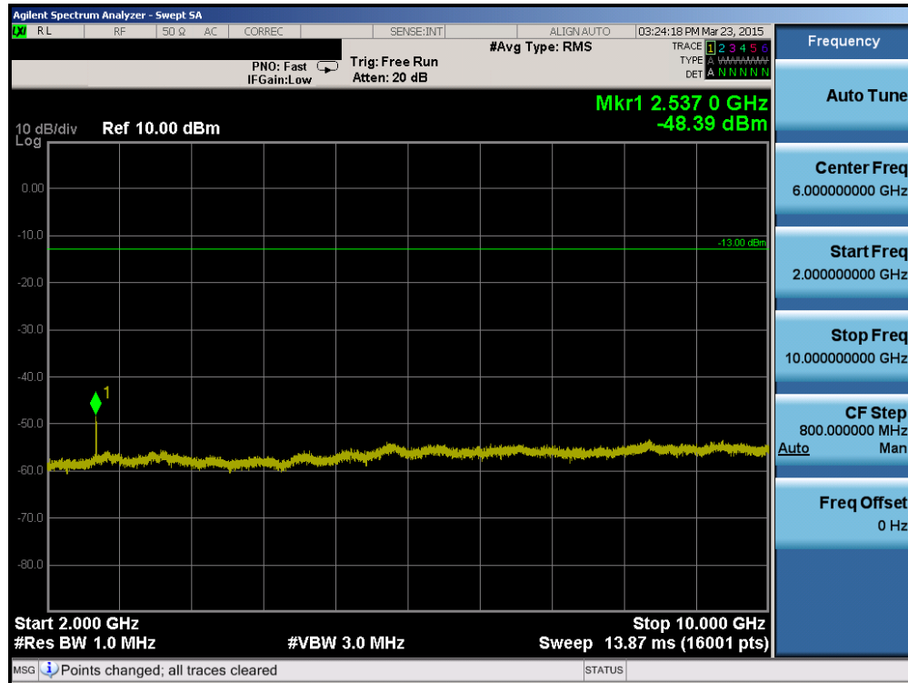
Plot 6-12. Conducted Spurious Plot (Cellular WCDMA Mode – Ch. 4233)
