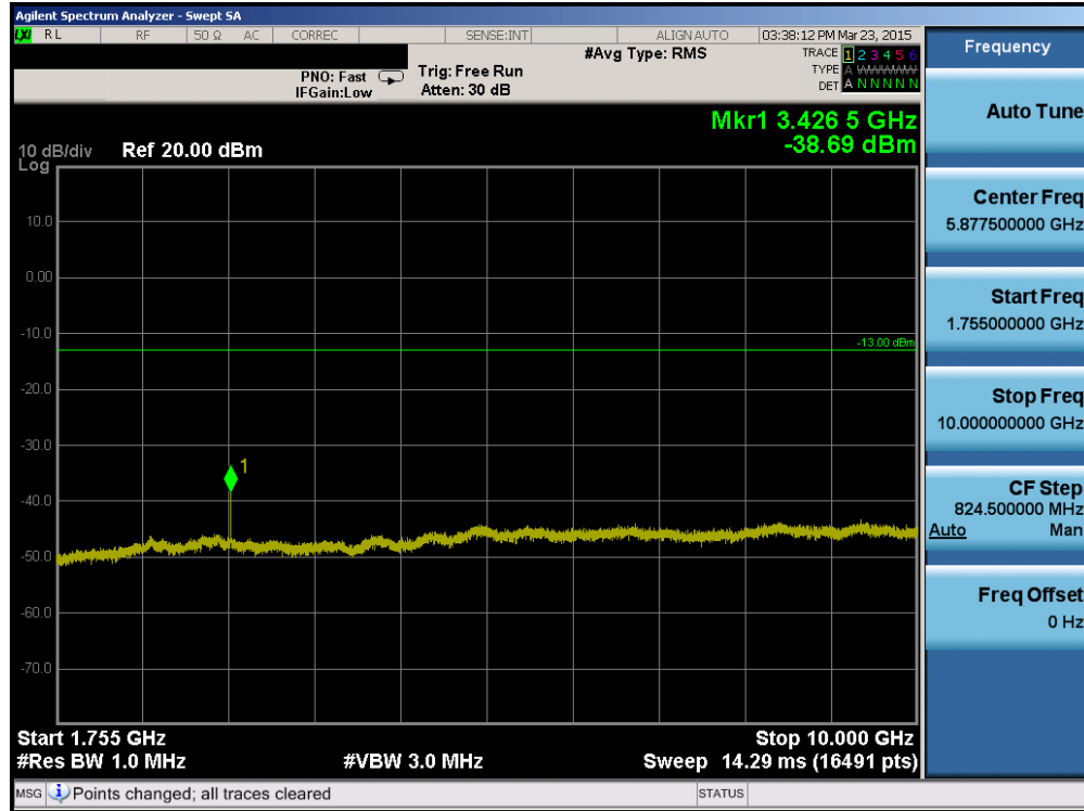
Plot 6-14. Conducted Spurious Plot (AWS WCDMA Mode – Ch. 1312)
