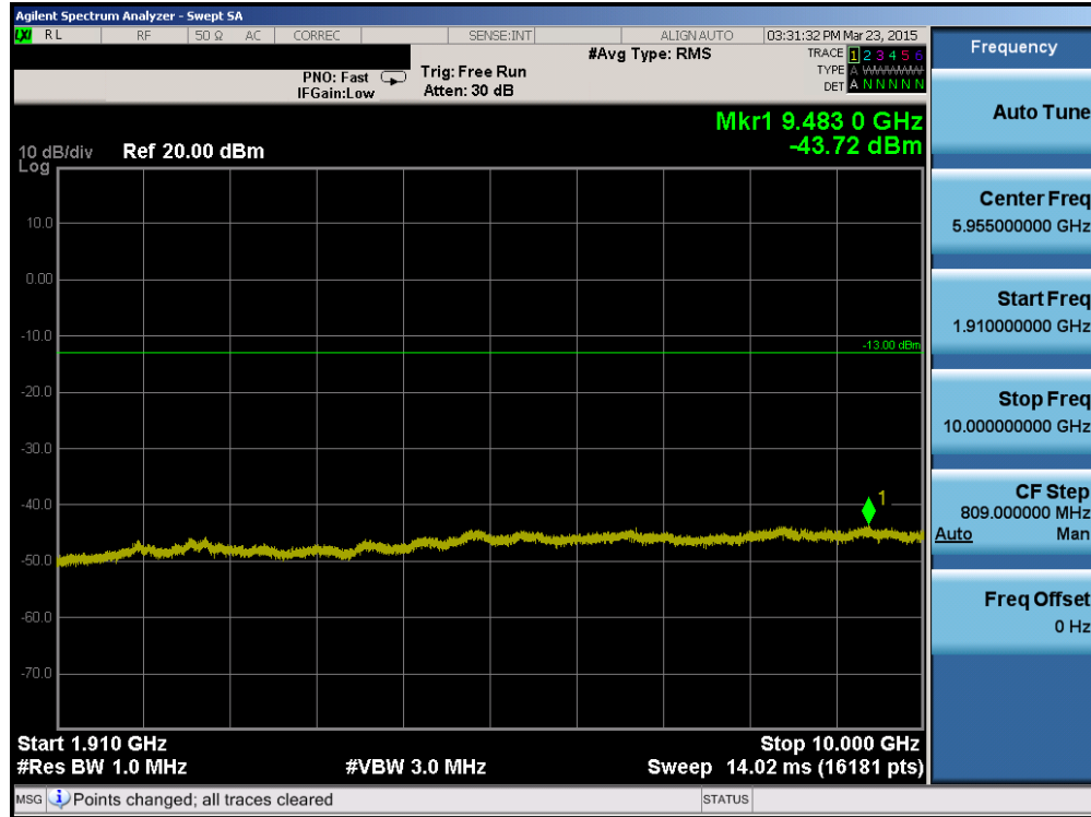
Plot 6-26. Conducted Spurious Plot (PCS WCDMA Mode – Ch. 9400)
