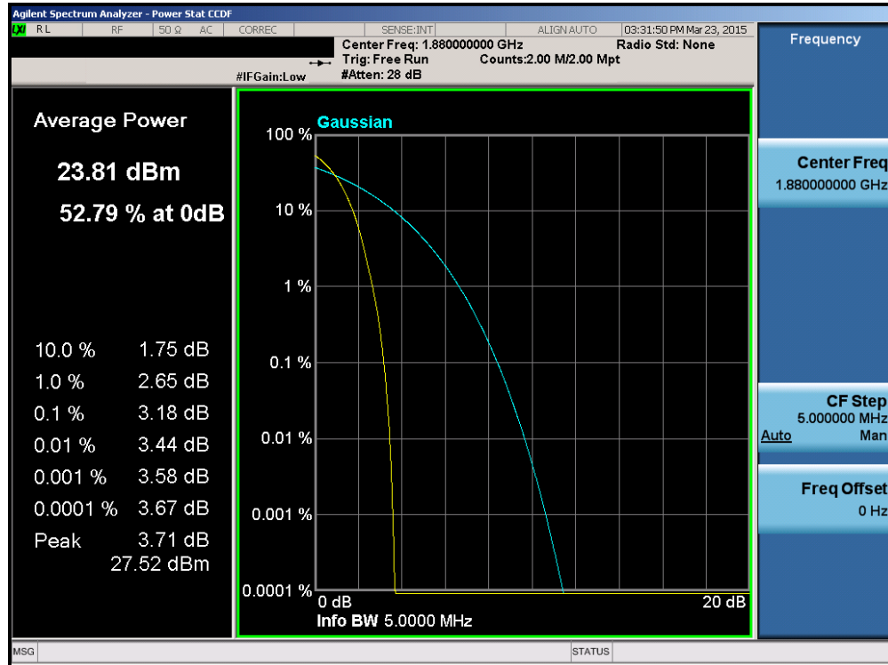
Plot 6-41. Peak-Average Ratio Plot (PCS WCDMA Mode – Ch. 9400)
