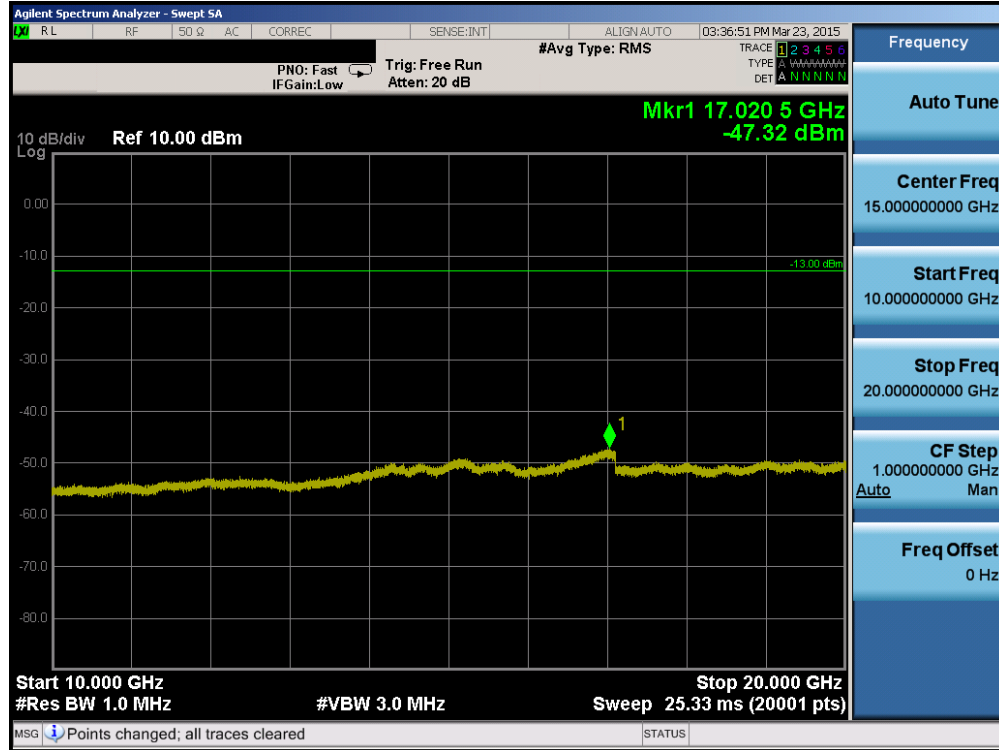
Plot 6-18. Conducted Spurious Plot (AWS WCDMA Mode – Ch. 1412)
