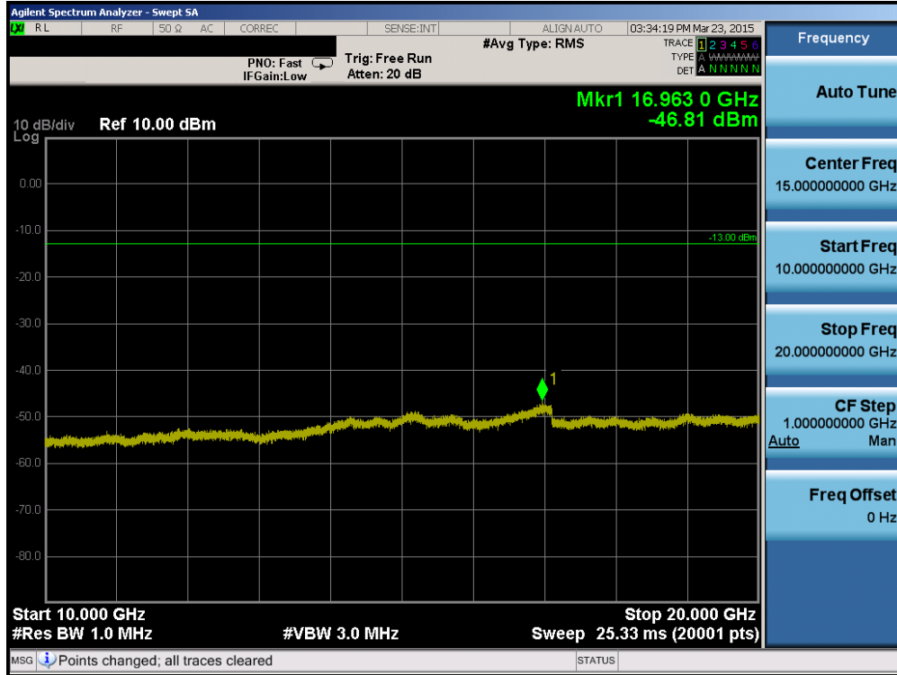
Plot 6-24. Conducted Spurious Plot (PCS WCDMA Mode – Ch. 9262)
