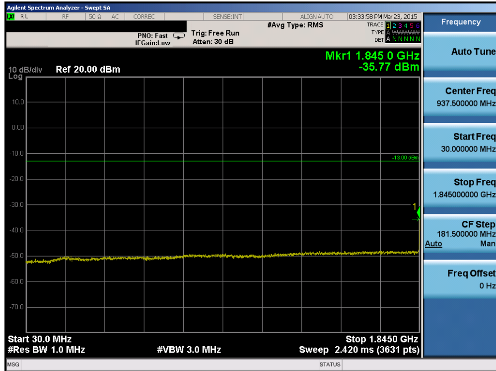
Plot 6-22. Conducted Spurious Plot (PCS WCDMA Mode – Ch. 9262)
