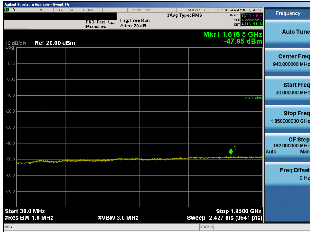
Plot 6-28. Conducted Spurious Plot (PCS WCDMA Mode – Ch. 9538)
