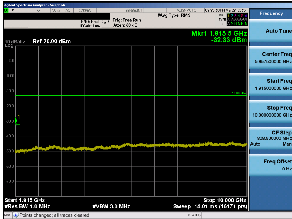
Plot 6-29. Conducted Spurious Plot (PCS WCDMA Mode – Ch. 9538)
