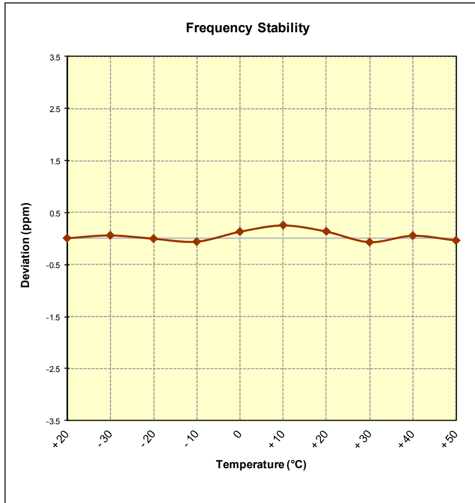
Figure 6-8. Frequency Stability Graph (AWS WCDMA Mode – Ch. 1412)
