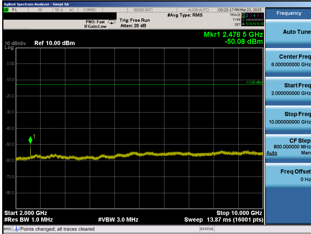
Plot 6-6. Conducted Spurious Plot (Cellular WCDMA Mode – Ch. 4132)
