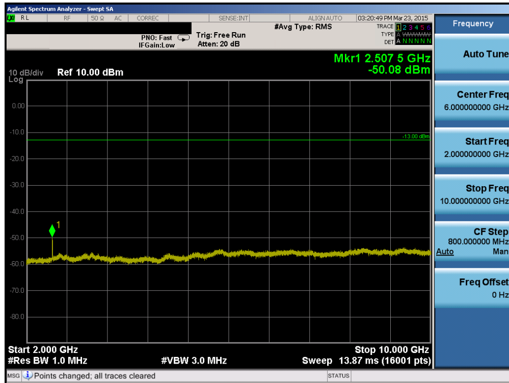
Plot 6-9. Conducted Spurious Plot (Cellular WCDMA Mode – Ch. 4183)
