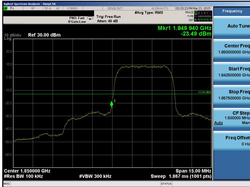
Plot 6-37. Band Edge Plot (PCS WCDMA Mode – Ch. 9262)
