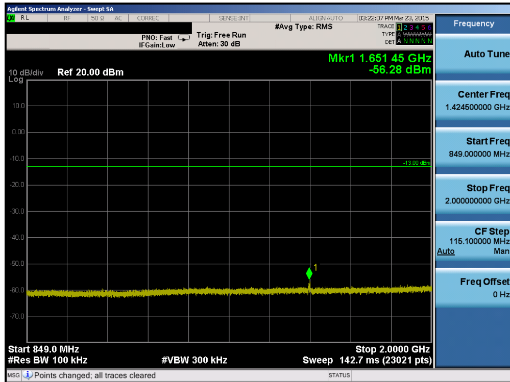
Plot 6-5. Conducted Spurious Plot (Cellular WCDMA Mode – Ch. 4132)
