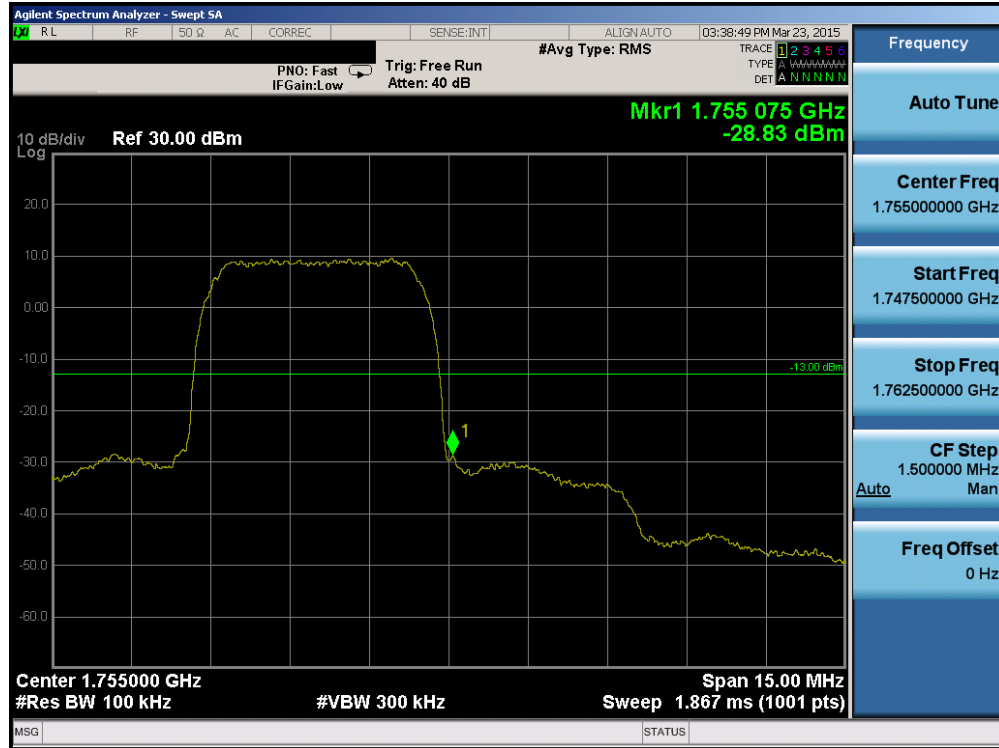
Plot 6-35. Band Edge Plot (AWS WCDMA Mode – Ch. 1862)
