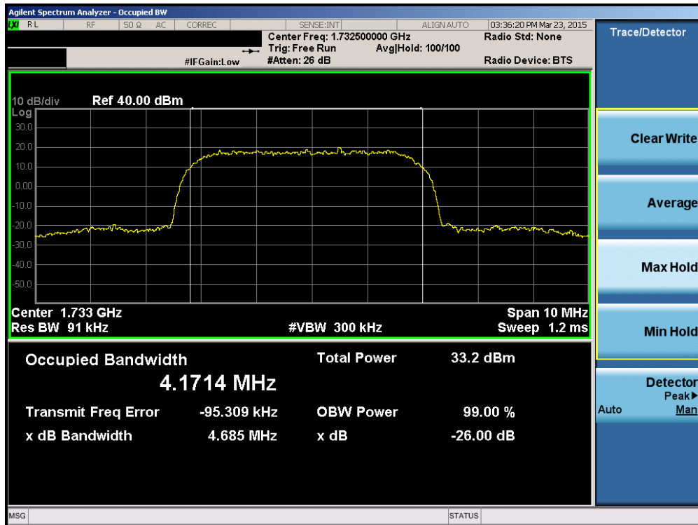
Plot 6-2. Occupied Bandwidth Plot (AWS WCDMA Mode – Ch. 1412)
