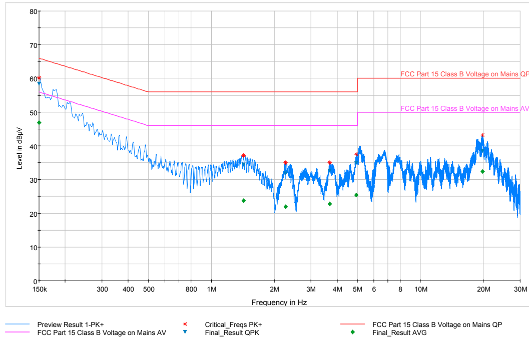
Plot 6-54. Line-Conducted Test Plot (L1)
