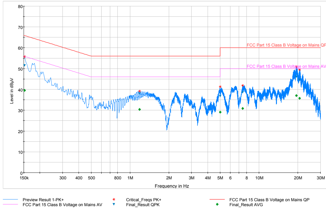
Plot 6-55. Line-Conducted Test Plot (N)
