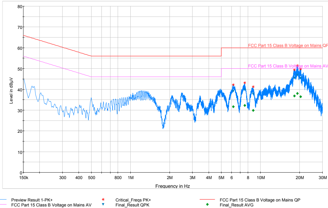
Plot 6-96. Line Conducted Plot with 802.11a UNII Band 2C (N)
