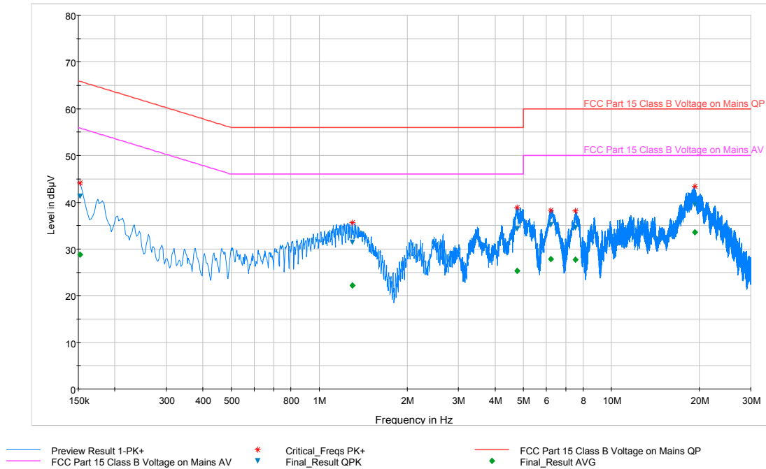
Plot 6-95. Line Conducted Plot with 802.11a UNII Band 2C (L1)
